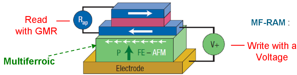
Fig. 9: Concept of multiferroic memory cell [22]. As in the already existing magnetic RAM (MRAM), the information is encoded in the parallel or antiparallel alignment of the magnetization of two layers, read out with the giant magneto-resistance effect. The addition of a layer of magnetoelectrically active (e.g. multiferroic) material allows to write the information by applying a voltage, overcoming the main drawback of MRAM cells.
