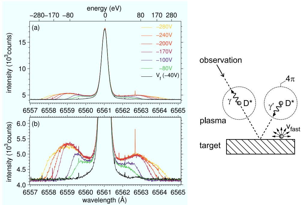
Figure 3: (left) Scan of acceleration potential: Measurement of D_\alpha from the 35° observation. (right) With 35° observation direct light is seen with a blue Doppler shift, reflected emission is seen with a red Doppler shift.
