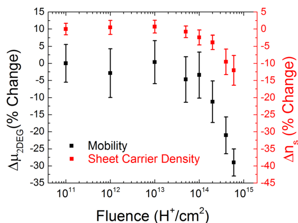
FIG. 5. Hall characteristics as a function of fluence. After a 6 \times 10^{14} \text{ cm}^{-2} dose of proton radiation, the electron mobility and 2DEG sheet carrier density decrease by 28.9% and 12.1%, respectively.
