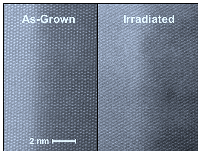
FIG. 4. High resolution STEM image of the GaN/AlGaIn interface before (left) and after (right) an irradiation of 6 \times 10^{14} \text{ H}^+/\text{cm}^2 . The interface is less abrupt after irradiation.
