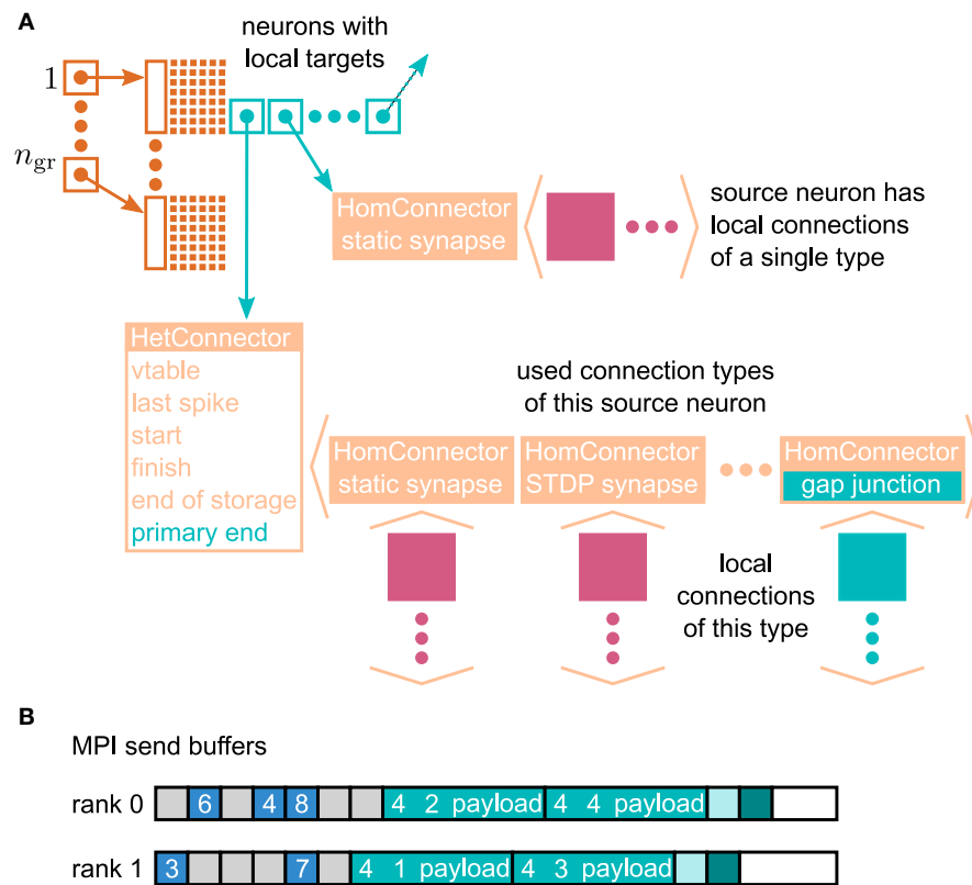
FIGURE 4 | Data structures for the representation of gap junctions. Turquoise elements indicate necessary changes to the fundamental data structures with respect to the 4g simulation kernel of NEST (cf. Kunkel et al., 2014). (A) Thread-local connection infrastructure. For all neurons a sparse table (dark orange) encodes whether at least one thread-local target is present or not. If a neuron has local targets, the sparse table stores a pointer (turquoise square with arrow) to a connection container (light orange data structure), where the least significant bits of this pointer encode whether gap junctions are present or not. The container is either a HomConnector or a HetConnector depending on whether the neuron has only one or more than one type of local connection. A HomConnector directly stores the connection objects, whereas a HetConnector stores a vector of HomConnectors, one per connection type. The HomConnectors for spiking connections come first in the vector and the member primary_end is the number of spiking connection types in the vector. (B) MPI send buffers accumulating outgoing events in the scheduler. Toy example for a particular communication interval with two MPI processes, where rank 0 hosts the neurons with even global IDs (GIDs) and rank 1 hosts the neurons with odd GIDs. Each buffer consists of two parts: the data related to spiking connections (blue boxes) followed by the data related to gap junctions (turquoise boxes). The spike data consist of the GIDs of the local neurons that spiked in the last communication interval, where markers (light gray boxes) define the end of a simulation interval (here four simulation steps per communication step) and thereby encode the spike time. For each local neuron that has gap junctions (here neurons 1–4) the corresponding buffer contains an entry, which consists of the ID of the connection type (here gap junctions have the ID 4), the GID of the neuron, and information about the state of the neuron (payload). A marker (light turquoise box) defines the end of the gap-junction data. The final valid entry in each buffer is a boolean value (dark turquoise box), which encodes whether the local neurons require another iteration of the waveform-relaxation method. The buffers may not be completely filled (white boxes).
