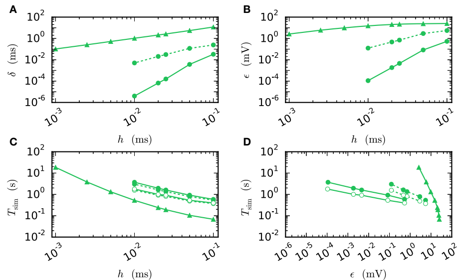
FIGURE 7 | Efficiency of a two-neuron simulation. Triangles show results with the single-step method, while circles indicate results obtained by the iterative method. Again solid curves indicate cubic interpolation and dashed curves were obtained with linear interpolation. The used communication scheme is indicated by open ( h -step communication) and filled symbols (communication in intervals of the minimal delay). The iteration control was used with prelim_tol chosen as 10^{-6} . (A) Shift of the spike times after 1 s of biological time plotted against used step size h . (B) RMSE \epsilon measured over 1 s of biological time plotted against the step size h . (C) Simulation time of the different approaches for 1 s of biological time. (D) Simulation time vs. RMSE \epsilon of the corresponding simulation.
