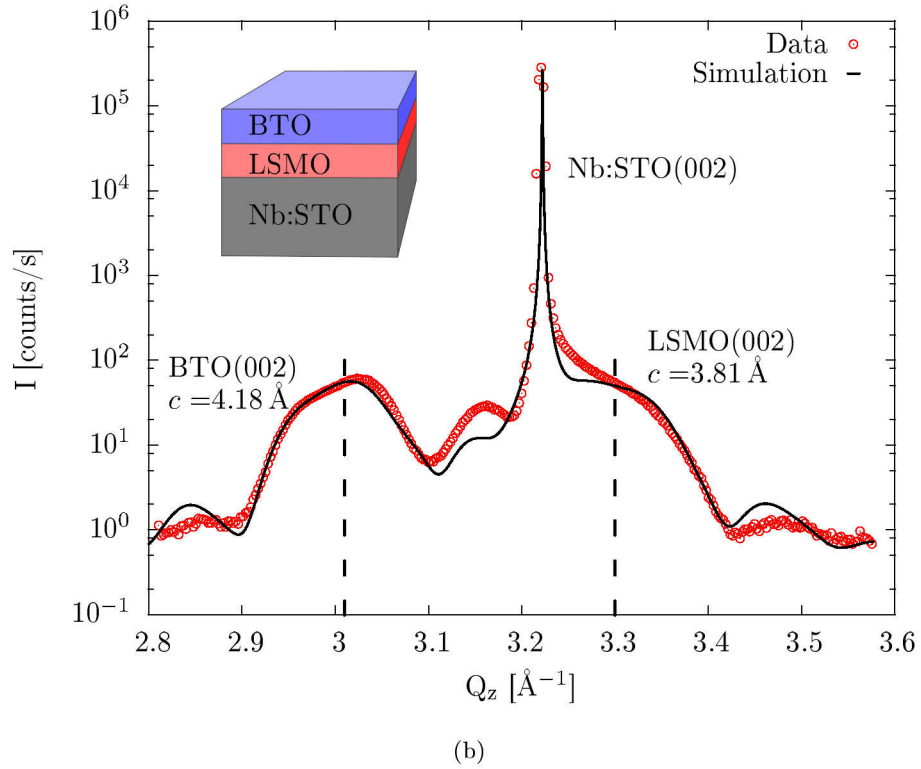
Figure 8.6: XRD measurements of both samples around the (002) reflections of the layers and the substrates. The given values for the out-of-plane parameters c are obtained by the peak positions resulting from the simulations. Simulations have been done by using the plot.py data evaluation software [108]. Detailed results are listed in table 8.1.
