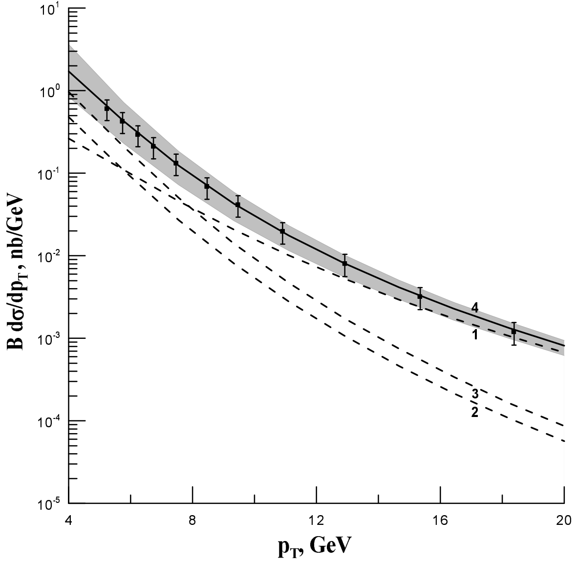
FIG. 2: J/\psi transverse momentum spectrum from \psi' decays from CDF Collaboration [27], \sqrt{S} = 1.8 TeV, |\eta| < 0.6 , (1) is the contribution of [^3S_1^{(8)}] state, (2) – [^3S_1^{(1)}] , (3) – [^1S_0^{(8)}] , (4) – sum of their all.
