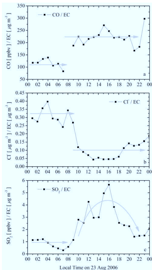
Figure 3. Time series of (a) CO, (b) \text{Cl}^- , and (c) \text{SO}_2 scaled by EC concentration, as indicators of air mass change. Light gray arrows illustrate the possible changes in the air masses.
