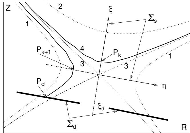
FIG. 2. Schematic view of magnetic field lines near the X-point and the separatrix mapping (18). Dotted curves 1–3 describe the unperturbed closed (curves 1), open (curve 2) field lines, and the separatrix (curve 3); solid curve 4 represents perturbed field lines; the section \Sigma_s consists of two segments of the \xi - and \eta -axes; the segments \Sigma_d correspond to the divertor plates; P_k ( k=0, \pm 1, \pm 2, \dots ) are the sequence of crossing points of the perturbed field line with the \xi - and \eta -axes; P_d is a hitting point of the perturbed field line with the divertor plate \Sigma_d ; \xi_d is a \xi -coordinate of the divertor plates. The unperturbed field lines (curves 1 and 2) transversely cross the axes (\xi, \eta) .
