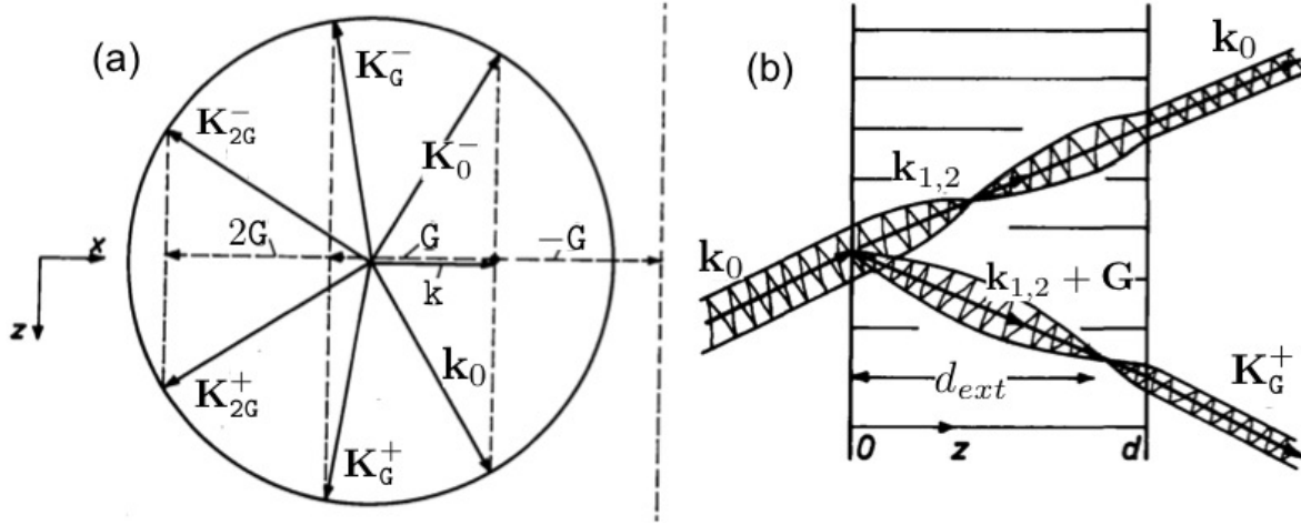
Fig. 8: (a) Plane waves \mathbf{K}_G^\pm in the vacuum. (b) Wave fields in the symmetrical Laue case at exact Bragg condition ( W = 0 ). Taken from [11].
