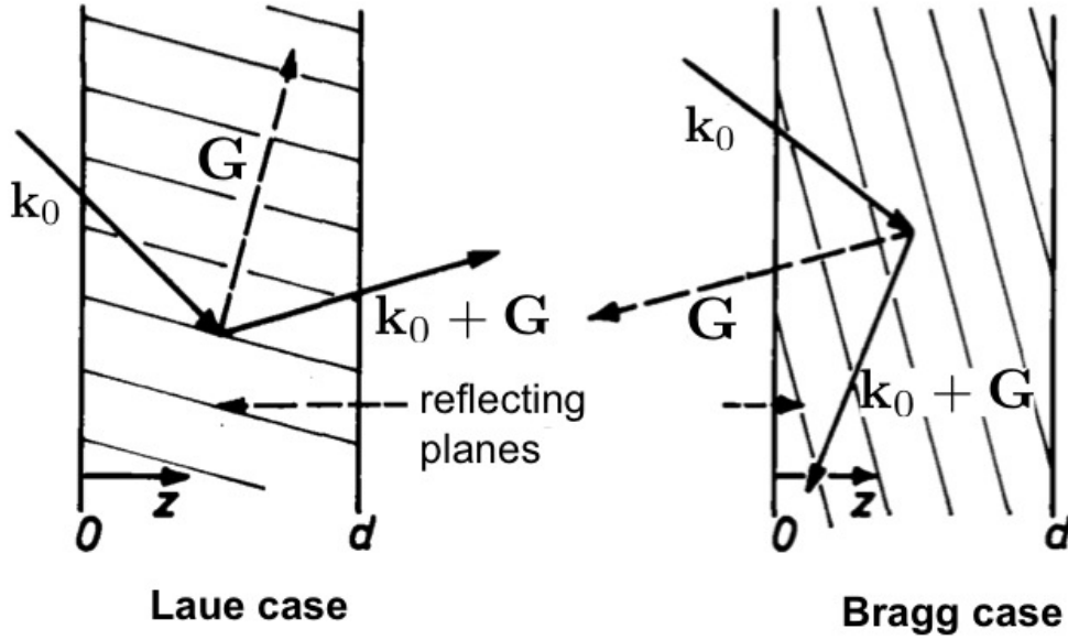
Fig. 6: Incident wave k_0 and reflected wave k_0 + G for the Laue and Bragg case. Taken from [11].
