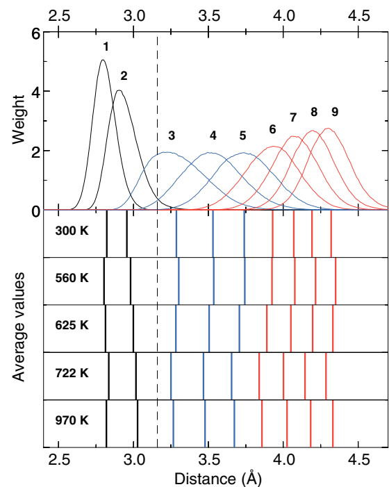
FIG. 8. (Color online) Near-neighbor distributions in a -Te at 300 K. The bars show the average distances at each temperature.
