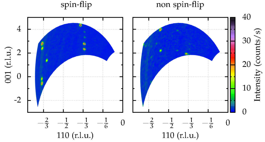
Figure A.18: hhl-plane at 230 K on warming.
