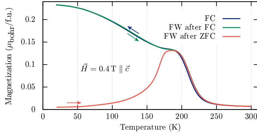
Figure 3.13: Magnetization of sample Z5G2 of NS-type. The red curve is measured during field warming (FW) at H = 0.4 \text{ T} after cooling without field, the green curve during FW after cooling in a 0.4 T field and the blue curve is field cooling (FC).
