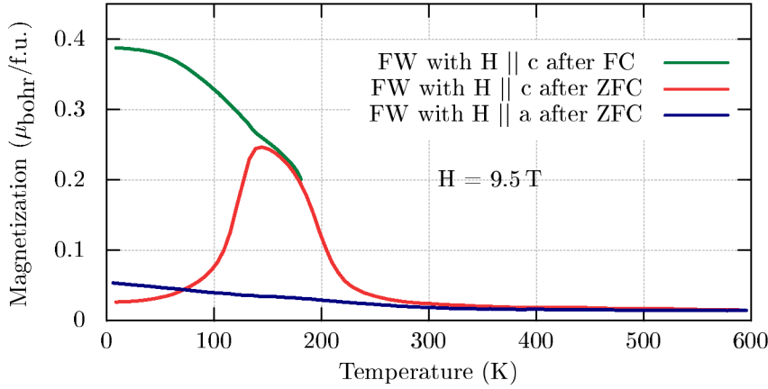
Figure 1.6: Magnetization of non-stoichiometric YFe 2 O 4-δ single crystal. (Data taken from [15]).
