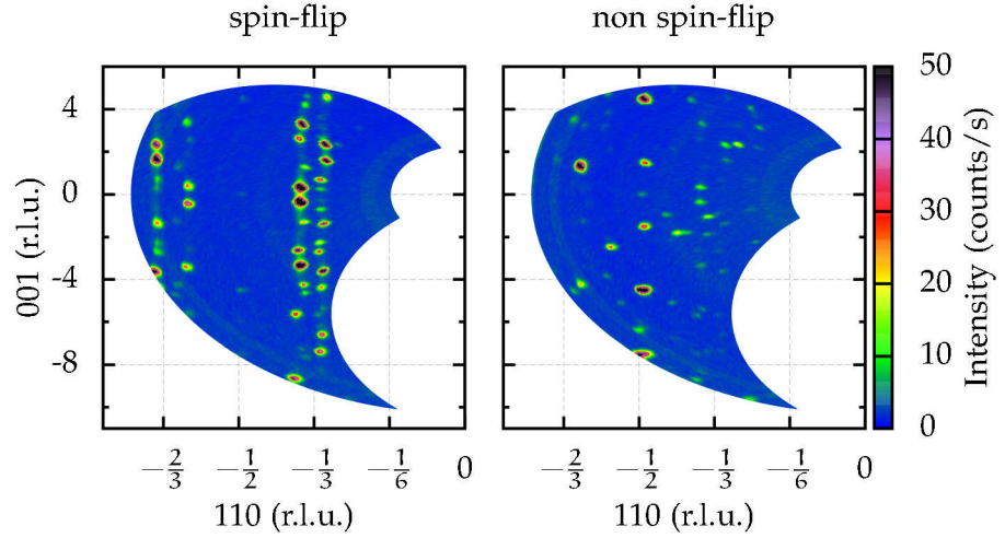
Figure 3.35: hhl -plane at 160 K in spin-flip (left) and non spin-flip (right) channel with magnetic field H \parallel z .
