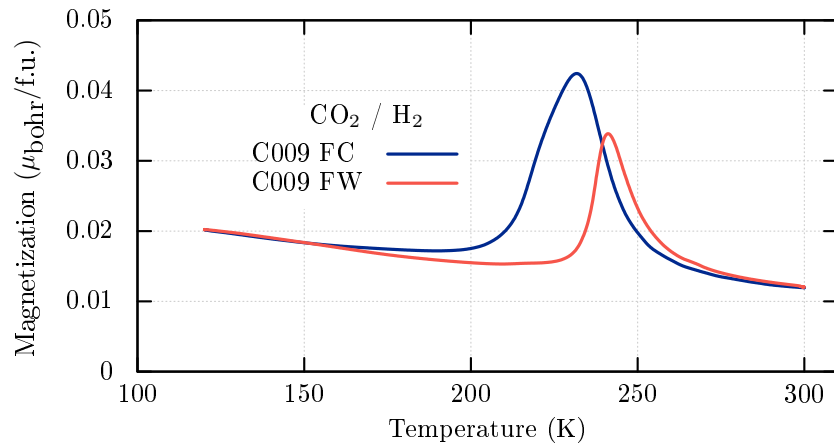
Figure A.8: Magnetization during field cooling and field warming at 3970 Oe for the calcination C009 ( \text{CO}_2/\text{H}_2 = 5.42 ).
