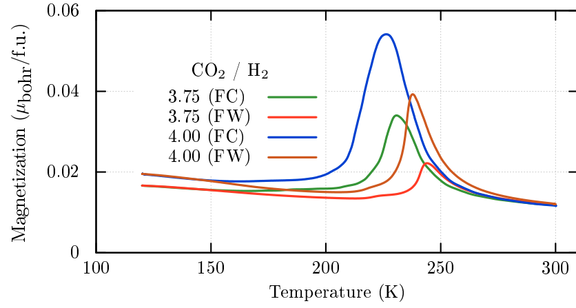
Figure A.2: Magnetization during field cooling and field warming at 3970 Oe for the calcinations C006 ( \text{CO}_2/\text{H}_2 = 3.75 ) and C015 ( \text{CO}_2/\text{H}_2 = 4.00 ).
