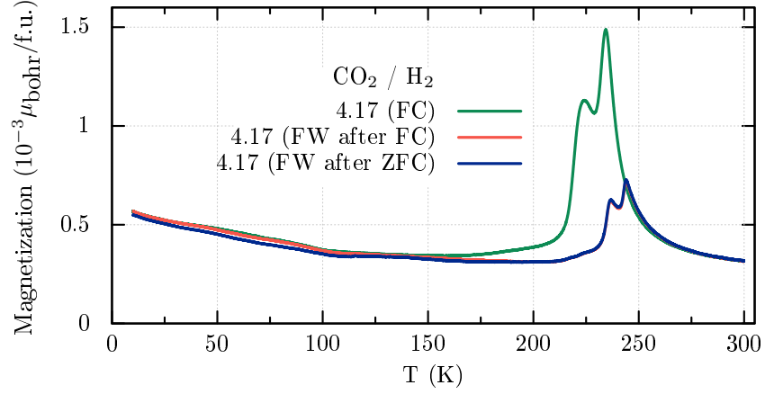
Figure 3.5: Magnetization during field cooling, following field warming and field warming after zero field cooling at 100 Oe for the calcination C003 ( \text{CO}_2/\text{H}_2 = 4.17 ) at a cooling rate of 1.5 K/min.
