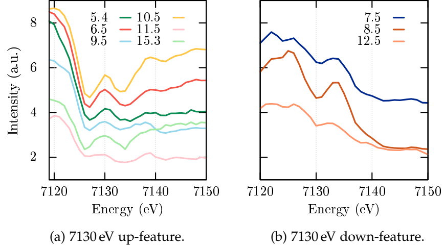
Figure 3.26: Energy spectra over the Fe K-edge on (1/3 \ 1/3 \ \ell) for different half-integer \ell at 10 K (data is normalized, corrected for absorption and shifted) .
