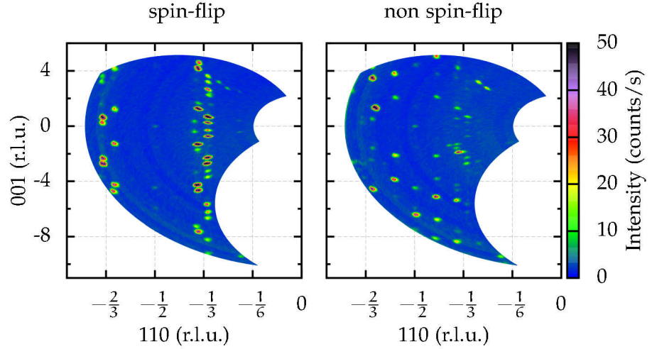
Figure 3.34: hhl -plane at 200 K in spin-flip (left) and non spin-flip (right) channel with magnetic field H \parallel z .
