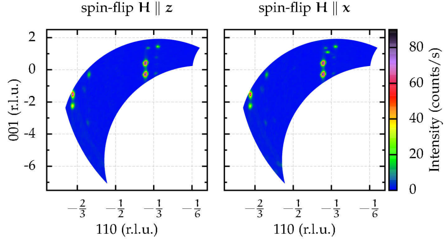
Figure 3.38: hh\bar{l} -plane at 160 K on cooling in spin-flip channel with magnetic field H \parallel z (left) and H \parallel x (right) — counting time: 15 s — five detector bank positions.
