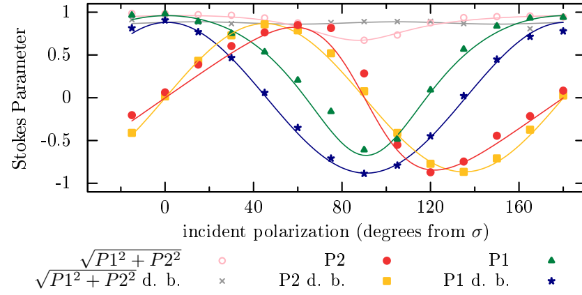
Figure A.11: Polarization analysis at 120 K on 7118 eV feature in RXRD on (\frac{1}{2}, \frac{1}{2}, 10.6) superstructure reflection (errors are the size of the symbols or smaller).
