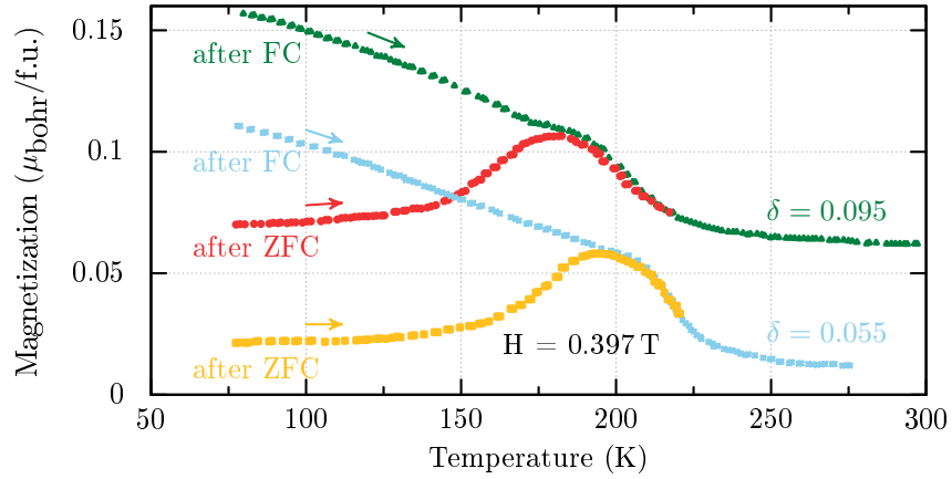
Figure 1.7: Magnetization of \text{YFe}_2\text{O}_{4-\delta} powder samples with different off-stoichiometry (Data taken from [18].) All curves are measured during warming, with previous cooling in a field H = 0.397 \text{ T} (FC) or without applied field ZFC.
