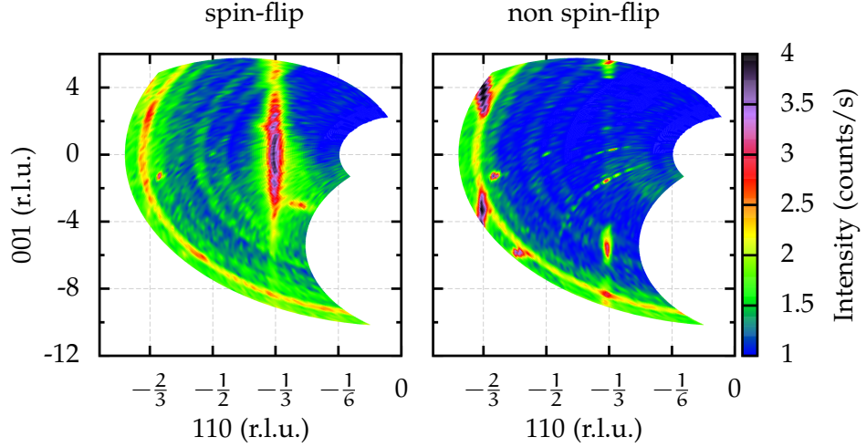
Figure 3.33: hhl -plane at 242 K on cooling in spin-flip (left) and non spin-flip (right) channel with magnetic field \mathbf{H} \parallel \mathbf{x} — counting time: 120 s — two detector bank positions.
