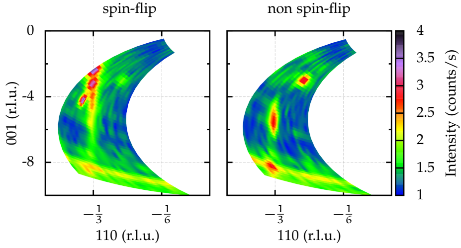
Figure A.12: hhl-plane at 236 K in spin-flip (left) and non spin-flip (right) channel with magnetic field \mathbf{H} \parallel \mathbf{z} .
