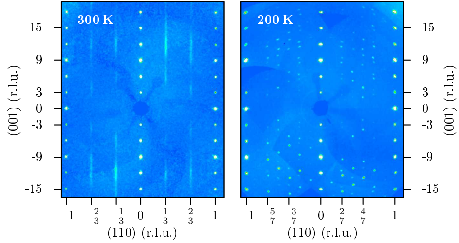
Figure 3.22: X-ray diffraction precession image of stoichiometric \text{YFe}_2\text{O}_{4-\delta} single crystal with magnetic behaviour of Type B. Projection in the (h\ell\ell) plane at 300 K (left) and 200 K (right) on cooling.
