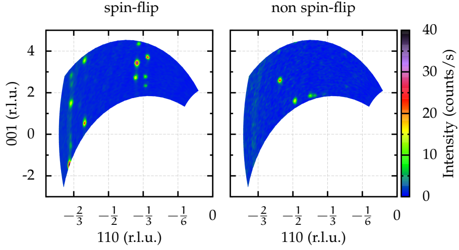
Figure A.15: hhl-plane at 185 K on warming.
