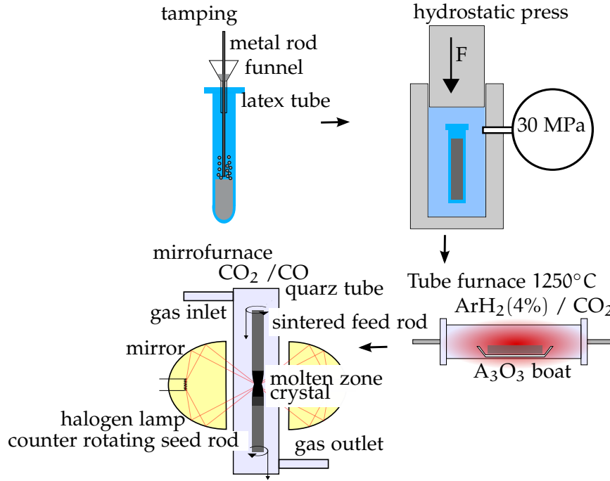
Figure 2.3: Schematic view of the crystal growth procedure.
