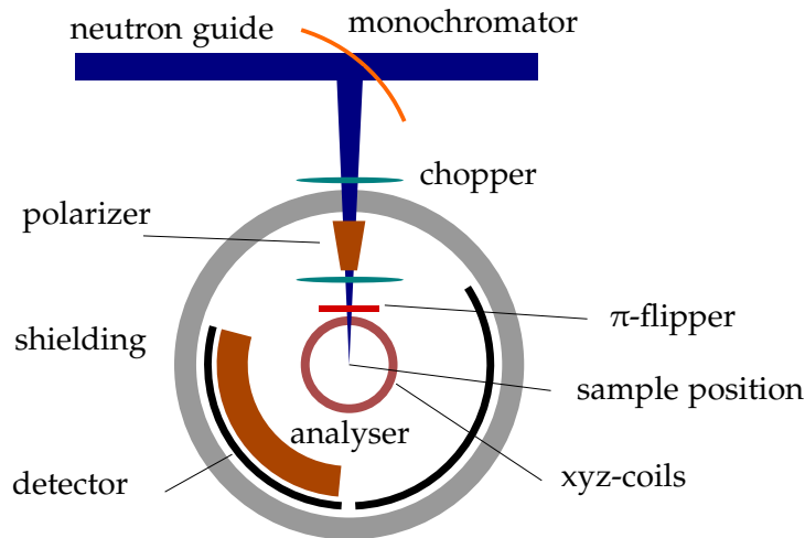
Figure 2.9: Schematic view of the DNS-instrument. [65]
