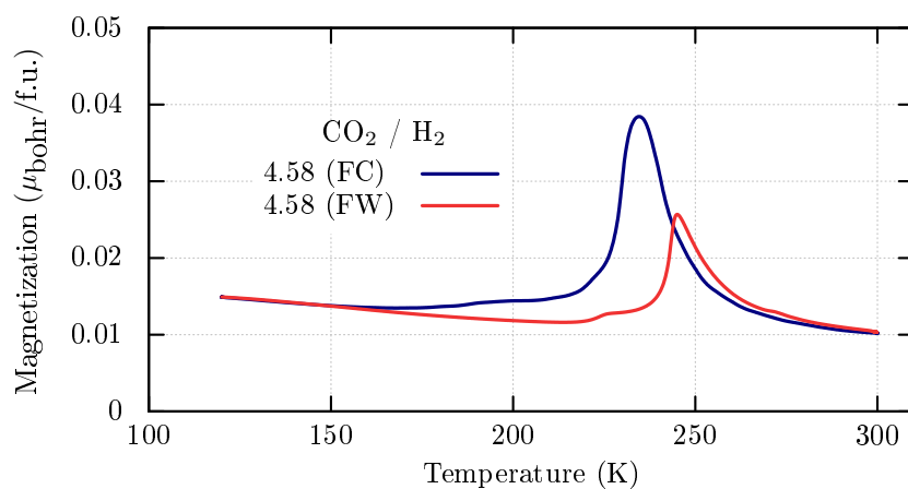
Figure A.5: Magnetization during field cooling and field warming at 3970 Oe for the calcination C008 ( \text{CO}_2/\text{H}_2 = 4.58 ) .
