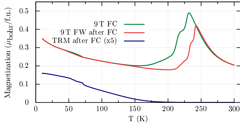
Figure 3.8: Magnetization during field cooling (1.5 K/min.) and following field warming (1.5 K/min.) at 9 T, also thermoremanent magnetization (1.5 K/min.) after 9 T field cooling (20 K/min.) for sample C003 ( \text{CO}_2/\text{H}_2 = 4.17 ).
