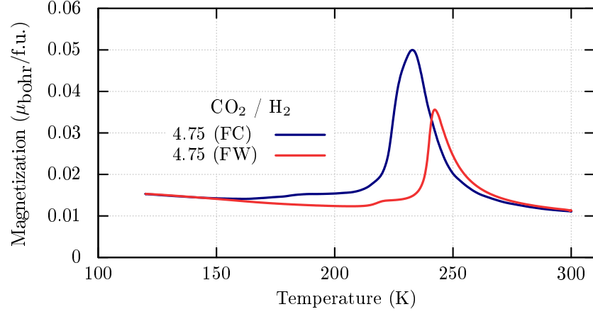
Figure A.6: Magnetization during field cooling and field warming at 3970 Oe for the calcination C013 ( \text{CO}_2/\text{H}_2 = 4.75 ).
