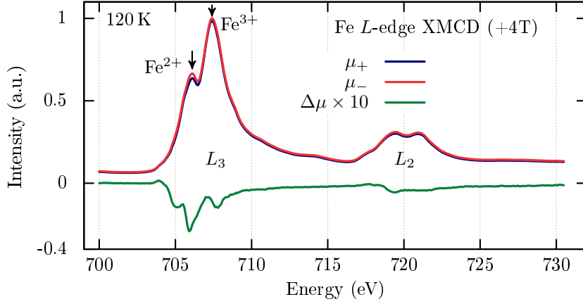
Figure 3.42: XAS spectra for left and right circularly polarized light over the Fe L-edge at 120 K for sample Z2 and XMCD signal. All received from total electron yield.
