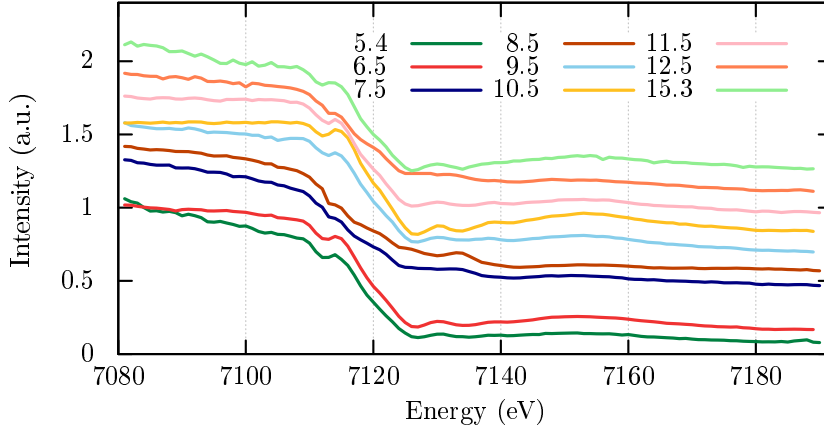
Figure 3.25: Energy spectra over the Fe K-edge on (1/3 \ 1/3 \ \ell = \text{half-integer}) for different half-integer \ell at 10 K (data is normalized and shifted) but not corrected for absorption.
