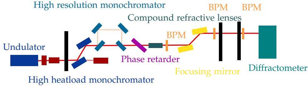
Figure 2.8: Schematic view of the P09 beamline at Petra III [63].
