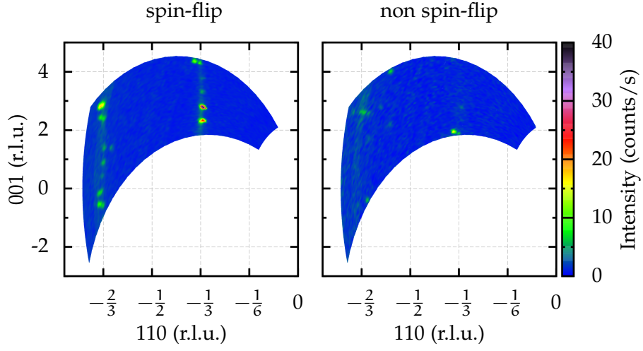
Figure A.21: hhl-plane at 230 K on cooling.
