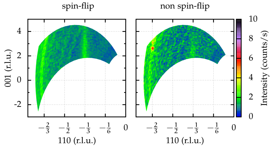
Figure A.20: hhl-plane at 255 K on warming — changed temperature scale.
