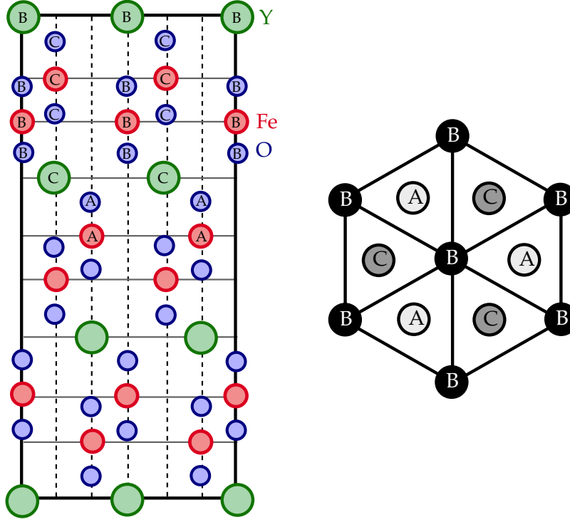
Figure 1.2: Rhombohedral R\bar{3}m crystal structure of \text{YFe}_2\text{O}_{4-\delta} at room temperature. The right part is the projection in c -plane, which shows three trigonal layers A, B and C stacked along c -axis as shown in the left part of the figure. The colours of the A, B and C positions identify the occupation by O, Fe or Y. Figure adopted from [7].
