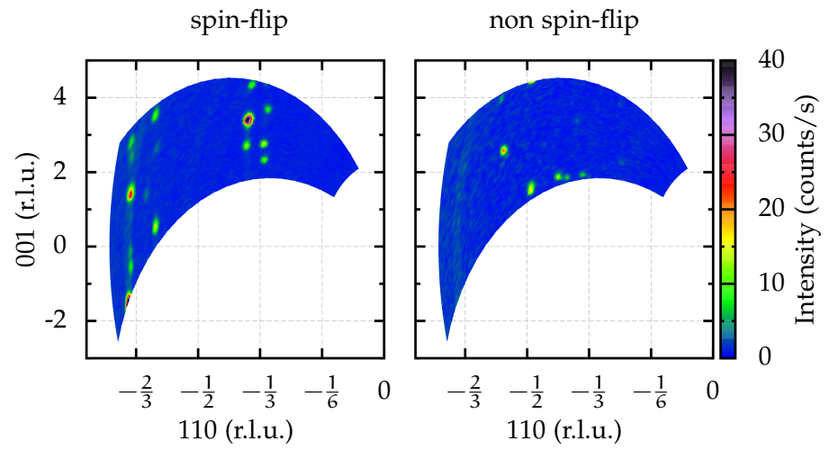
Figure A.26: hhl-plane at 170 K on cooling.
