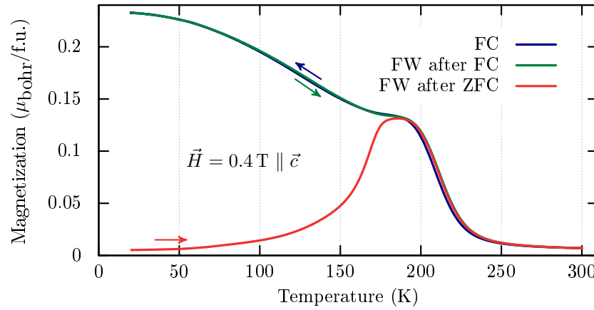
Figure 3.13: Magnetization of sample Z5G2 of NS-type. The red curve is measured during field warming (FW) at H = 0.4 T after cooling without field, the green curve during FW after cooling in a 0.4 T field and the blue curve is field cooling (FC).
