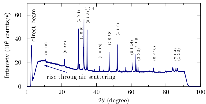
Figure A.1: Raw-data powder diffractogram of C001 (corrected data can be found in Figure 3.1).
