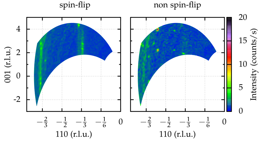
Figure A.19: hhl-plane at 240 K on warming — changed temperature scale.
