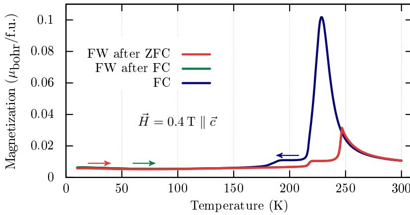
Figure 3.14: Magnetization of sample Z8G5real_S1 of Type B. The red curve is measured during field warming (FW) at H = 0.4 T after cooling without field, the green curve during FW after cooling in a 0.4 T field and the blue curve is field cooling (FC).
