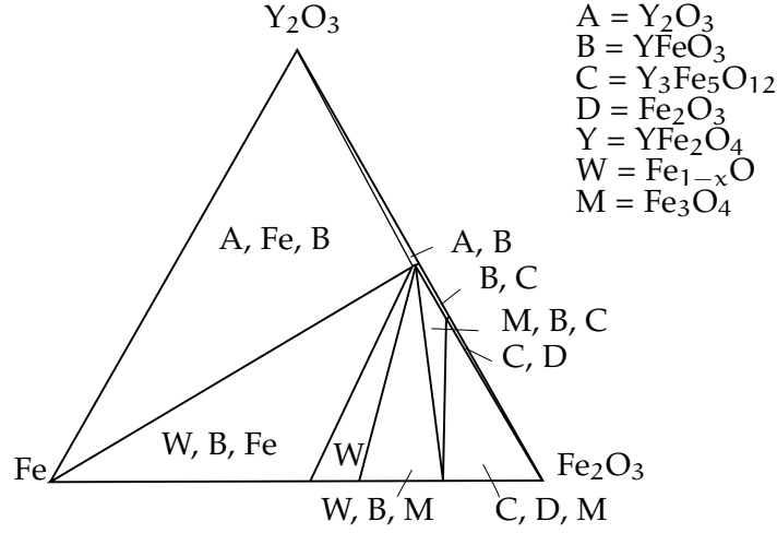
Figure 1.5: Phasediagram of the Fe-Fe 2 O 3 -Ye 2 O 3 -system at 1100 °C [13].
