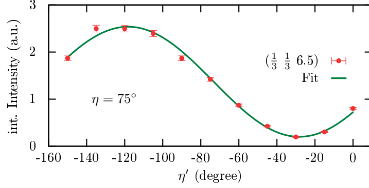
Figure 2.7: Fit of Equation 2.13 to the integrated intensities for incident polarization angle \eta = 75^\circ .
