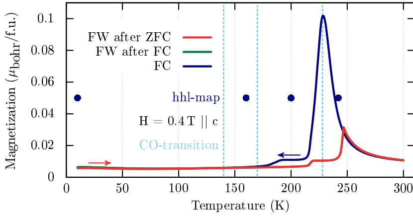
Figure 3.37: Magnetisation of sample Z8G5_S1, the blue dot marks position at which full hhl-maps were measured at the DNS experiment, while the light blue lines are roughly the charge ordering transitions.
