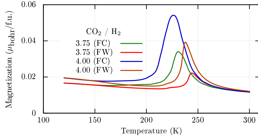
Figure A.2: Magnetization during field cooling and field warming at 3970 Oe for the calcinations C006 ( \text{CO}_2/\text{H}_2 = 3.75 ) and C015 ( \text{CO}_2/\text{H}_2 = 4.00 ).
