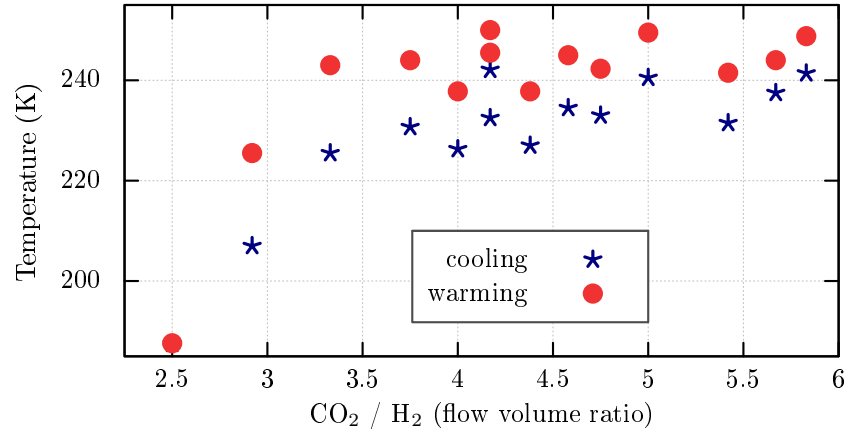
Figure 3.11: Analysis of the higher transition temperature (peak position) under the influence of varying \text{CO}_2 to \text{H}_2 ratio. Measured in a magnetic field of 3970 Oe.
