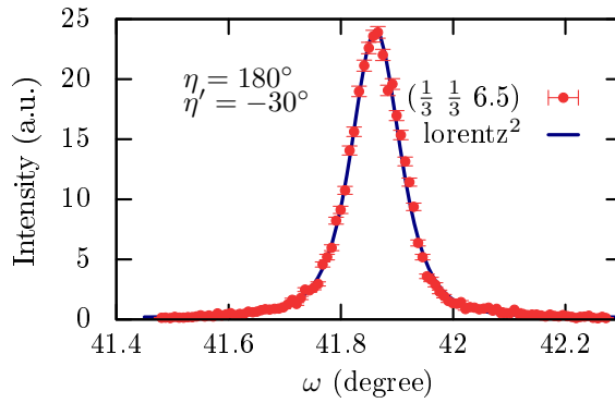
Figure 2.6: Rocking curve of the analyser crystal at 10 K at 7116.5 eV on (\frac{1}{3} \frac{1}{3} 6.5) superstructure reflection.
