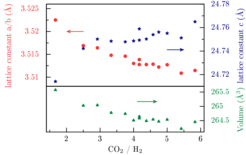
Figure 3.3: Dependence of the hexagonal lattice constants and the unit cell volume of \text{YFe}_2\text{O}_{4-\delta} from \text{CO}_2/\text{H}_2 -gas-mixture-ratio during synthesis. Higher ratio corresponds to smaller \delta .
