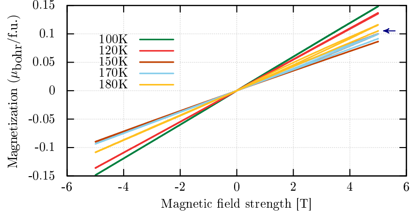
Figure 3.17: Field dependence of magnetization of sample Z2GinfS3 at temperatures between 100 K and 200 K with \mathbf{H} \parallel \mathbf{c} .
