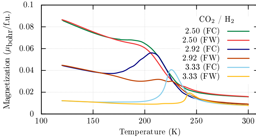
Figure 3.4: Magnetization during field cooling and field warming at 3970 Oe for the calcinations C001 ( \text{CO}_2/\text{H}_2 = 2.5 ), C012 ( \text{CO}_2/\text{H}_2 = 2.92 ) and C002 ( \text{CO}_2/\text{H}_2 = 3.33 ).
