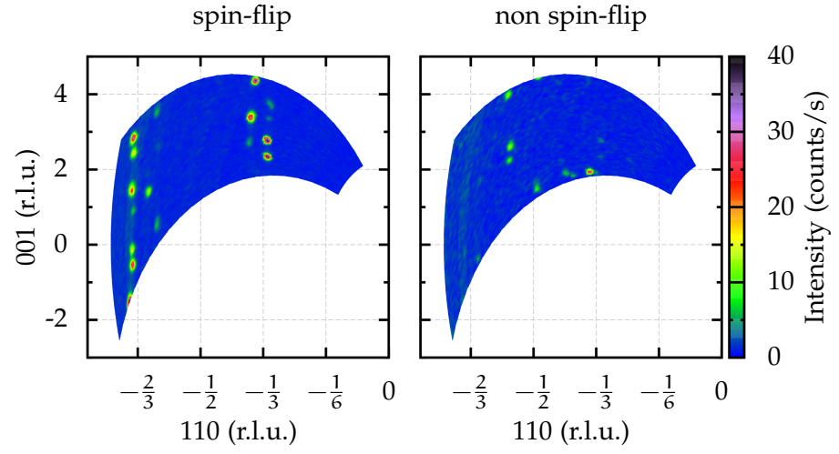
Figure A.24: hhl-plane at 190 K on cooling.
