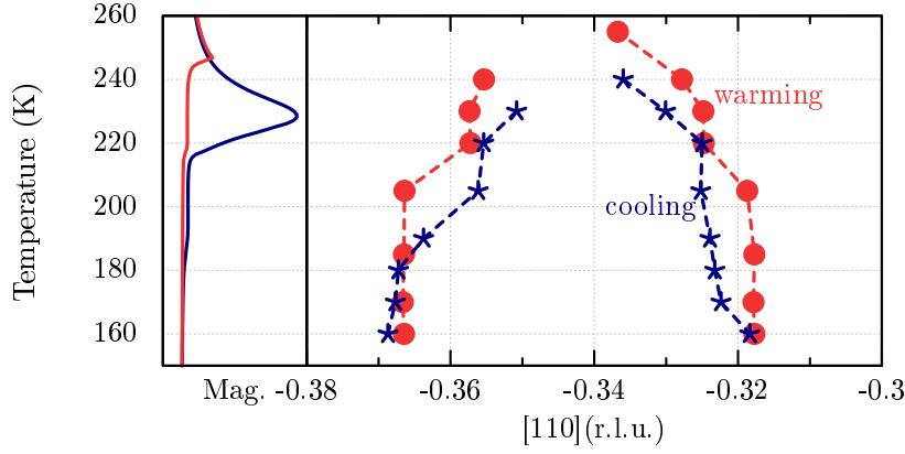
Figure 3.40: Temperature dependence of magnetic superstructure peak position in the (1/3 \ 1/3 \ \ell) -region — the points correspond to maxima in the, along \ell integrated, intensity. An example of the integrated intensity profiles is shown in Fig. 3.39.
