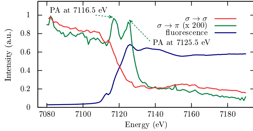
Figure 3.29: Energy spectra around the Fe K-edge on (1/2 \ 1/2 \ 10.75) at 120 K.
