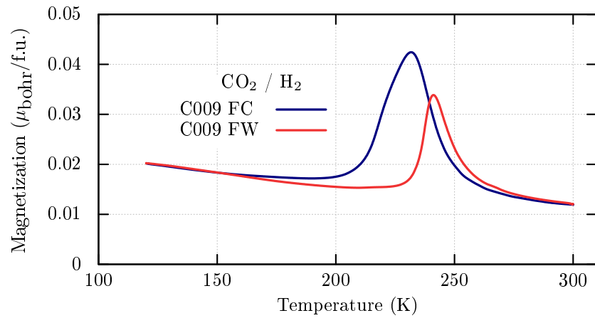
Figure A.8: Magnetization during field cooling and field warming at 3970 Oe for the calcination C009 ( \text{CO}_2/\text{H}_2 = 5.42 ).
