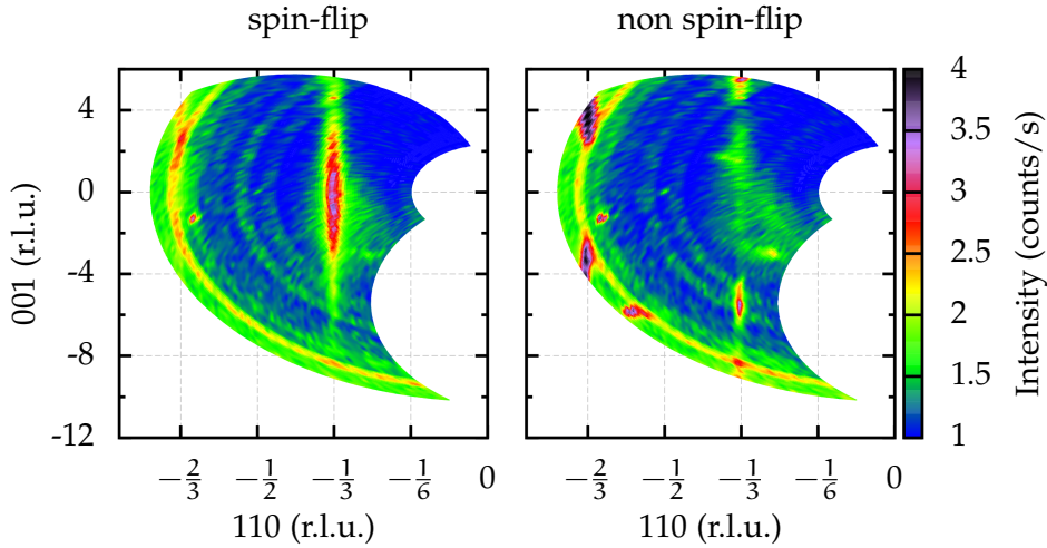
Figure 3.32: hhl -plane at 242 K on cooling in spin-flip (left) and non spin-flip (right) channel with magnetic field \mathbf{H} \parallel \mathbf{z} — counting time: 120 s — two detector bank positions.
