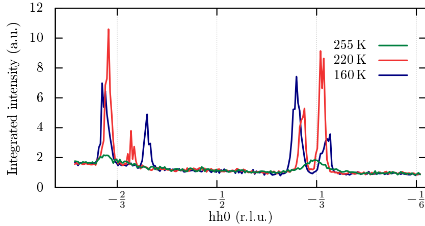
Figure 3.39: Along \ell integrated intensity at 160 K, 220 K and 255 K, all measured during warming.
