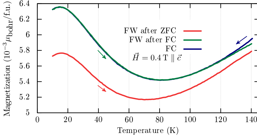
Figure 3.16: Magnification of the low temperature region of Fig. 3.14, showing the magnetization of sample Z8G5real_S1 below 140 K. The red curve is measured during field warming (FW) at H = 0.4 T after cooling without field, the green curve during FW after cooling in a 0.4 T field and the blue curve is field cooling (FC).
