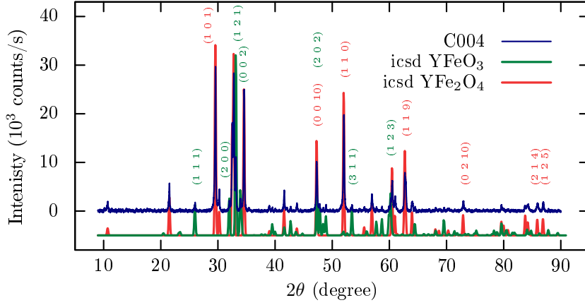
Figure 3.2: Powder x-ray diffractogram of C004 compared to the ICSD-Data of \text{YFe}_2\text{O}_{4-\delta} from [32] and \text{YFeO}_3 from [71]. (C004-Data is corrected for background. ICSD Data is shifted and scaled for clarity.)
