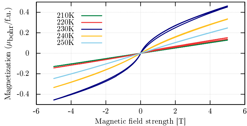
Figure 3.18: Field dependence of magnetization of sample Z2GinfS3 at different temperatures above 200 K with \mathbf{H} \parallel \mathbf{c} .
