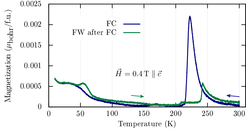
Figure 3.15: Magnetization of sample Z6G2_S6 of SB-type. The green curve is measured during field warming (FW) at H = 0.4 T after cooling in the same field and the blue curve during field cooling (FC).
