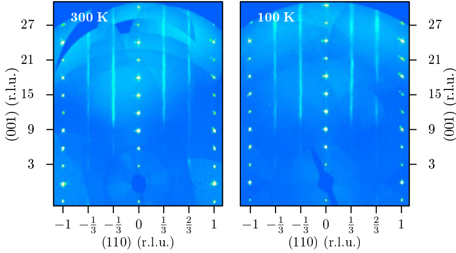
Figure 3.21: X-ray diffraction precession image of non-stoichiometric \text{YFe}_2\text{O}_{4-\delta} single crystal with magnetic behaviour of Type A. Projection in the (hh\ell) plane at 300 K (left) and 100 K (right) on cooling.
