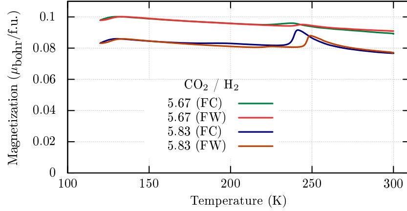
Figure 3.7: Magnetization during field cooling and field warming at 3970 Oe for the calcinations C011 ( \text{CO}_2/\text{H}_2 = 5.67 ) and C004 ( \text{CO}_2/\text{H}_2 = 5.83 ).
