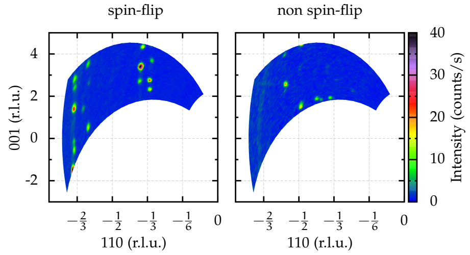
Figure A.25: hhl-plane at 180 K on cooling.
