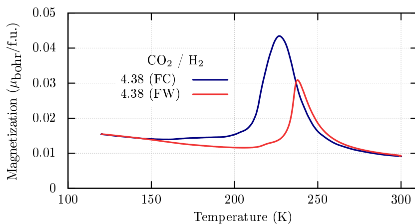
Figure A.4: Magnetization during field cooling and field warming at 3970 Oe for the calcination C014 ( \text{CO}_2/\text{H}_2 = 4.38 ) .
