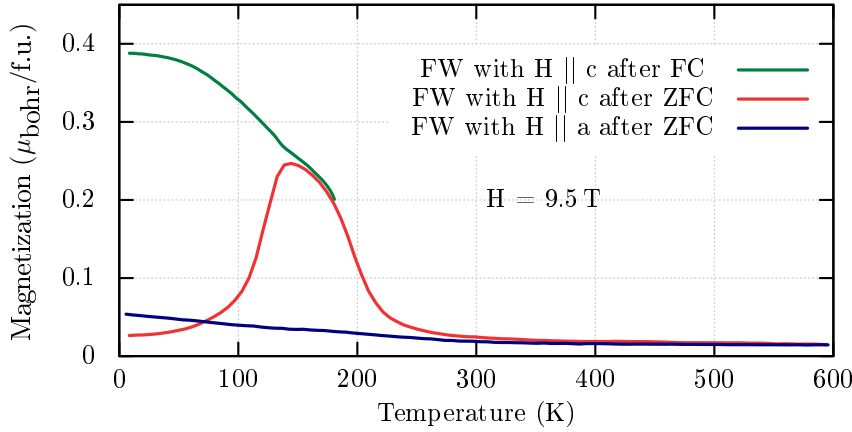
Figure 1.6: Magnetization of non-stoichiometric \text{YFe}_2\text{O}_{4-\delta} single crystal. (Data taken from [15]).
