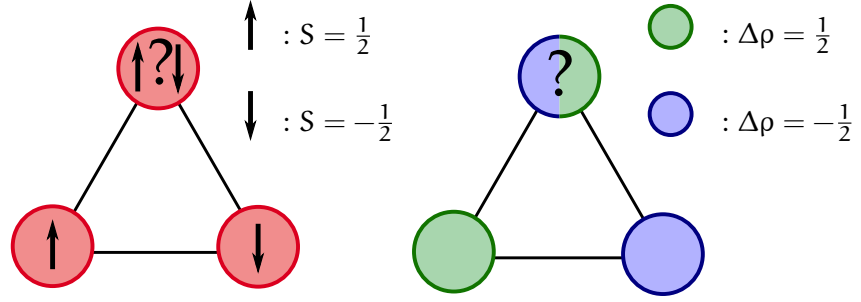
Figure 1.3: Spin and charge frustration in a triangular lattice. Figure adopted from [11].
