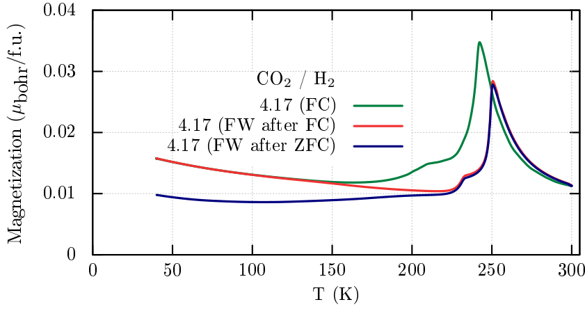
Figure 3.6: Magnetization during field cooling and field warming at 3970 Oe for the calcination C016 ( \text{CO}_2/\text{H}_2 = 4.17 ) at a cooling rate of 4 K/min.
