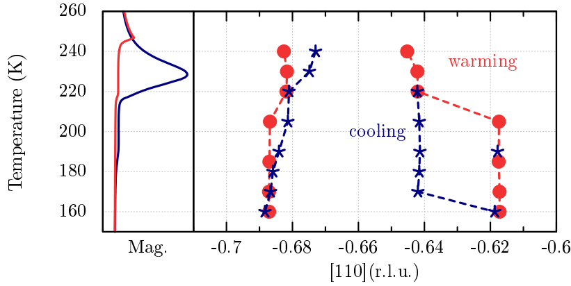
Figure 3.41: Temperature dependence of magnetic superstructure peak position in the (2/3 \ 2/3 \ \ell) -region — the points correspond to maxima in the, along \ell integrated, intensity. An example of the integrated intensity profiles is shown in Fig. 3.39.
