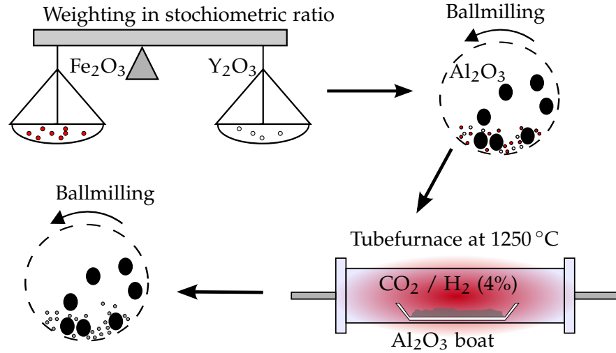
Figure 2.1: Process-diagram of the powder synthesis.
