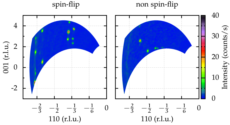
Figure A.16: hhl-plane at 205 K on warming.
