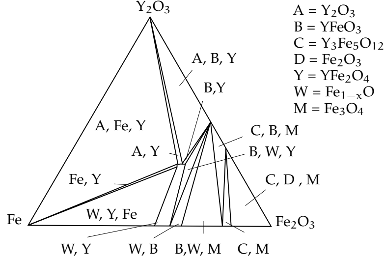
Figure 1.4: Phasediagram of the Fe-Fe 2 O 3 -Ye 2 O 3 -system at 1200 °C [12].
