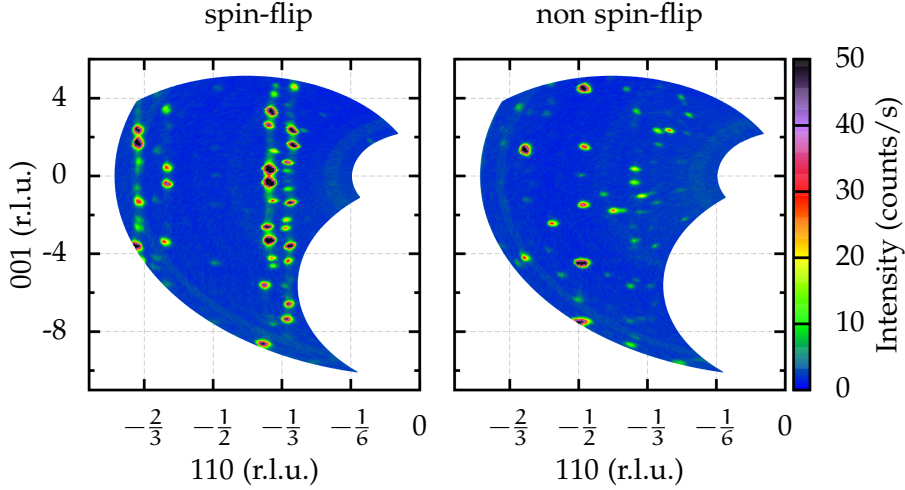
Figure 3.36: hhl-plane at 12 K in spin-flip (left) and non spin-flip (right) channel with magnetic field H \parallel z .
