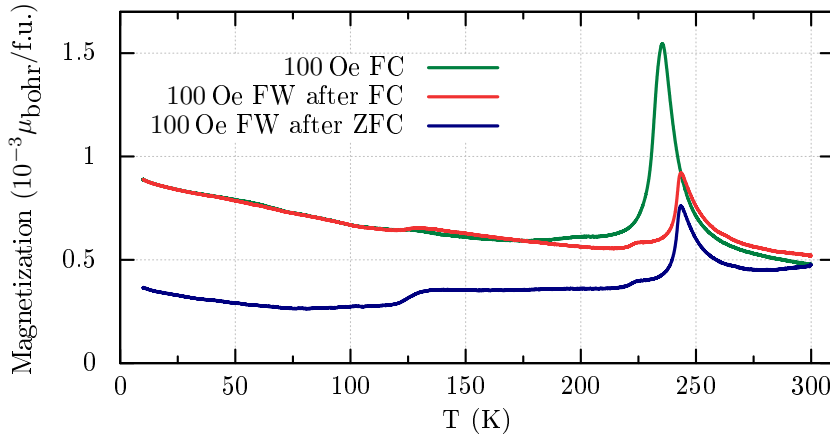
Figure 3.10: Magnetization during field cooling (1.5 K/min.) and following field warming (1.5 K/min.) at 100 Oe also field warming at 100 Oe (1.5 K/min.) after zero field cooling (20 K/min.) for sample C008 ( \text{CO}_2/\text{H}_2 = 4.58 ).
