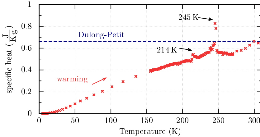
Figure 3.19: Specific heat of 1.08 mg sample Z2Ginf_S3 which is stoichiometric from magnetically Type B. The blue curve is the prediction from Dulong-Petit law, which sets an upper limit for the phononic specific heat contribution, ignoring molecule degrees of freedom or electron contributions.
