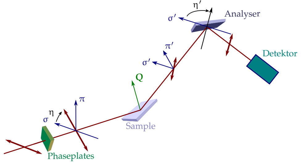
Figure 2.5: Schematic view of the diffractometer beam path in the polarization analysis setup [58].
