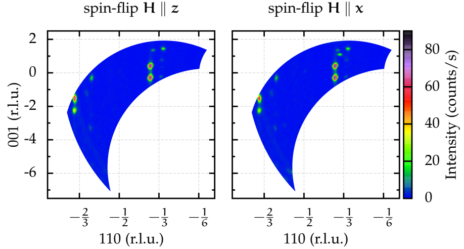
Figure 3.38: hhl -plane at 160 K on cooling in spin-flip channel with magnetic field H \parallel z (left) and H \parallel x (right) — counting time: 15 s — five detector bank positions.
