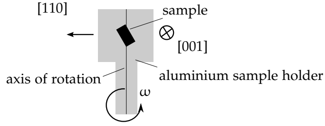
Figure 2.10: Sample holder and sample orientation in the DNS set-up.
