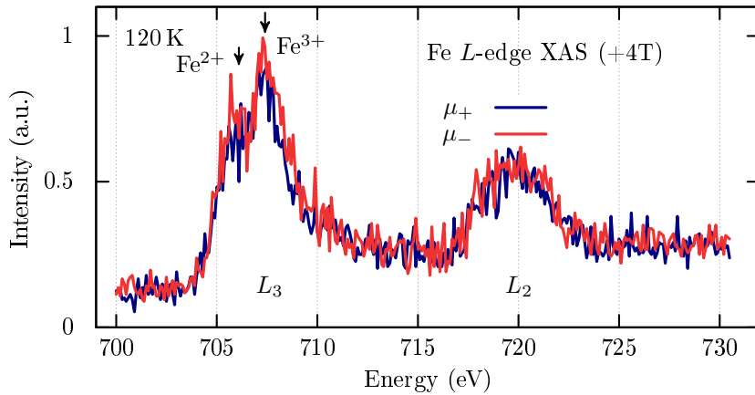
Figure 3.43: XAS spectra for left and right circularly polarized light over the Fe L-edge at 120 K. Measured with fluorescence detector.
