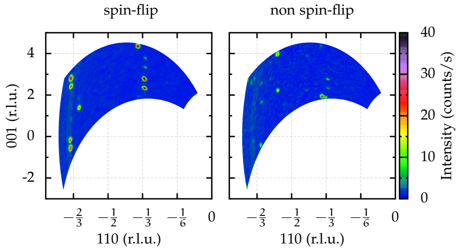
Figure A.23: hhl-plane at 205 K on cooling.
