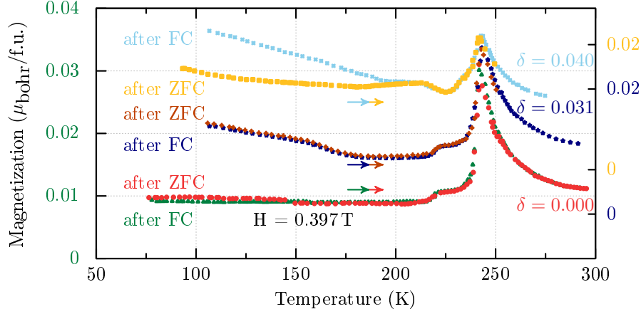
Figure 1.8: Magnetization of \text{YFe}_2\text{O}_{4-\delta} powder samples with different off-stoichiometry and stoichiometric oxygen amount (Data taken from [18]). The upper four curves are shifted for clarity by 0.007\mu_{\text{bohr}}/\text{f.u.} and 0.014\mu_{\text{bohr}}/\text{f.u.} respectively, as in [18]. All curves are measured during warming, with previous cooling in a field H = 0.397 \text{ T} (FC) or without applied field ZFC.
