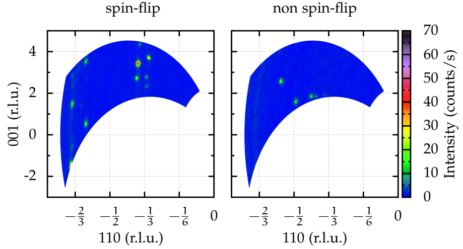
Figure A.14: hhl-plane at 170 K on warming — changed temperature scale.
