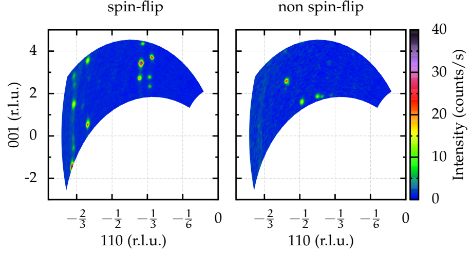
Figure A.13: hhl-plane at 160 K on warming.
