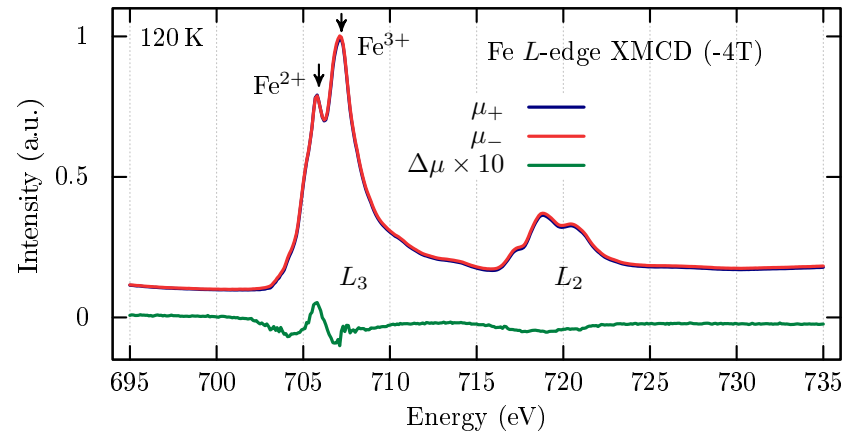
Figure 3.44: XAS spectra for left and right circularly polarized light over the Fe L-edge at 120 K for sample Z3 and XMCD signal. All received from total electron yield.
