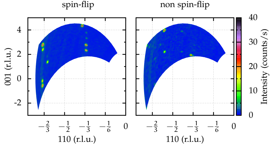
Figure A.18: hhl-plane at 230 K on warming.
