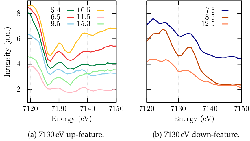
Figure 3.26: Energy spectra over the Fe K-edge on (1/3 \ 1/3 \ \ell) for different half-integer \ell at 10 K (data is normalized, corrected for absorption and shifted) .
