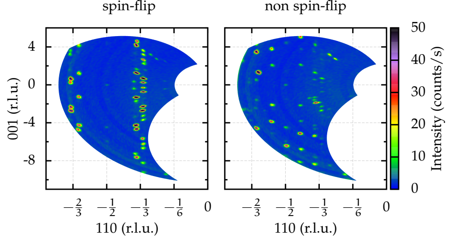
Figure 3.34: hhl -plane at 200 K in spin-flip (left) and non spin-flip (right) channel with magnetic field H \parallel z .
