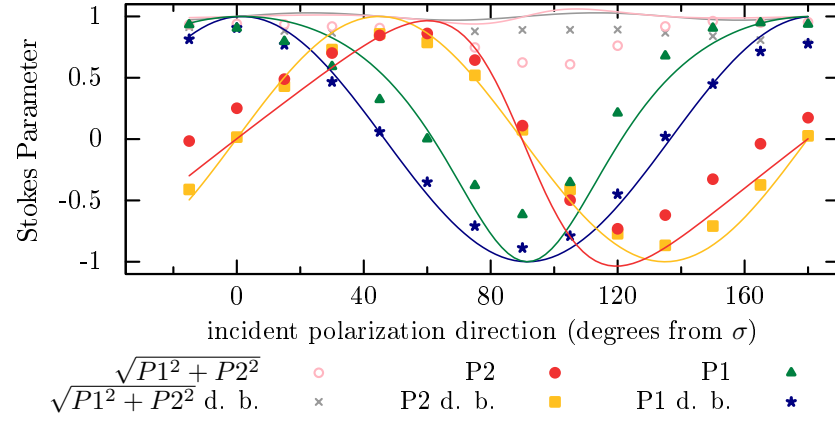
Figure A.10: [Polarization analysis at 120 K on 7125.5 eV feature in RXRD on (\frac{1}{2}, \frac{1}{2}, 10.6) superstructure reflection (errors are the size of the symbols or smaller). Amplitude of sinusoidal fit of the direct beam is fixed to 1.
