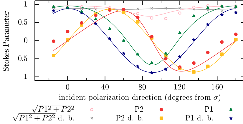
Figure 3.30: [Polarization analysis at 120 K on 7125.5 eV feature in RXRD on (1/2 \ 1/2 \ 10.6) superstructure reflection (errors are the size of the symbols or smaller).
