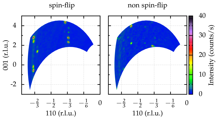
Figure A.17: hhl-plane at 220 K on warming.
