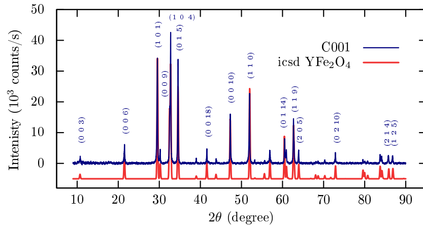
Figure 3.1: Powder x-ray diffractogram of C001 compared to the ICSD-Data of \text{YFe}_2\text{O}_{4-\delta} from [32]. (C001-Data is corrected for background. ICSD Data is shifted and scaled for clarity.)
