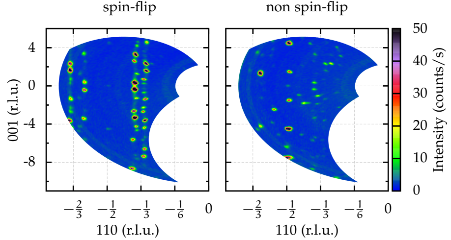
Figure 3.35: hhl -plane at 160 K in spin-flip (left) and non spin-flip (right) channel with magnetic field H \parallel z .
