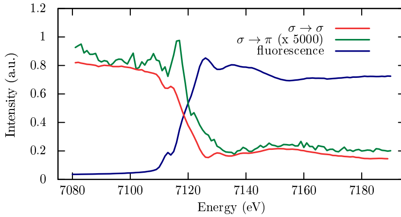
Figure 3.27: Energy spectra around the Fe K-edge on (1/3 \ 1/3 \ 6.5) at 10 K.
