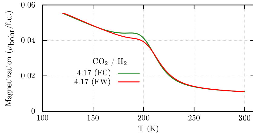
Figure A.3: Magnetization during field cooling and field warming at 3970 Oe for the calcination C017 ( \text{CO}_2/\text{H}_2 = 1.67 ).
