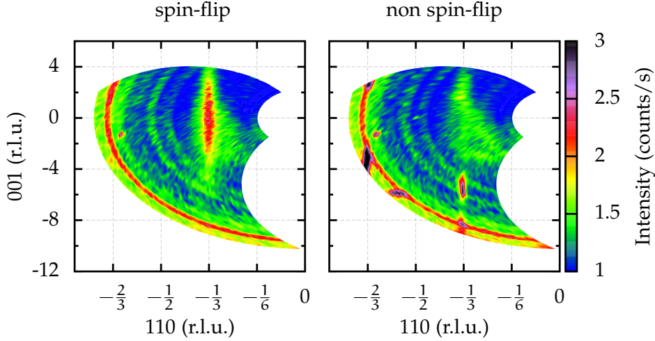
Figure 3.31: hhl -plane at 252 K in spin-flip (left) and non spin-flip (right) channel with magnetic field \mathbf{H} \parallel \mathbf{z} — counting time: 120 s — two detector bank positions.
