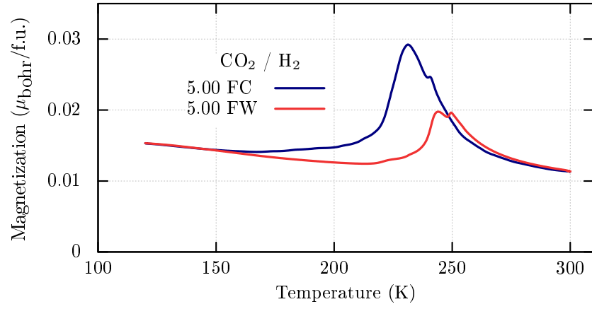
Figure A.7: Magnetization during field cooling and field warming at 3970 Oe for the calcination C005 ( \text{CO}_2/\text{H}_2 = 5.00 ).
