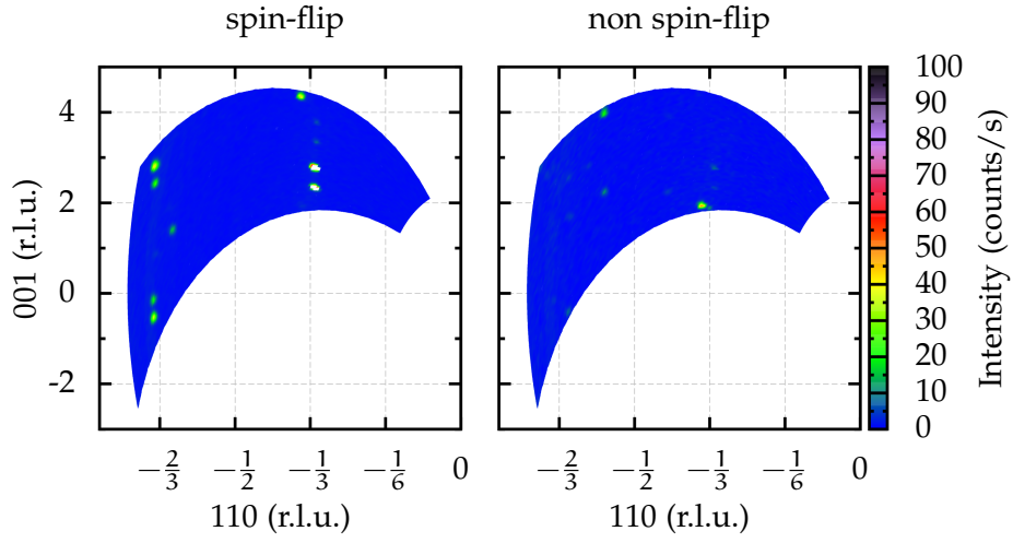
Figure A.22: hhl-plane at 220 K on cooling — changed temperature scale.
