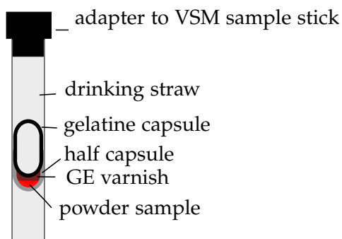
Figure 2.2: Powder sample holder for the PPMS VSM.
