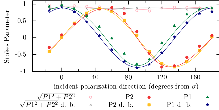
Figure 3.28: Polarization analysis at 10 K on 7116 eV feature in RXRD on (1/3 \ 1/3 \ 6.5) superstructure reflection (errors are the size of the symbols or smaller).
