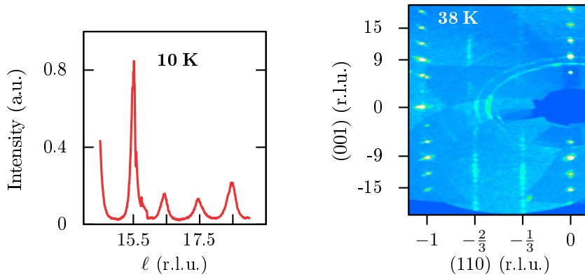
(a) Reciprocal scan along (1/3 \ 1/3 \ \ell) at 10 K on cooling. Recorded at the PETRA III P09 beamline. (b) Projection in the (hh\ell) plane at 38 K on cooling. Recorded with the SuperNova diffractometer and the Helijet option.
