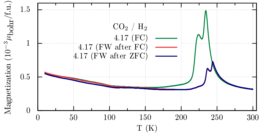
Figure 3.5: Magnetization during field cooling, following field warming and field warming after zero field cooling at 100 Oe for the calcination C003 ( CO_2/H_2 = 4.17 ) at a cooling rate of 1.5 K/min.
