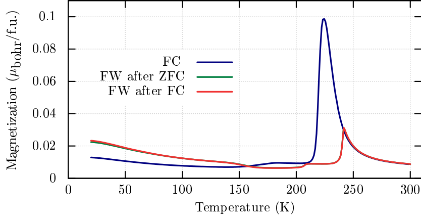
Figure A.9: Magnetization during field cooling and field warming at 3970 Oe after field cooling and zero field cooling for stoichiometric sample Z2Ginf_S3. Both field warming curves were measured after cooling with 10 K/min. While the cooling rate during measurement was 2 K/min. This leads to the difference at lower temperatures between FC and FW after FC. With the same cooling rate the curve would look like the Type B sample in Figure 3.14.
