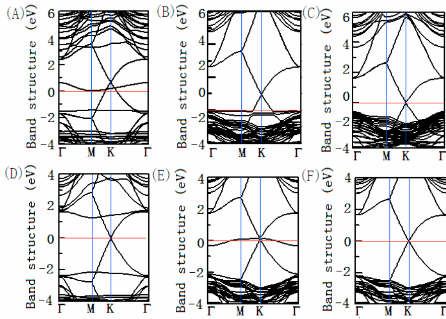
Fig. 6 The band structures of the mixed systems of graphene absorbed on \text{SiO}_2 surface: O-polar (0001) \alpha -quartz surface with pair oxygen due to physical absorption on top site (A), O-polar (111) cristobalite surface with bridge site (B), H-terminated O-polar (111) cristobalite surface with bridge site (C), Si-polar (0001) \alpha -quartz surface with bridge site (D), Si-polar (111) cristobalite surface with hexagonal center site (E) and H-terminated Si-polar (111) cristobalite surface with top site.
