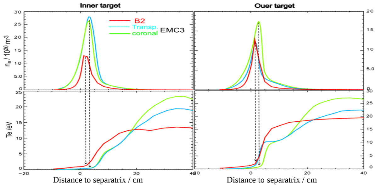
Fig. 4: Comparison of n_e and T_e profiles downstream
