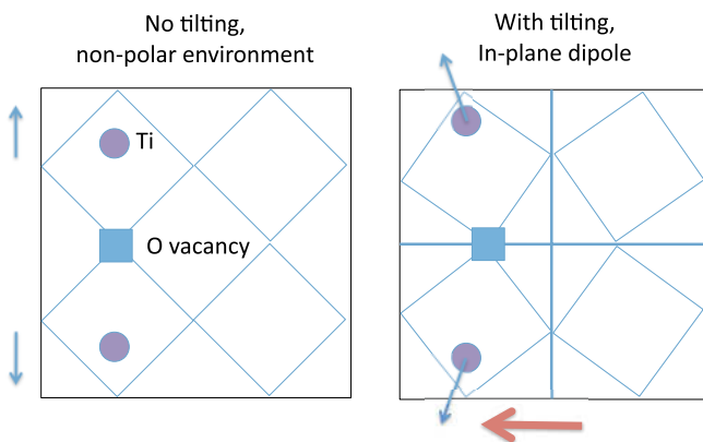
FIG. 11. (Color online) Schematic plot of the perovskite crystal structure in the view along [001] axis in the (a) untitled and (b) tilted AFD phases. Squares are marks for the oxygen octahedra, Eu cations are not shown. Orientation of the electric dipole moment created by the Ti displacement in the vicinity of oxygen vacancy in the tilted phase is marked by a large red arrow.
