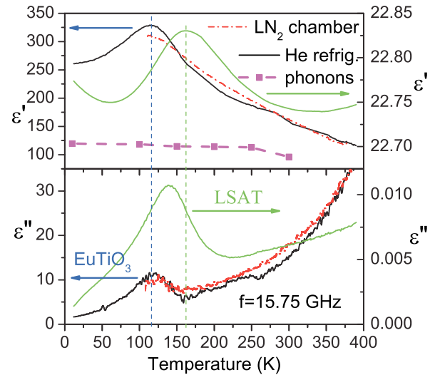
FIG. 6. (Color online) Temperature dependence of the complex permittivity in the 22-nm EuTiO 3 film (left scale) and the LSAT substrate (right scale) measured at 15.75 GHz. The thin-film MW data were obtained using two low-temperature devices (LN 2 chamber and He refrigerator). Static permittivity calculated from the phonon contributions (solid dots) is shown for comparison.
