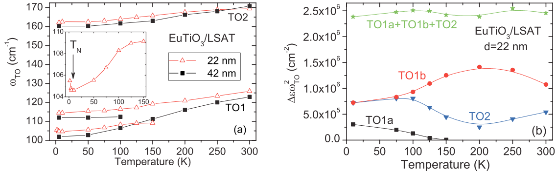
FIG. 4. (Color online) (a) Temperature dependence of the phonon frequencies for the EuTiO 3 films of two thicknesses 42 and 22 nm below 170 cm -1 . Stiffening of the TO1 and TO2 phonon frequencies in the more strained 22-nm film is seen. The new mode in the 22-nm film activates by 50 K higher than in the thicker film. The inset shows the temperature dependence of the new mode frequency in expanded scale down to 1.9 K. Mode hardening below the Néel temperature is clearly seen. (b) Temperature dependence of the oscillator strengths of all the modes seen below 200 cm -1 . One can see that the new TO1a mode gains strength from the TO1b mode. The sum of the oscillator strengths of all three modes remains constant within accuracy of the measurements, i.e., the sum rule (Ref. 13) is satisfied.
