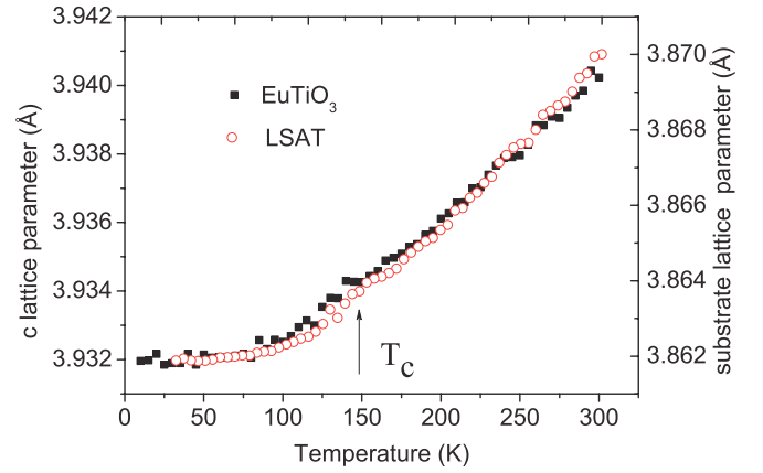
FIG. 10. (Color online) Temperature dependence of the out-of-plane lattice parameter of the \text{EuTiO}_3 film (thickness 22 nm) and of the LSAT substrate.
