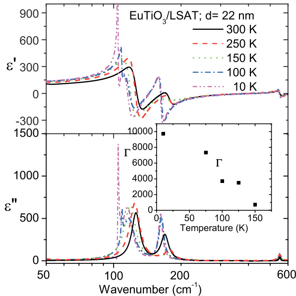
FIG. 5. (Color online) Complex dielectric function spectra of 22-nm EuTiO 3 film evaluated at various temperatures from the reflectance spectra in Fig. 3. The inset shows the temperature dependence of the imaginary coupling constant between two lowest-frequency modes.
