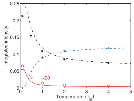
FIG. 5. (Color online) Calculated integrated intensity of the one-magnon band (black stars), two-magnon band (red circles; note the intensity is scaled by a factor of 20 to be visible on the same scale), and central quasielastic band (blue crosses), as computed in Ref. 21 using 16 spin diagonalizations for copper nitrate. The temperature is rescaled to the dimer energy J . The black dash-dotted line is the zero bandwidth limit result discussed in Sec. IV B, and the blue dashed line is the corresponding value for the central peak (see Ref. 7). The red solid line is the intensity predicted for the two-magnon scattering from perturbation theory; see Sec. IV B.
