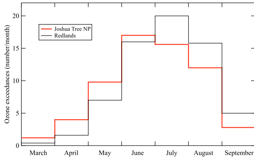
Figure 13. Number of days each month with daily maximum 8-h average ozone greater than 75 ppbv at Joshua Tree NP (red) and Redlands (black), averaged from 2006–2010.
