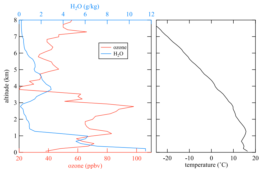
Figure 14. MOZAIC measurements of ozone (red), water vapor (blue), and temperature (black) over the LA Basin and Pacific Ocean following a 4:30 P.M. PDT departure from Los Angeles, CA on 7 June 2005.
