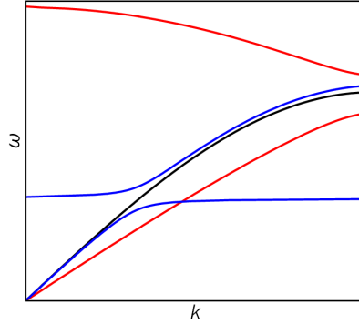
Figure 2: The phonon dispersion for a monoatomic linear chain (black curve), diatomic (red curve) and diatomic chain with stiff framework ( m_1, K ) and loosely bound guest atoms ( m_2, K_1, K_2 ) (blue curve) in the Born - von Karman approximation.
