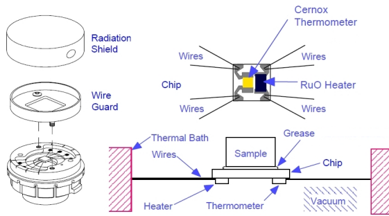
Figure 5: The sample holder (puck) for heat capacity measurements [25] using the QD-PPMS. The set of heater - thermometer and the sample position is shown. (Adapted from QD manual)
