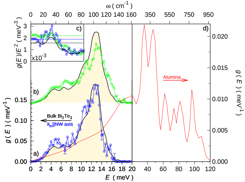
Figure 25: Te specific DPS measured in two orientations, (a) transmission (blue points) and (b) grazing (green points) incident geometry, on an array of \text{Bi}_2\text{Te}_3 nanowires with 56 nm diameter embedded in amorphous alumina template, typical error bar is given. For comparison, reference data (highlighted area) measured on bulk polycrystalline \text{Bi}_2\text{Te}_3 are shown. (c) Shows the Debye representation, g(E)/E^2 , and the extracted Debye level, \lim_{E \rightarrow 0} g(E)/E^2 , (color lines) are shown. The theoretically calculated DPS of amorphous alumina template is given in (d).
