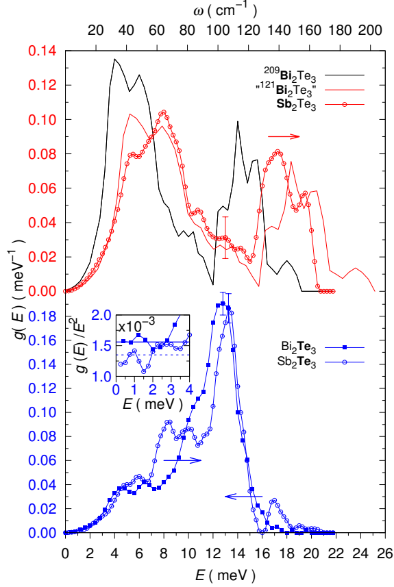
Figure 18: Element specific, Sb or Bi (red tics) and Te (blue tics), density of phonon states in \text{Sb}_2\text{Te}_3 (open circles) and \text{Bi}_2\text{Te}_3 (filled circles). The Bi specific DPS was extracted from the combination of NIS and reference neutron data [85] (black line) and renormalisation according to homology relation was applied (red line). Inset shows the Debye level calculated from the Te specific DPS measured in \text{Sb}_2\text{Te}_3 and \text{Bi}_2\text{Te}_3 .
