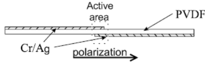
Figure 37: A scheme of the metallised PVDF transducer is shown where the PVDF, the metallised sides and the active area are shown.
