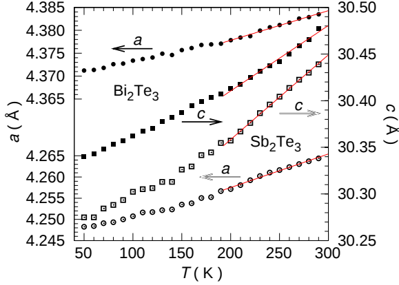
Figure 15: The temperature dependence of the a (circles) and c (squares) lattice parameters for \text{Sb}_2\text{Te}_3 (open tics) and \text{Bi}_2\text{Te}_3 (filled tics) between 50 and 300 K. Pointsize defines errorbar. The linear thermal expansion above 200 K in both orientations is indicated by red lines.
