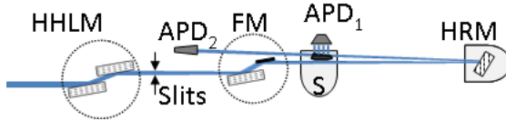
Figure 10: Experimental set-up for nuclear inelastic scattering measurements with high heat load monochromator (HHLM), high resolution monochromator (HRM), sample environment (S), avalanche photo diode detectors for measuring the instrumental function (APD2) and the inelastic spectrum (APD1). Figure is modified by Ref. [45].
