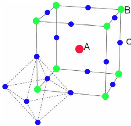
Figure 13: The perovskite structure in which \text{EuTiO}_3 crystallises. The A site are occupied by Eu atoms, the B sites by Ti atoms. Oxygen atoms are located at O sites.
