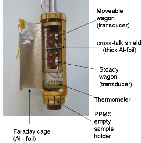
Figure 39: Resonant ultrasound spectrometer for small samples mounted in the QD cryostat sample holder.
