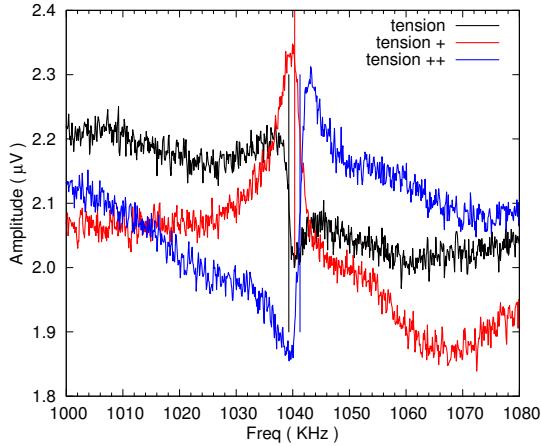
Figure 40: Sample loading effect in determination of resonant frequency in RUS measurement on a GaAs single crystalline sample with dimensions 1.0 mm · 1.1 mm · 0.5 mm. The central frequency is indicated by vertical line.
