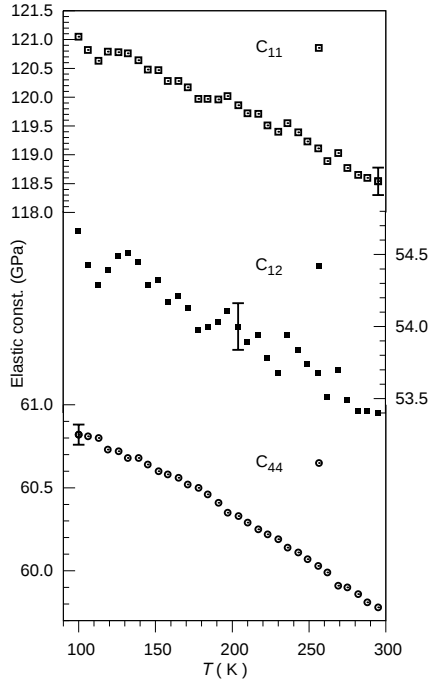
Figure 44: The elastic constants of GaAs between 100 and 300 K measured using the RUS cell for small samples constructed in this work
