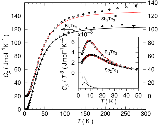
Figure 20: Specific heat at constant pressure, C_p , data measured on \text{Sb}_2\text{Te}_3 (circles) and \text{Bi}_2\text{Te}_3 (triangles) between 3 and 300 K and heat capacity at constant volume, C_v , calculated from low temperature DPS (red line). A typical errorbar is given. Inset: the Debye representation, C_p/T^3 , of both measurements. A fit of the experimental data was applied using a two level Schottky model superimposed to a Debye model with embedded Einstein oscillators (solid lines). The contribution of the Schottky model is given in the lower part of the inset. Specific heat measurements under 4 T magnetic field are shown as red symbols.
