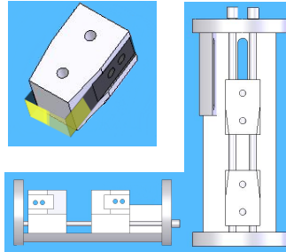
Figure 36: The transducer holder and the flexible transducer, see text, is shown in the left top figure. The bare RUS cell for small samples is shown in side view, bottom left, and top view perspective, bottom right.
