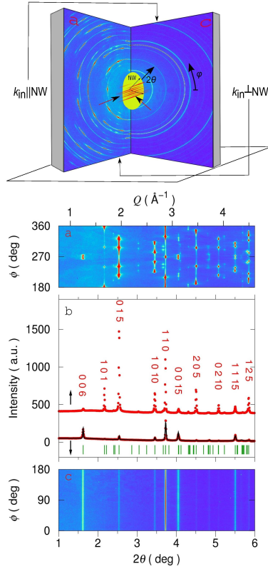
Figure 24: Diffraction of synchrotron radiation obtained on an array of \text{Bi}_2\text{Te}_3 nanowires with diameter of 56 nm embedded in a self ordered amorphous alumina membrane. (upper figure) shows the diffraction configuration. (a) shows the Debye - Scherrer rings recorded using a two dimensional area detector in grazing geometry versus the azimuthal angle \phi . (c) shows the azimuthal projection of the Debye - Scherrer measured on the same sample in transmission geometry. (b) shows the extracted diffractograms (red points) and the refinement (black line).
