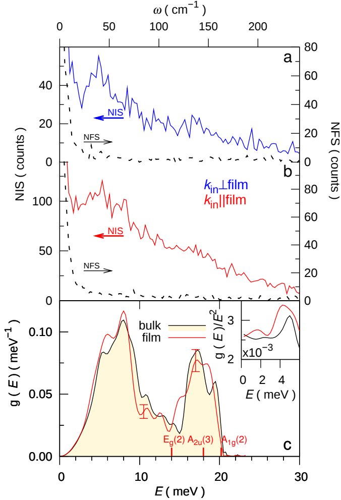
Figure 22: The nuclear inelastic spectra (lines) and the time integrated nuclear forward scattering, NFS-instrumental function (dashed lines), obtained in the elemental modulated \text{Sb}_2\text{Te}_3 film in two orientations. (a) with the incident wavevector, k_{\text{in}} , perpendicular to film surface and (b) with k_{\text{in}} parallel to the film surface. (c) shows the density of phonon states extracted with k_{\text{in}} parallel to the film surface (red) and the DPS measured on bulk \text{Sb}_2\text{Te}_3 . Inset: Debye level calculated from the Sb specific DPS measured in \text{Sb}_2\text{Te}_3 .
