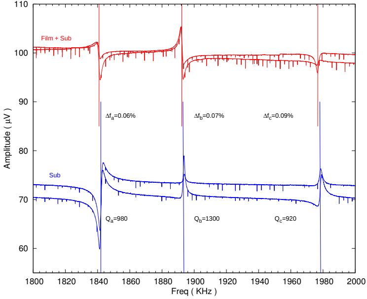
Figure 45: A comparison of two RUS spectra measured on a bare substrate and two spectra measured on the same substrate covered with \text{SnSb}_2\text{Te}_4 film.
