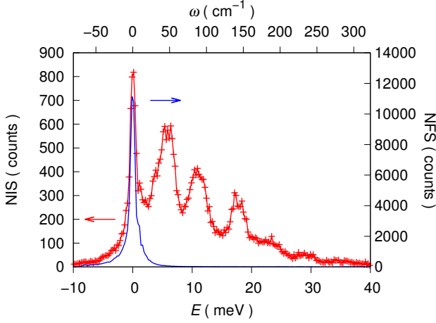
Figure 11: The nuclear inelastic scattering, NIS, measured on a polycrystalline metallic Te sample with the ^{125}\text{Te} resonance at 20 K (red points) and the time integrated nuclear forward scattering, NFS, which was measured as resolution function (blue line) [45].
