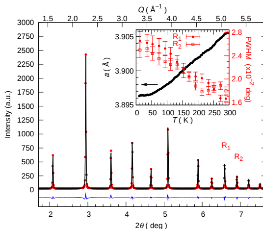
Figure 26: Rietveld refinement (black line) of a typical \text{EuTiO}_3 diffractogram (red points) at 300 K measured using synchrotron radiation and refinement residuals (blue line). Inset: the extracted temperature dependent lattice parameter (pointsize defines errorbars) in cubic symmetry and the Full Width at Half Maximum (FWHM) of certain reflections ( R_1 and R_2 ) are given.
