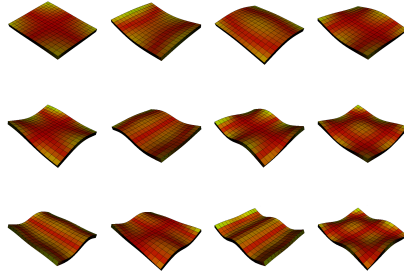
Figure 33: The first 12 normal modes of a sample with plate like geometry, dimensions 0.05 \text{ mm} \cdot 1.1 \text{ mm} \cdot 1.0 \text{ mm} . The figure was reconstructed from the calculated eigenvectors using Mathematica. The red areas denote high strain regions.
