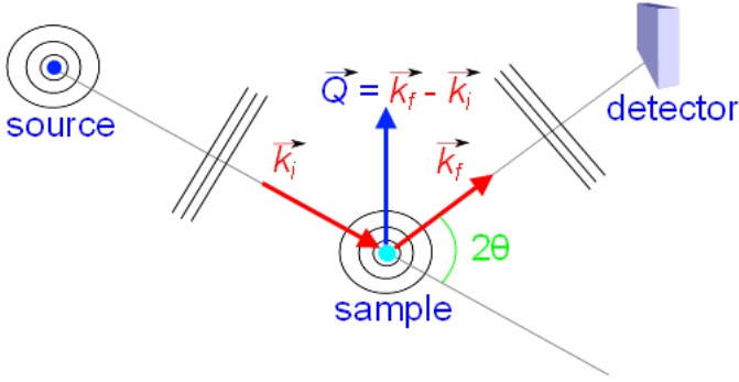
Figure 8: Elastic scattering process in the Fraunhofer approximation. The detector as well as the source is viewed at a long distance from the diffracting object.
