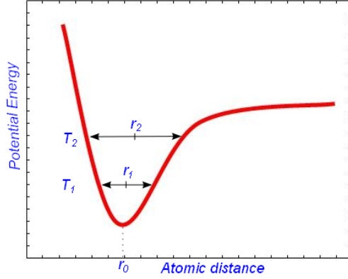
Figure 3: An anharmonic potential energy and the atomic distance equilibrium, r_0 , r_1 and r_2 at absolute zero temperature, at T_1 and at T_2 , respectively.
