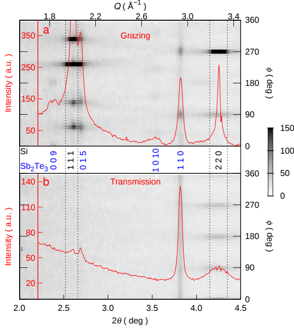
Figure 21: X-ray diffraction pattern of the elemental modulated \text{Sb}_2\text{Te}_3 film obtained at 295 K using synchrotron radiation in two orientations, see text, (a) grazing incident geometry and (b) transmission geometry. Background shows the actual detector pattern and red lines the related diffractograms. Expected peak positions are indicated by the corresponding Miller indices in pseudohexagonal setting.
