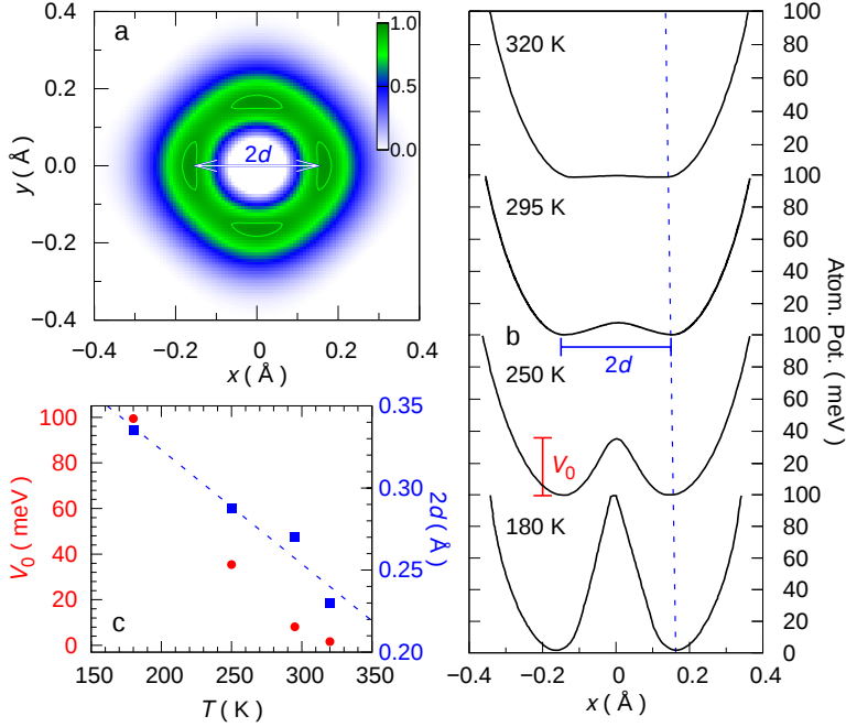
Figure 28: (a) Probability density function distribution of the Eu-atom in the ab plane at 180 K. (b) Shows the effective one-particle potential of the Eu atom along the a direction ( y = 0 ) at 320, 295, 250 and 180 K obtained from crystallographic structure analysis. (c) The potential barrier, V_0 , and the displacement from equilibrium position, 2d , (dashed line is guide to the eye) extracted from the potential given in (b).
