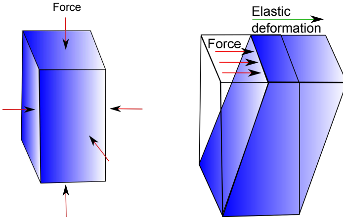
Figure 6: The applied external forces and the elastic deformation related to the bulk, left, and shear moduli, right are shown.
