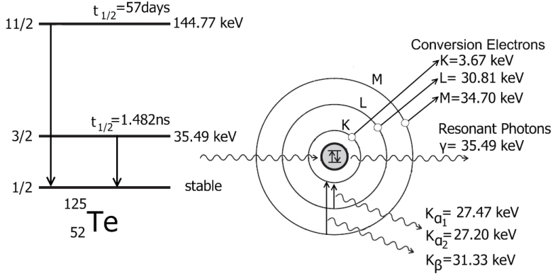
Figure 9: The nuclear excited states of ^{125}\text{Te} and various scattering and emission processes that can follow from resonant absorption of \gamma -photons. Data were summarized from [44].
