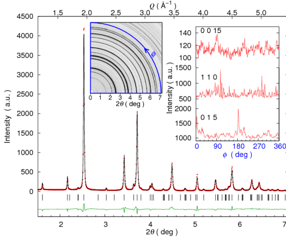
Figure 14: X-ray diffraction pattern of \text{Bi}_2^{125}\text{Te}_3 obtained at 295 K using synchrotron radiation (red dots), the expected peak positions (black ticks), the corresponding refinement (black line) obtained using Fullprof [40] and the difference plot (green line). Inset: (left) a quarter of the corresponding detector image, (right) intensity distribution along the \phi angle for the (0 1 5), (1 1 0) and (0 0 15) reflections in the pseudohexagonal setting.
