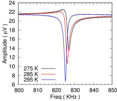
Figure 41: Temperature dependence of a resonance recorded between 275 and 295 K on the same GaAs single crystalline sample used in Fig. 40.
