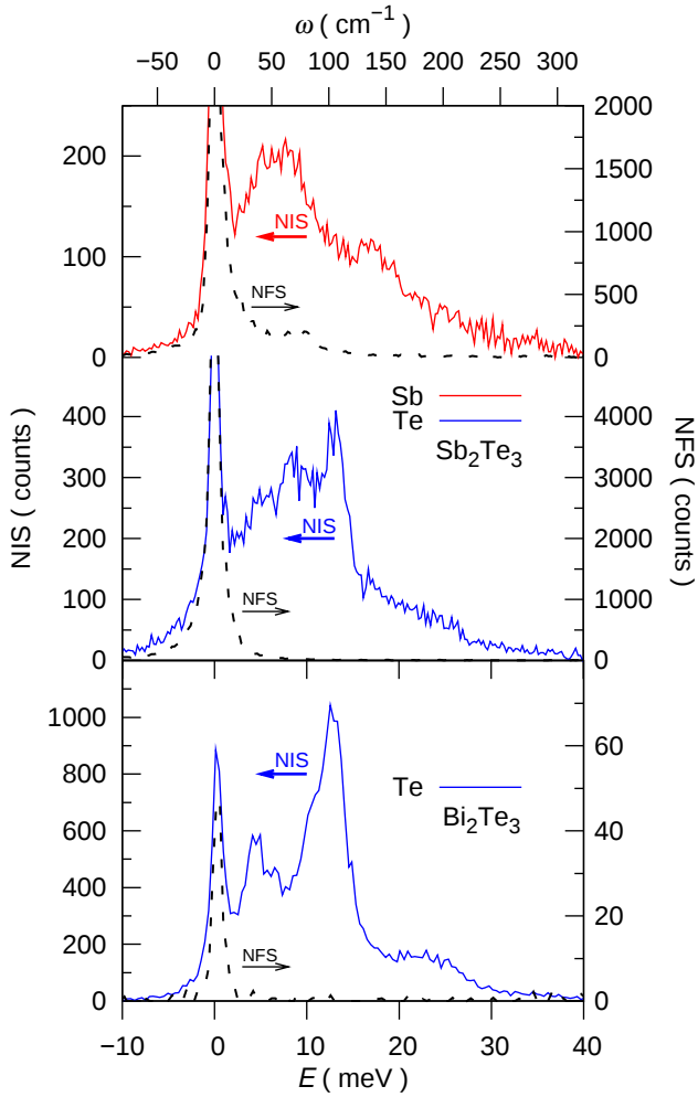
Figure 16: The Nuclear Inelastic Scattering, NIS, spectra (lines) and the time integrated nuclear forward scattering, NFS-instrumental function, (dashed lines) obtained with the ^{125}\text{Te} (blue lines) and the ^{121}\text{Sb} (red line) resonances on \text{Bi}_2^{125}\text{Te}_3 and \text{Sb}_2^{125}\text{Te}_3 .
