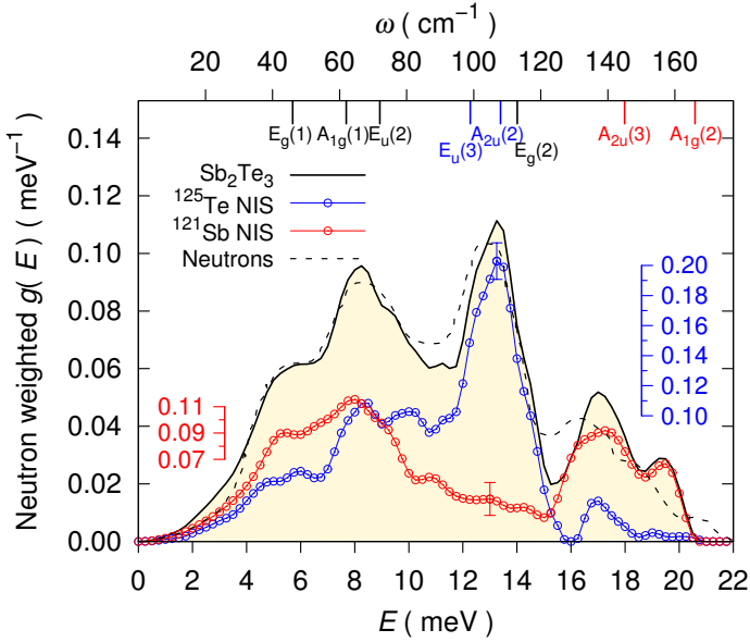
Figure 17: Density of Phonon States measured with the ^{125}\text{Te} (blue points) and ^{121}\text{Sb} (red points) resonance at 20 K on \text{Sb}_2\text{Te}_3 , for clarity line between points and typical errorbar is given. Comparison of the neutron weighted DPS of \text{Sb}_2\text{Te}_3 obtained with NIS (highlighted area), see text, with the one obtained using neutrons [85] (dashed line). Calculated [93] \Gamma -point phonon mode energies and symmetries are indicated by the labeled ticks.
