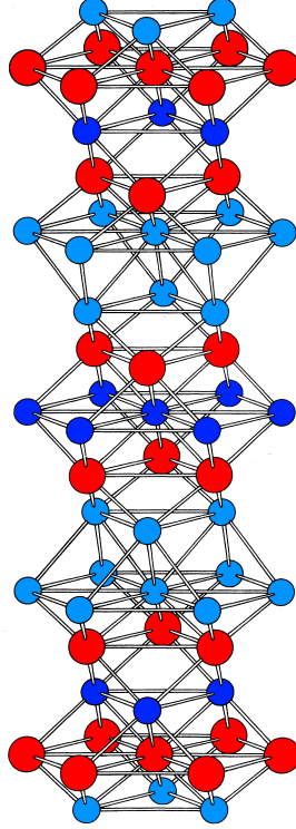
Figure 12: The tetradymite structure in which \text{Bi}_2\text{Te}_3 and \text{Sb}_2\text{Te}_3 crystallise. The blue balls stand for the Te atoms and the red for the Bi or Sb atoms, respectively. Figure is adapted from Ref. [58].
