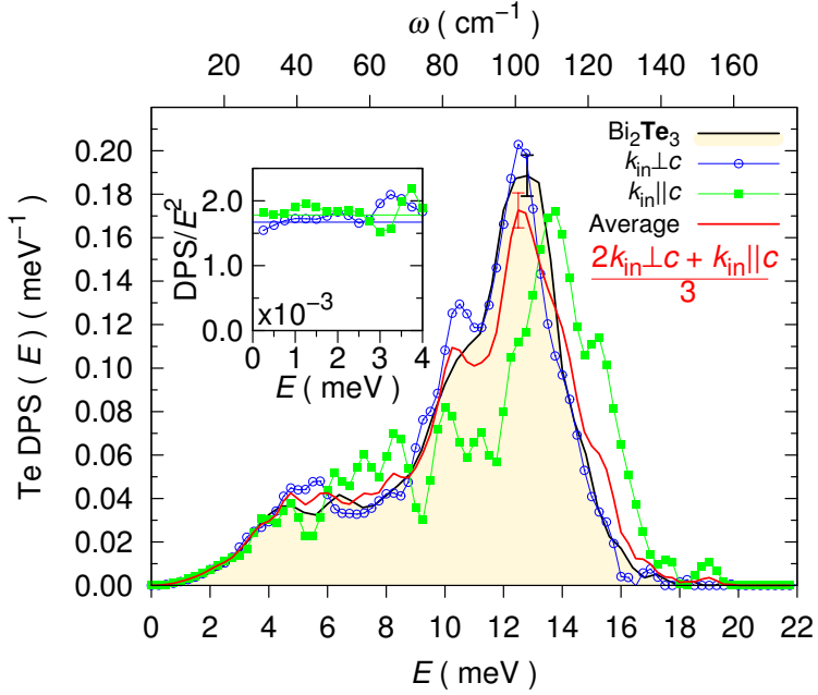
Figure 19: Orientation dependent Te DPS measured on a \text{Bi}_2\text{Te}_3 single crystal parallel (green squares), and perpendicular (blue circles), to the crystallographic c -axis. A comparison of the measured Te DPS in a \text{Bi}_2\text{Te}_3 polycrystalline sample (black curve) with the isotropic average obtained from data measured on single crystal (red curve) is given. Inset: Debye level calculated in the two orientations (solid lines) from the measured Te specific DPS.
