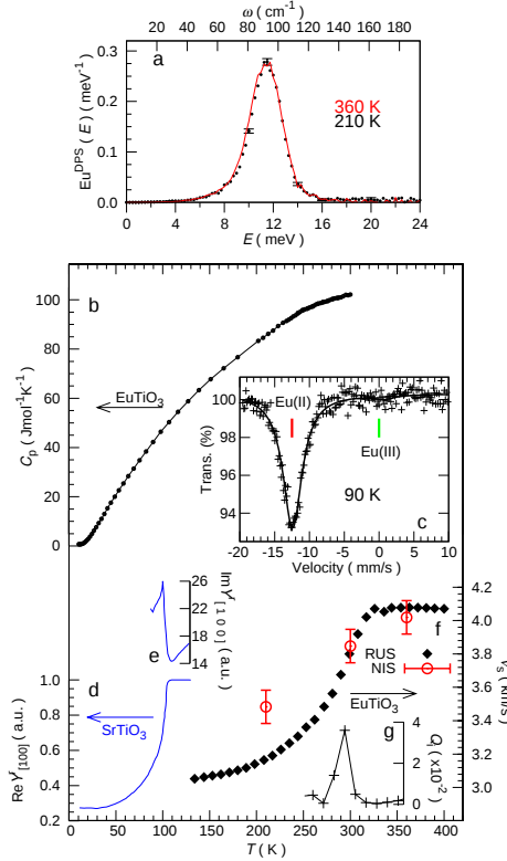
Figure 27: (a) The Eu specific density of phonon states in EuTiO 3 at 210 K (black ticks) and 360 K (red line-ticks) measured using NIS, typical errorbar is given. (b) Heat capacity data between 10 and 300 K measured on EuTiO 3 using calorimetry (pointsize defines errorbar), line between points is given as guide to the eye. (c) Mössbauer spectrum at 90 K (points) and the two component model (line). The positions of divalent and trivalent Eu are indicated. (d) The real part, \text{Re}Y_{[100]}^r (a.u.), of the complex Young's modulus in SrTiO 3 obtained from Ref. [182]. The imaginary part, \text{Im}Y_{[100]}^r , of the complex Young's modulus of SrTiO 3 obtained from the same reference is shown in (e). (f) Speed of sound extracted from RUS (black points), pointsize defines errorbar, and the corresponding extracted from NIS (red circles) at 210, 300 and 360 K. (g) The inverse quality factor of the resonance at 590 kHz between 250 and 350 K.
