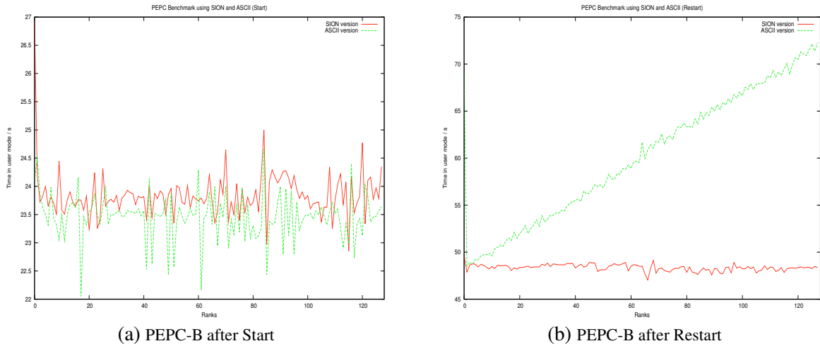
Figure 9: PEPC-B Benchmark on 128 CPUs
