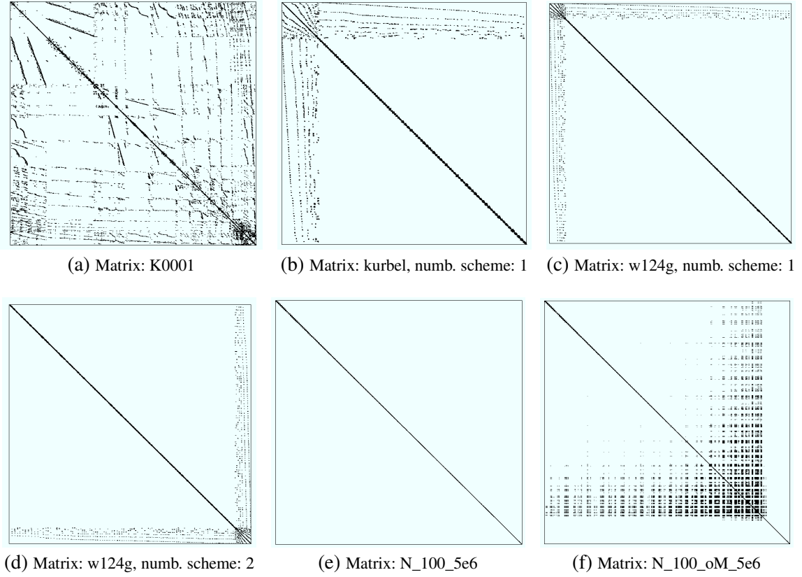
Figure 1: Structure plots of some of the used input matrices.
