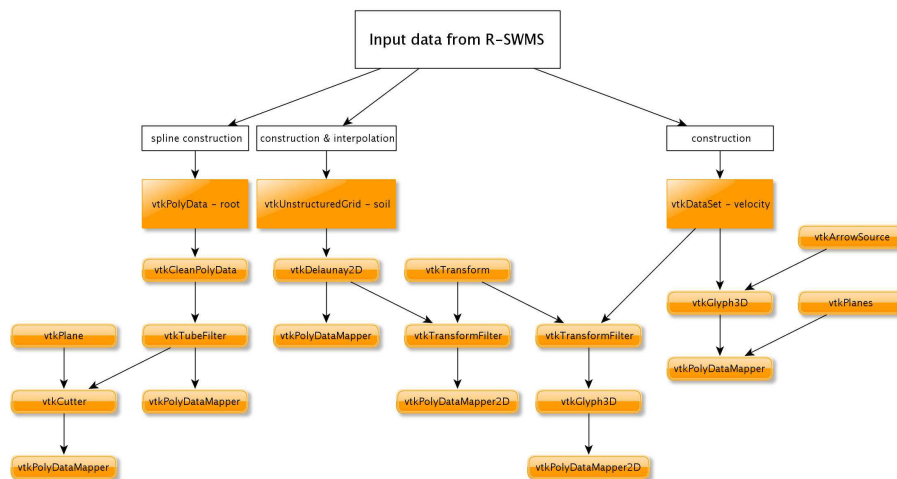
Figure 7: Reduced overview of the most important VTK pipeline segments in RSWMSViz
