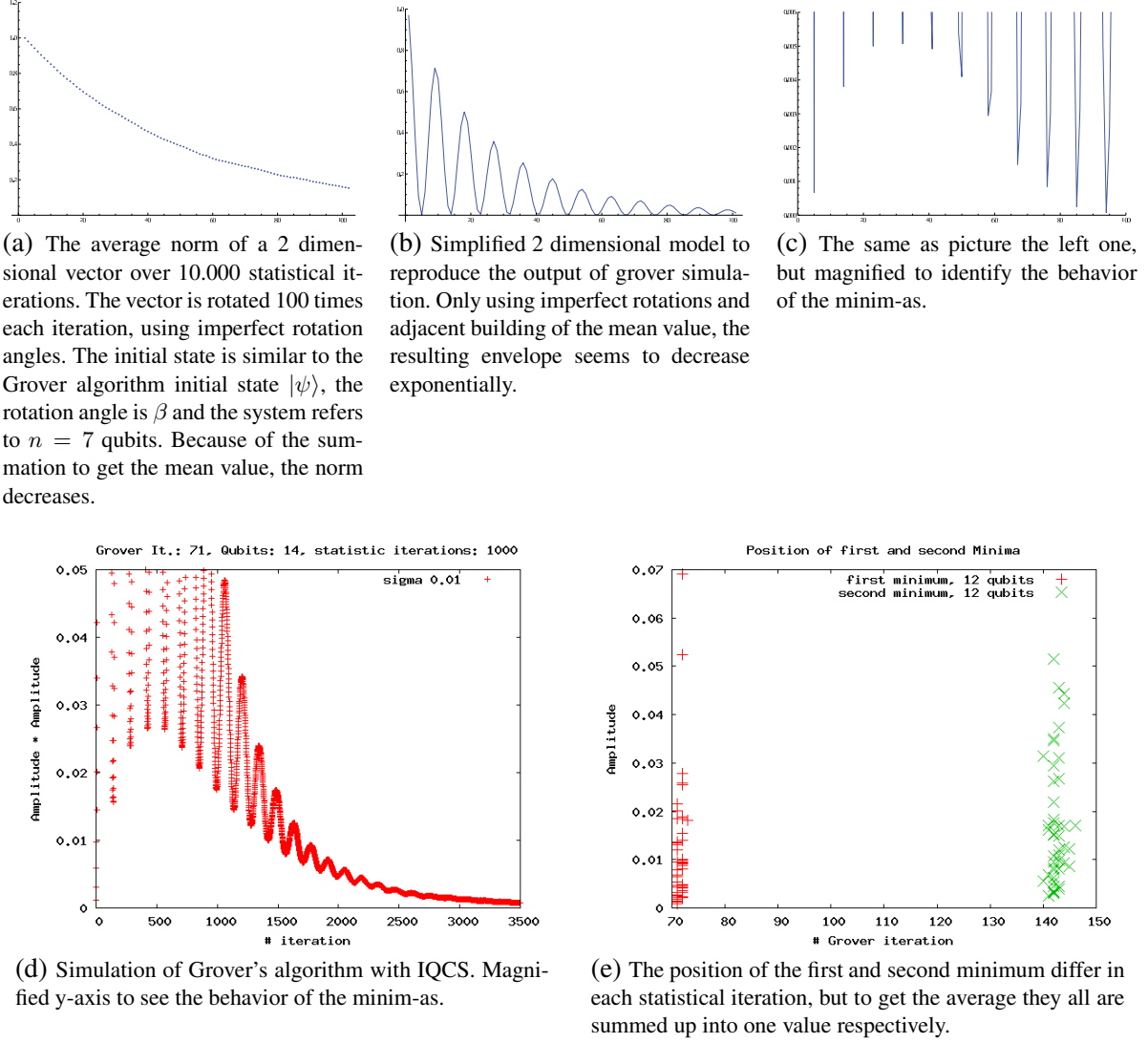
Figure 4: Plots analyzing statistical artifacts.
