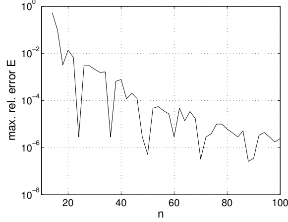
(a) For \alpha = 7.11 .
