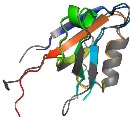
(b) The template 2OCS. The target 1G9O is depicted in grey for comparison.
