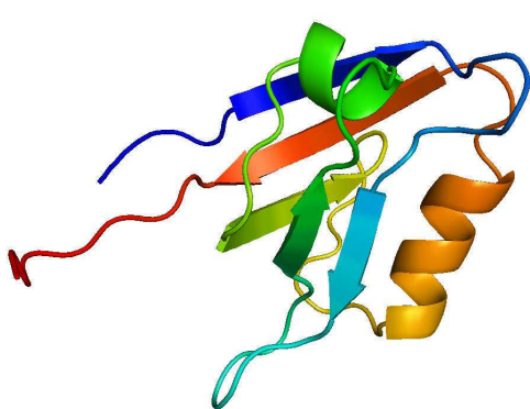
(a) The target 1G9O.
