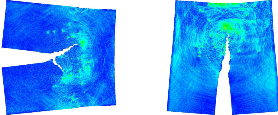
Figure 2: A mode I crack in a 2 dimensional Lennard Jones solid.
