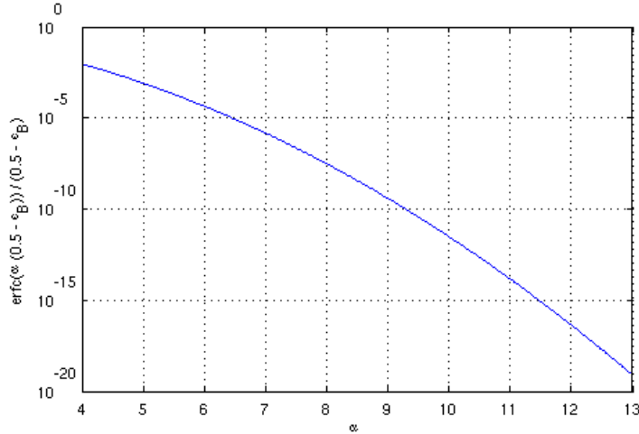
Figure 1: The function value of e_\alpha = K(\mathbf{x}) = \frac{\text{erfc}(\alpha \|\mathbf{x}\|)}{\|\mathbf{x}\|} for \mathbf{x} with \|\mathbf{x}\| = \frac{1}{2} - \varepsilon_B depending on \alpha .
