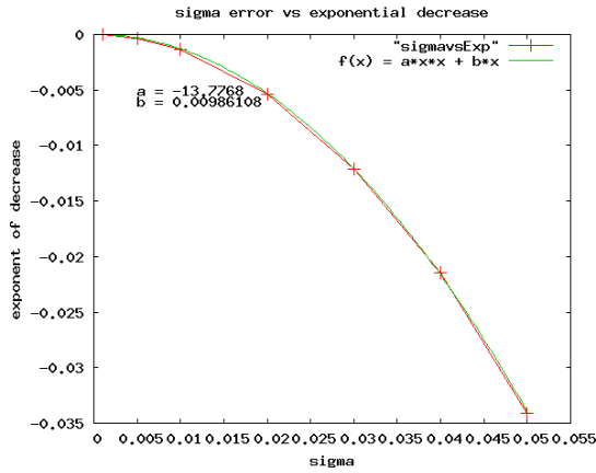
(c) Dependence of the exponent of decrease on the sigma parameter. The quadratic part of an polynomial interpolating function is highly exaggerated.
