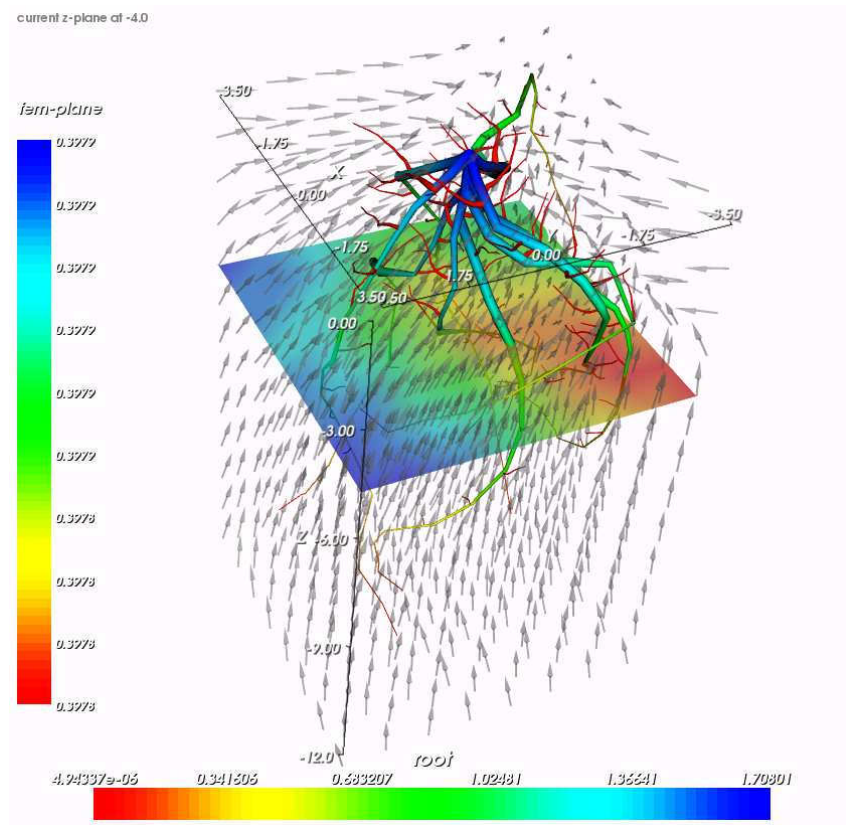
Figure 12: RSWMSViz graphical output showing root structure, vertical soil plane and velocity field
