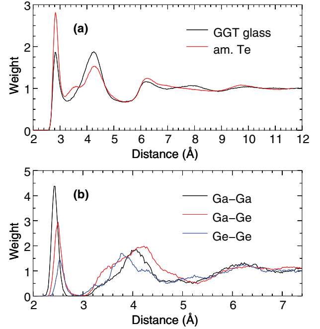
FIG. 4. (Color online) PDF of g -GGT: (a) Comparison of Te-Te PDF with DF-MD results for a -Te (Ref. 26), (b) PDF for Ga-Ga (black), Ga-Ge (red), and Ge-Ge (blue) for the MD simulations at 300 K. The corresponding coordination numbers are small (“wrong bonds”).
