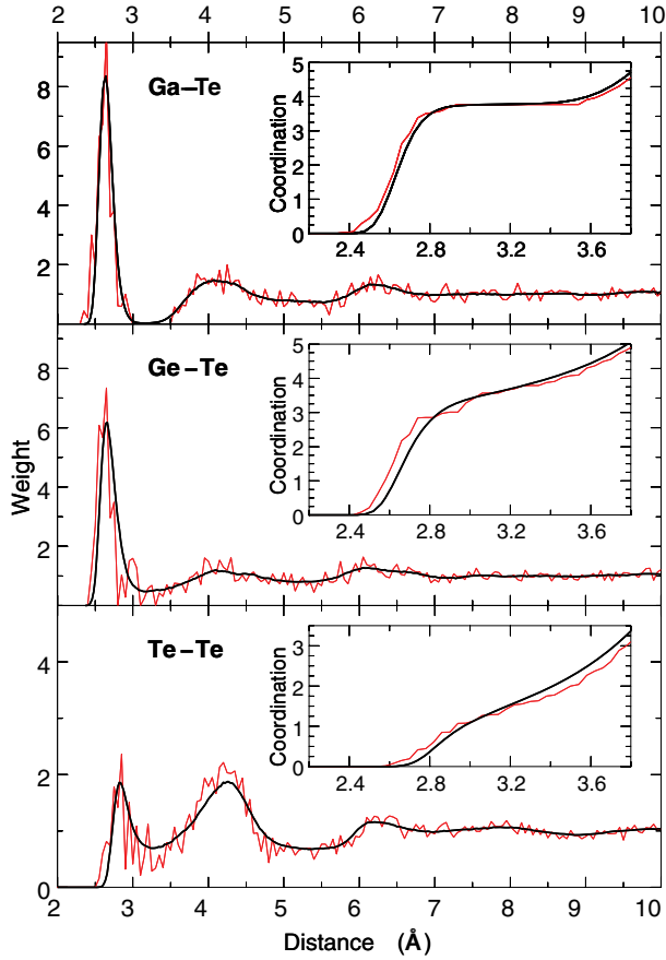
FIG. 3. (Color online) PDF of g -GGT for Ga-Te, Ge-Te, and Te-Te. Black, DF-MD simulation at 300 K (12 000 frames); red, RMC-refined structure (one frame). Insets: coordination numbers as a function of cutoff distance.
