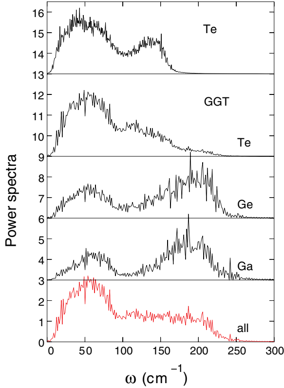
FIG. 9. (Color online) Vibrational density of states of a -Te at 300 K (top frame, Ref. 26) and of g -GGT at 300 K with projections onto elements. All curves have the same maximum.
