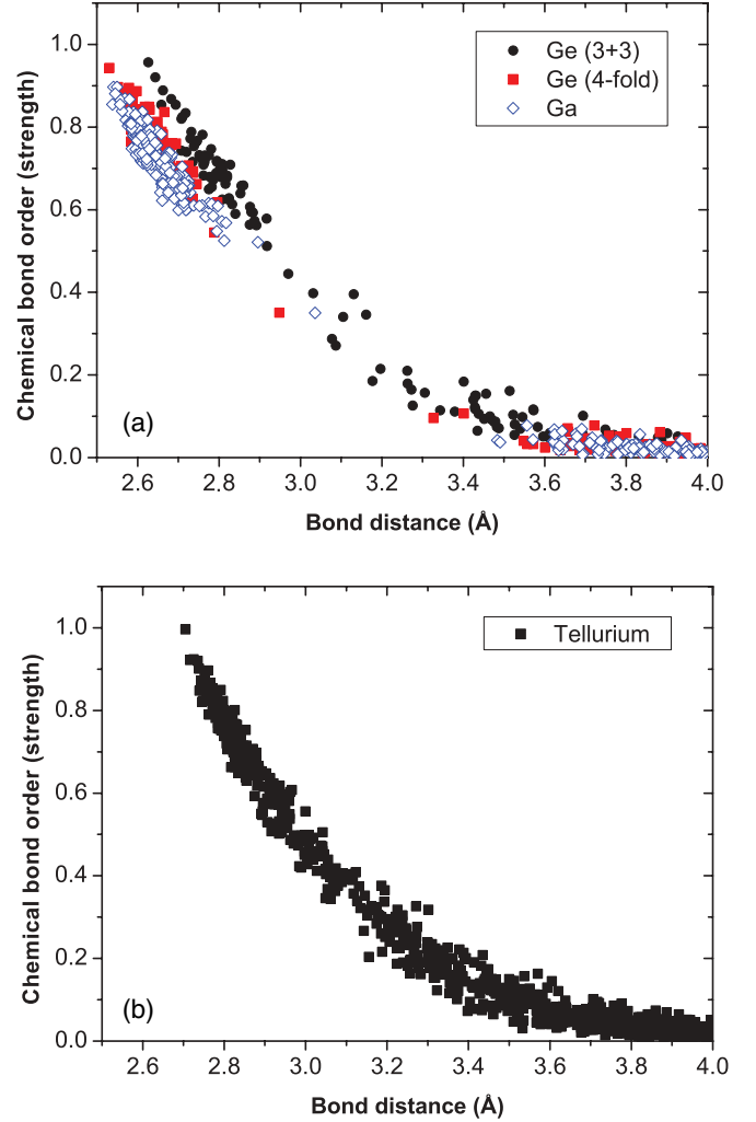
FIG. 8. (Color online) (a) Chemical bond orders (strengths) as a function of distance for (a) Ga-Te and Ge-Te bonds, and (b) Te-Te bonds.
