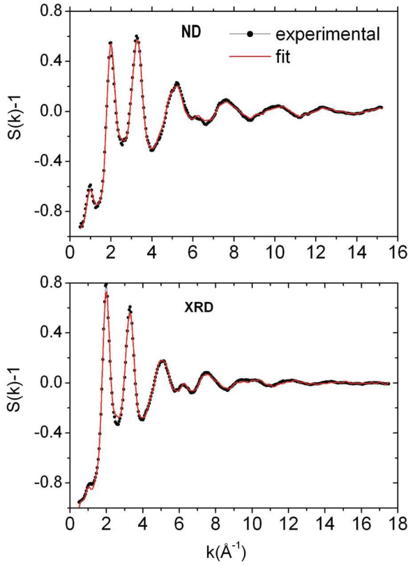
FIG. 1. (Color online) Experimental measurements of ND and XRD structure factors of glassy GGT (g-GGT) compared with the RMC-refined model (540 atoms).
