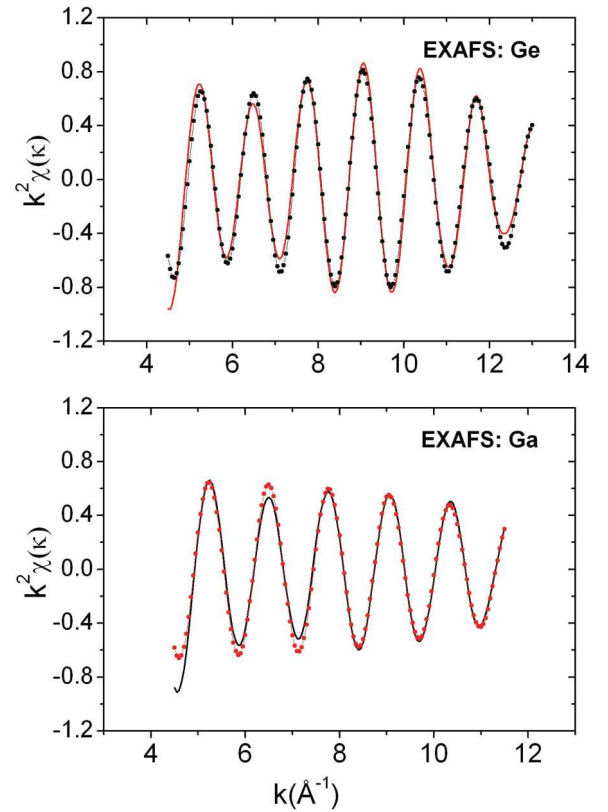
FIG. 2. (Color online) Experimental Ge and Ga K -edge EXAFS spectra of g-GGT compared with the RMC-refined model (540 atoms).
