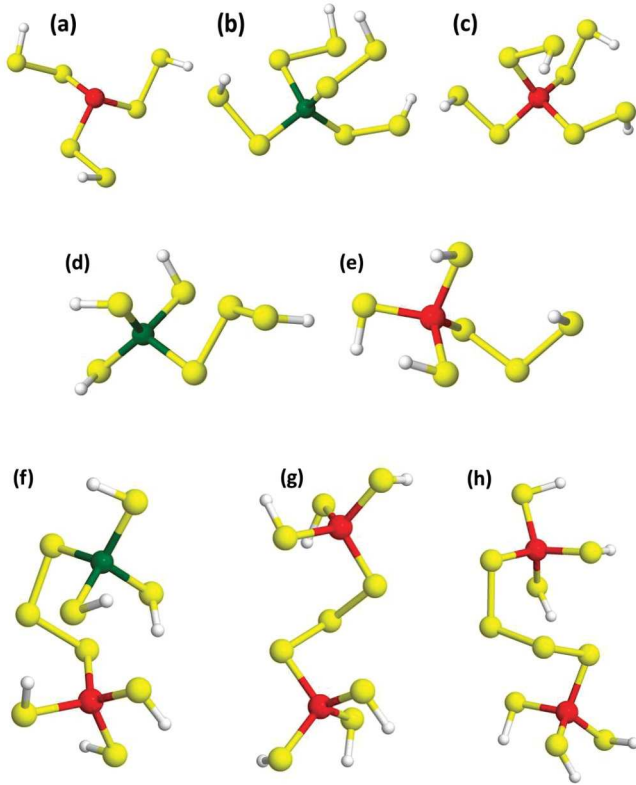
FIG. 11. (Color online) DF-optimized geometries of selected Ga-Ge-Te clusters with H termination. The labels correspond to Table IV.
