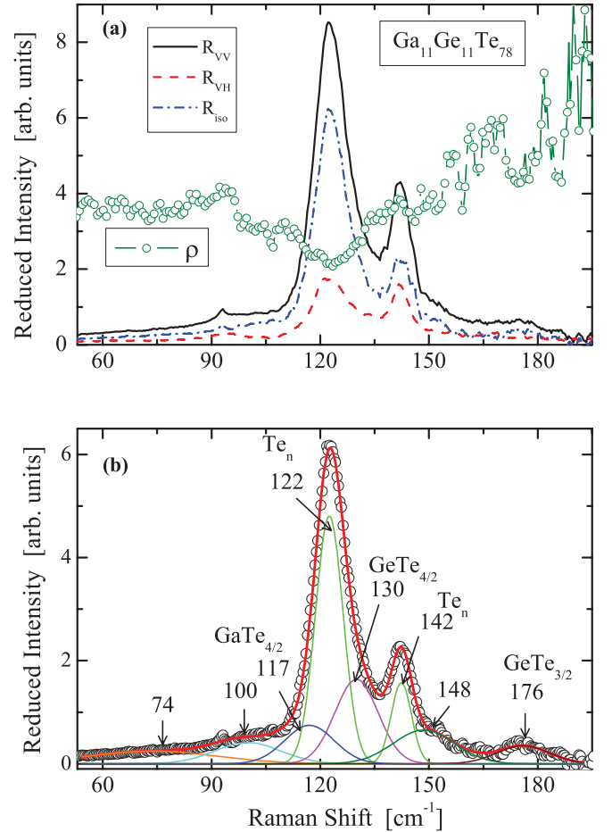
FIG. 12. (Color online) Reduced Raman spectra of g-GGT. (a) Polarized and isotropic [I_{VV} - (4/3)I_{VH}] Raman spectra and frequency dependence of the depolarization ratio \rho . (b) Decomposition of the reduced isotropic spectrum.
