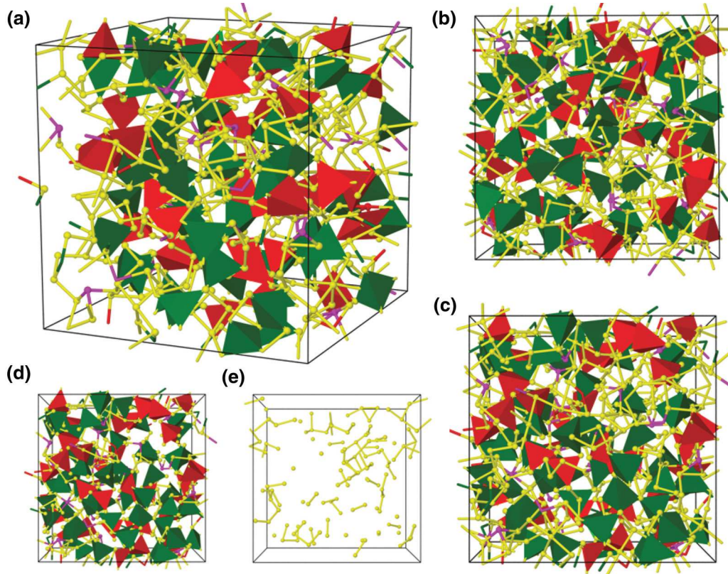
FIG. 6. (Color online) Glassy GGT: (a)–(c) From three perspectives, (d) atoms in Ga/Ge network (side view), and (e) Te atoms not bonded to Ga/Ge network (side view). Color code: Ga, green polyhedra; Ge (tetrahedral), red polyhedra; Ge (defective octahedral), magenta; and Te, yellow.
