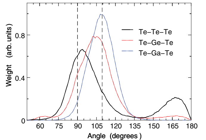
FIG. 5. (Color online) Angular distribution functions of g -GGT at 300 K (DF-MD simulation): Te-Ga-Te, Te-Ge-Te, and Te-Te-Te configurations. The dashed lines denote the octahedral (90°) and tetrahedral (109.47°) reference values.
