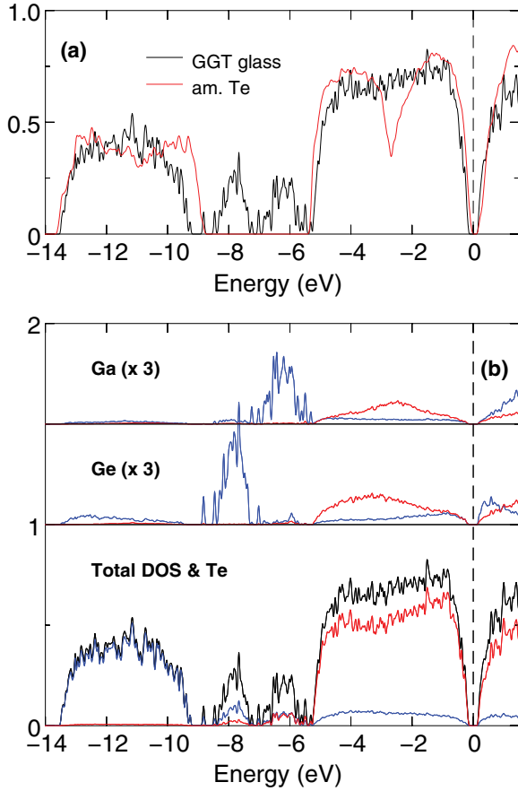
FIG. 7. (Color online) (a) Density of states of a -Te (Ref. 6) and g -GGT. (b) Projected density of states (DOS) of g -GGT. Blue, s , and red, p components. The scales for the Ga and Ge components are three times larger than for Te to compensate for the lower concentration.
