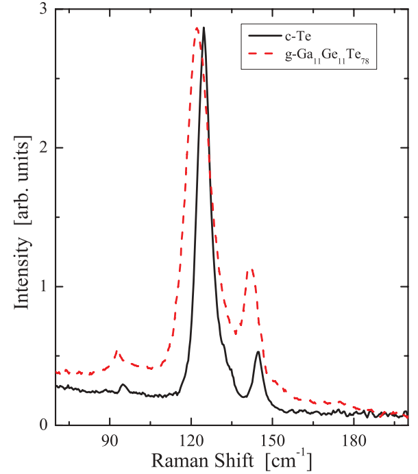
FIG. 10. (Color online) Unpolarized Stokes-side Raman spectra of g -GGT and c -Te.
