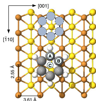
FIG. 1. (Color online) Ball and stick model of the Cu(110) surface and the benzene molecule. For better visibility, the second layer atoms of the copper surface are displayed in a lighter color (gray) compared to the first layer atoms. The so-called “long-bridge” site between two rows of the first layer Cu atoms has the lowest adsorption energy. The hexagonal structure in the upper part of the image indicates the so-called “hollow-site” position, which has a slightly higher adsorption energy. In the AFM simulations, we approached Si- and Cu-terminated tips at three different sites on the benzene molecule marked by A (on top of a carbon atom), B (carbon atom in “ortho” position to A), and C (center of the carbon ring). With a clean silicon tip, the molecule can easily be pushed along the [110] direction.
