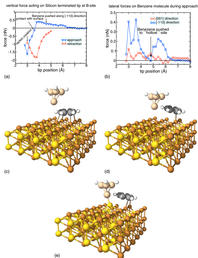
FIG. 2. (Color online) (a) Vertical force on the tip during approach and retraction for the clean silicon tip at the B site (see Fig. 1). The arrows mark the selected events shown in the ball and stick models. (b) Lateral forces acting on the benzene molecule along the [110] and [001] directions during the approach of the clean silicon tip. The arrow marks the tip position directly after the jump of the benzene molecule from the long-bridge to the hollow site. Here, the lateral force is initially zero. (c) During the approach, the benzene molecule is pushed along the [110] direction. (d) As the benzene molecule is moved away, the tip comes in direct contact with the Cu surface. (e) Finally, as the tip is pushed into the surface, an atomic defect is generated in the Cu surface.
