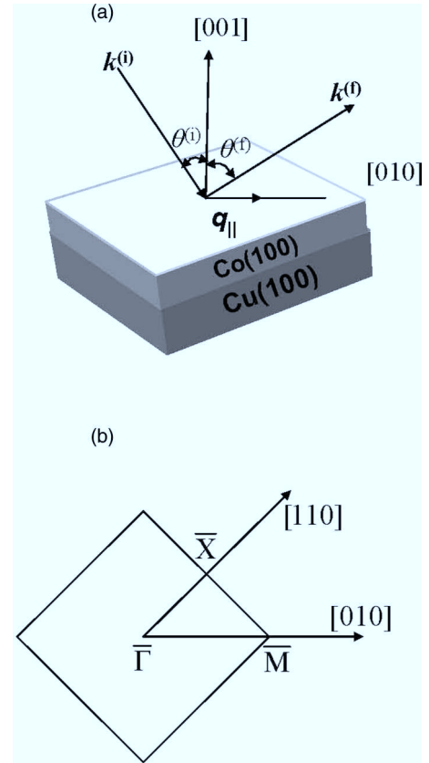
FIG. 1. (a) Schematic illustration of the scattering geometry used in our experiments. For all measurements, the angle between \mathbf{k}^{(i)} and \mathbf{k}^{(f)} , i.e., the scattering angle, is kept constant at 90°. (b) Surface Brillouin zone (SBZ) of the fcc(100) surface with the high-symmetry directions \bar{\Gamma}\bar{X} and \bar{\Gamma}\bar{M} indicated.
