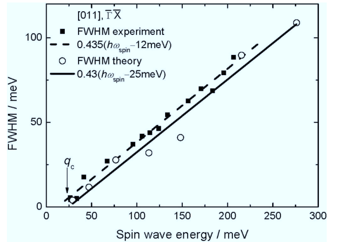
FIG. 11. Full width at half maximum (FWHM) of the spin wave peak vs the spin wave energy. Solid squares are the experimental data from Fig. 9, the open circles are from theory. When fitted to a linear relation the theoretical results follow the same slope. See text for further discussion.
