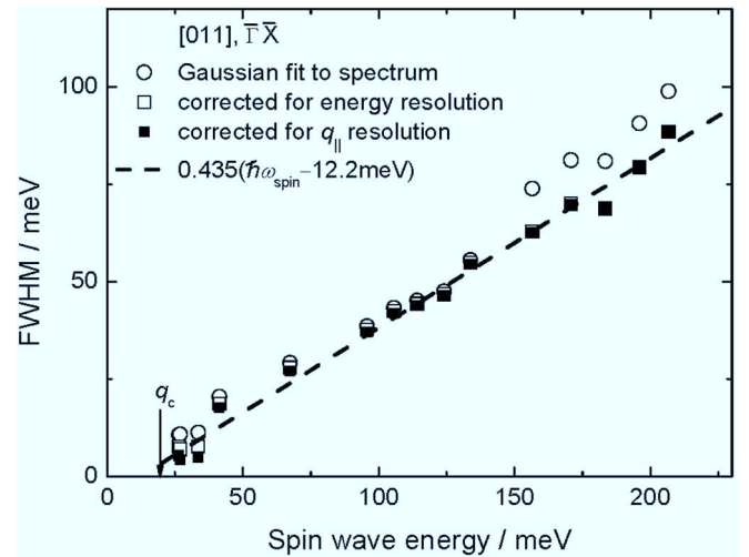
FIG. 9. Determination of the true FWHM of the spin wave peak from experimental spectra. Up to q_{\parallel} = 0.66 \text{ Å}^{-1} ( \hbar\omega \sim 130 \text{ meV} ) experimental spectra have been obtained with an energy resolution of 7 \text{ meV} FWHM. The variance of the distribution of accepted angles was s_\alpha = 0.015 . For larger q_{\parallel} , the energy resolution was 34 \text{ meV} and s_\alpha = 0.045 . The circles give the experimental FWHM. The open squares represent the values after correction for the energy resolution. The solid squares are obtained after the additional correction for the kinematic broadening. The data are plotted versus the spin wave energy. The dashed line is a linear fit to be discussed later.
