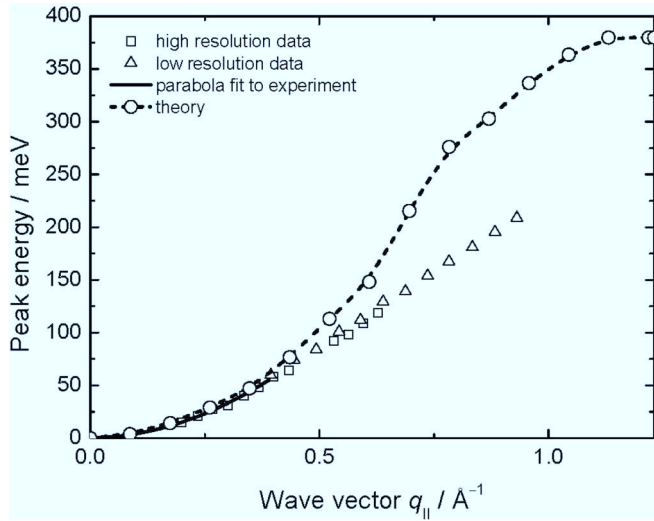
FIG. 10. Comparison of the theoretical dispersion (open circles) with experimental data (open squares and triangles).
