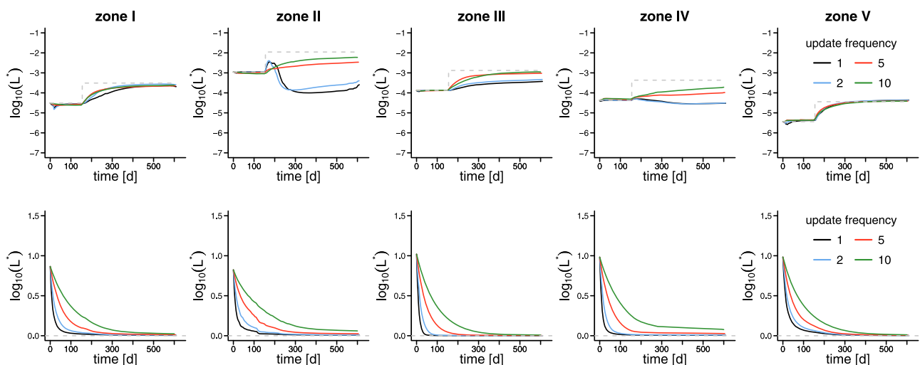
Figure 13. Temporal evolution (period January 2004–August 2005) of ensemble mean (upper row) and ensemble standard deviation (lower row) of zonal leakage coefficients for different updating frequencies of hydraulic heads and leakage coefficients (simulation scenario A).
