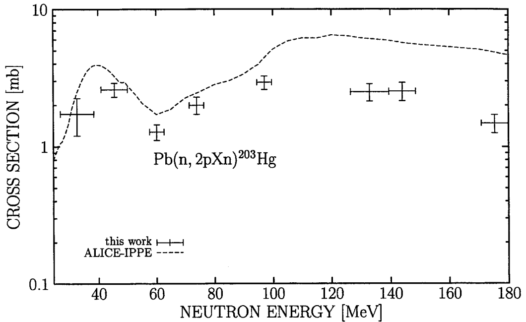
Fig. 2: Guess excitation function and final cross sections for the reaction ^{nat}\text{Pb}(n,2pxn)^{203}\text{Hg} . The uncertainties in energy given represent the half-width of the peak in the neutron spectrum.
