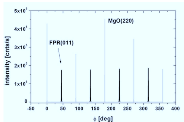
FIG. 3. Phi scans showing the \text{Fe}_{50}\text{Pt}_{40}\text{Rh}_{10} (011) and MgO (220) reflections. The scans reveal a 45° offset between film and substrate.
