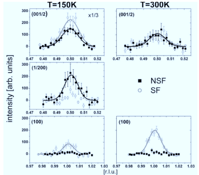
FIG. 6. Polarized neutron-diffraction scans of the (00\frac{1}{2}) , (\frac{1}{2}00) , and (100) AF reflections at 150 and 300 K plotted against the individual reciprocal-lattice units (RLUs). The data sets of the (00\frac{1}{2}) reflection have been multiplied by a factor of 1/3 .
