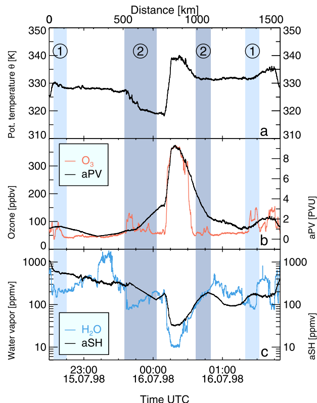
Figure 2. Time series for the flight on July 15, 1998. (a) Potential temperature (b) in-situ ozone (red line) and analyzed PV (from ECMWF, black line), (c) in-situ total water (blue line) and analyzed SH (from ECMWF, converted to ppmv, black line). Grey shaded areas mark four time ranges (on constant pressure levels) in regions 1 and 2 where strong tracer gradients were observed.
