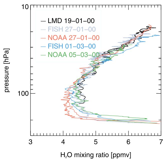
Figure 1. \text{H}_2\text{O} profiles measured during SOLVE/THESEO-2000 on 19 January, 27 January, 1 March, and 5 March 2000.
