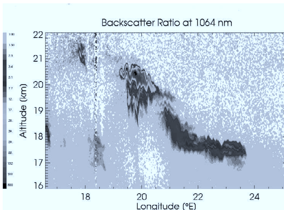
Figure 6. Lidar measurements of aerosol backscatter ratio at 1064 nm along the wind flow at PSC level measured from the Falcon aircraft on 27 January 2000. The backscatter ratio, defined as the ratio of the total backscatter coefficient (particles and molecules) to the molecular backscatter coefficient, is given in logarithmic scaling. See color version of this figure at back of this issue.
