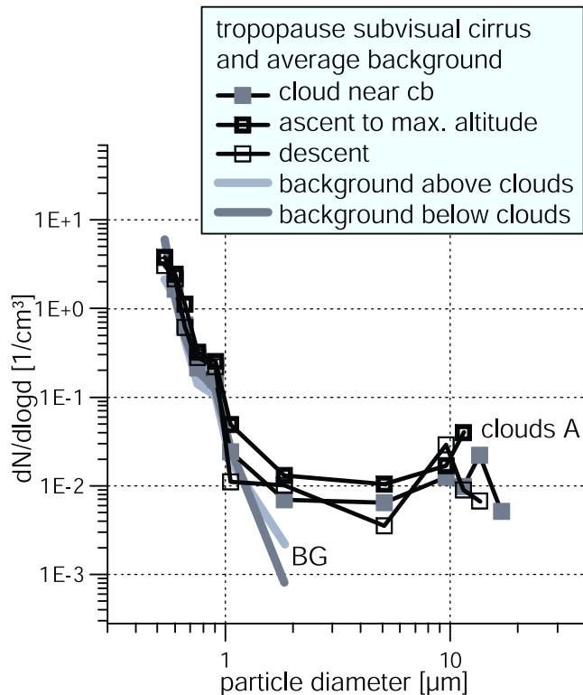
Figure 4. Size distributions of the subvisual cloud layer (labeled as “A” in Figure 3) at the tropical tropopause near 17 km. Due to counting statistics, the three curve segments do not significantly differ from each other at sizes above 2 \mu\text{m} . The curves labeled “BG” correspond to background aerosol measurements outside of (but close to) the cloud.
