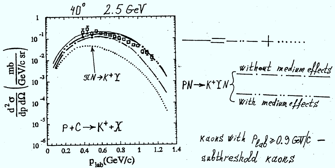
Fig. 7. Double differential cross sections for the production of K^+ mesons at an angle of 40^\circ in the interaction of 2.5 \text{ GeV} protons with the C^{12} nuclei as functions of kaon momentum.
