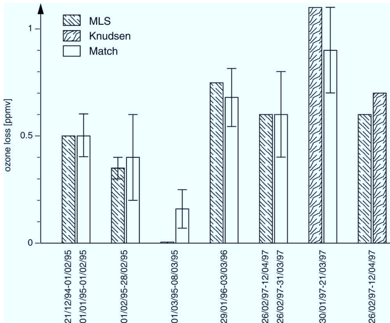
Figure 2. Comparison of accumulated losses in ozone mixing ratio derived from MLS [Manney et al. , 1996a, 1996b, 1997], Match [Rex et al. , 1997, 1999; Schulz et al. , 2000] and the vortex average approach [Knudsen et al. , 1998] at potential temperatures around 475 K. In each pair, the Match ozone loss rates have been integrated for the same time period and in the same subsiding air mass to allow direct comparisons.
