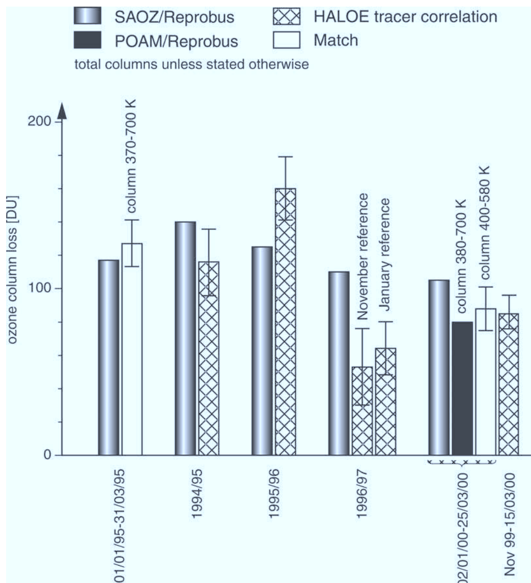
Figure 3. Comparison of column ozone losses derived from the SAOZ/REPROBUS [Goutail et al. , 1998, 1999]; POAM/REPROBUS [Deniel et al. , 1998]; Match [Rex et al. , 1999, 2001]; and HALOE tracer correlation [Müller et al. , 1996, 1997a, 1999; R. Müller et al. , Chemical ozone loss and chlorine activation deduced from HALOE and OMS measurements in the Arctic winter 1999–2000, manuscript in preparation, 2002; S. Tilmes et al. , Calculation of chemical ozone loss in the Arctic winter 1996/1997 using ozone-tracer correlations: Comparisons of ILAS and HALOE results, manuscript in preparation, 2002] approaches. The 1996/1997 January estimate uses ILAS data for the initial relation, and the 1999/2000 uses a mix of tracer data from the OMS remote and in situ balloon payloads that flew in November 1999. In both years the March relations used were found from HALOE data.
