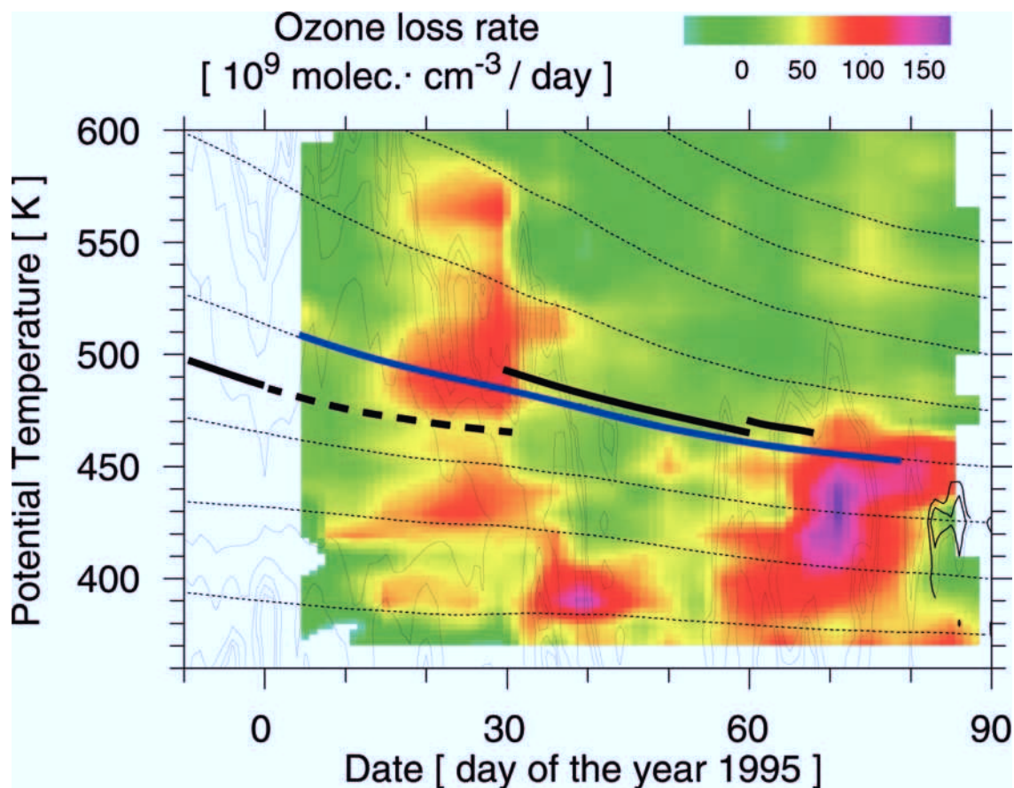
Figure 1. Ozone loss rates found by Match in the 1994/1995 Arctic winter [Rex et al. , 1999]. The thick black lines show the subsiding air masses observed during the three periods for which an accumulated ozone loss is reported using MLS data [Manney et al. , 1996b]. The thick solid lines represent continuous periods of MLS observations, while the thick dashed line represents the air mass linking the final measurements in one north looking period of MLS with the early measurements in the next period. The solid blue line indicates the subsiding air mass closest to the air masses observed by MLS, and the dashed black lines indicate the paths of other subsiding air masses. In this study, the Match ozone loss rates are integrated along the thick black lines to allow a direct comparison with the MLS-derived losses. The isolines drawn with thin solid black lines show the area below PSC existence temperatures.
