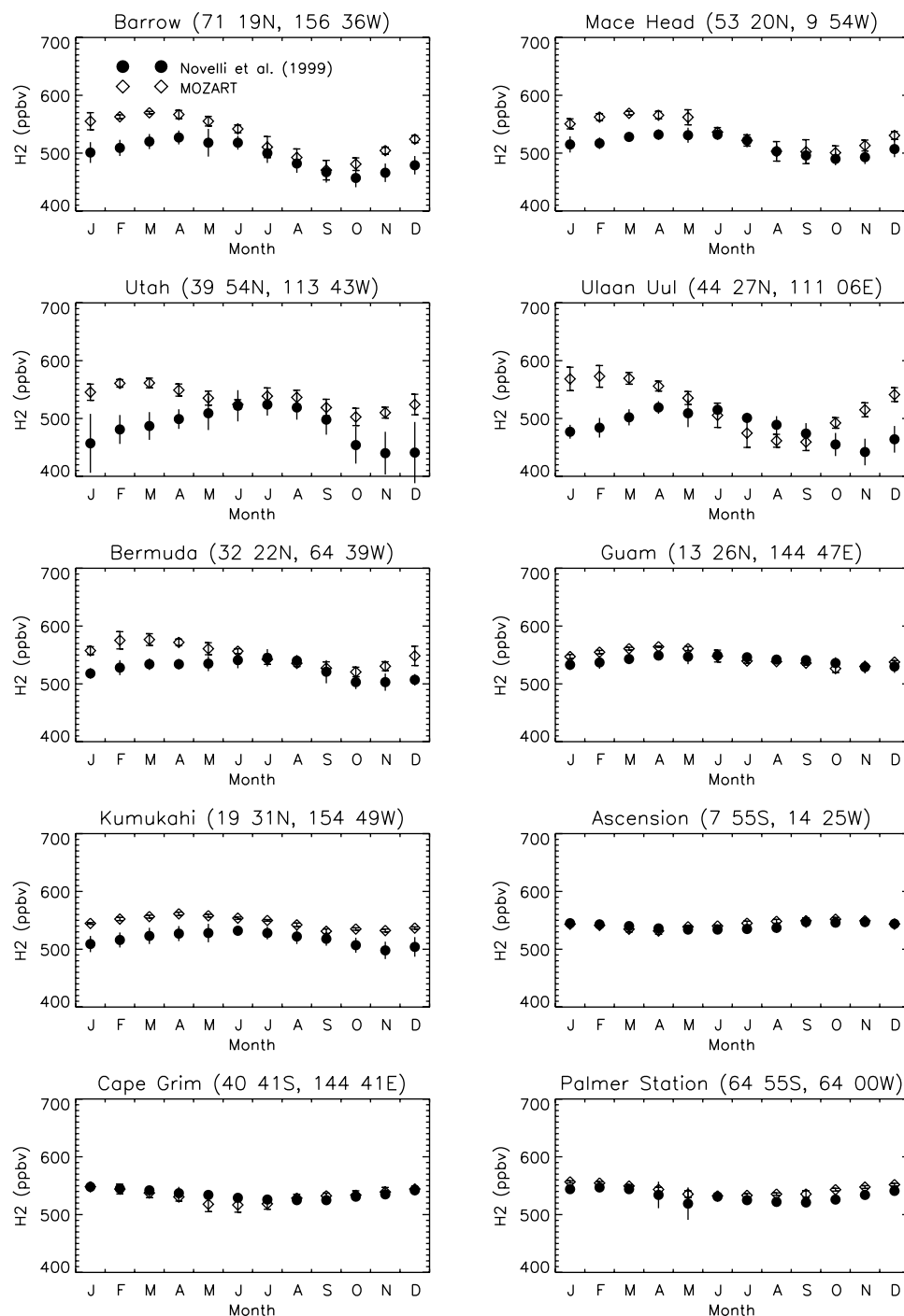
Figure 11. Modeled (diamonds) and measured (dots) seasonal variations in the H 2 mixing ratio at the Earth's surface for a number of stations at different latitudes. The stations Utah and Ulaan Uul are continental; all others are coastal or insular. The error bars indicate the mean standard deviation. Measurements are from Novelli et al. [1999].
