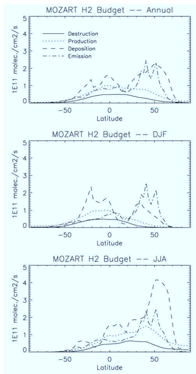
Figure 4. Latitudinal variation of \text{H}_2 photochemical production, destruction, surface emission, and surface deposition ( 10^{11} molecules/ \text{cm}^2/\text{s} ) calculated for annual mean, December–January–February (DJF), and June–July–August (JJA) conditions.
