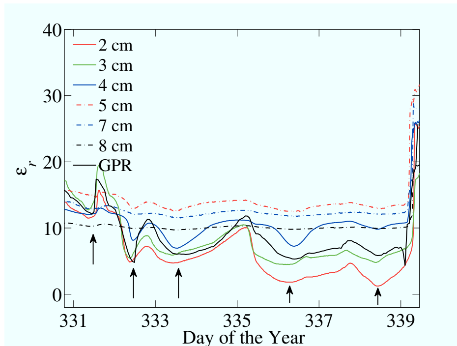
Figure 6. Time series of the relative permittivity ( \epsilon_r ) of the soil recorded at shallow depths (2, 3, 4, 5, 7, 8 cm) and estimated from time-lapse GPR data. Five freezing and thawing cycles can be clearly observed over a period of nine days, as indicated by arrows.
