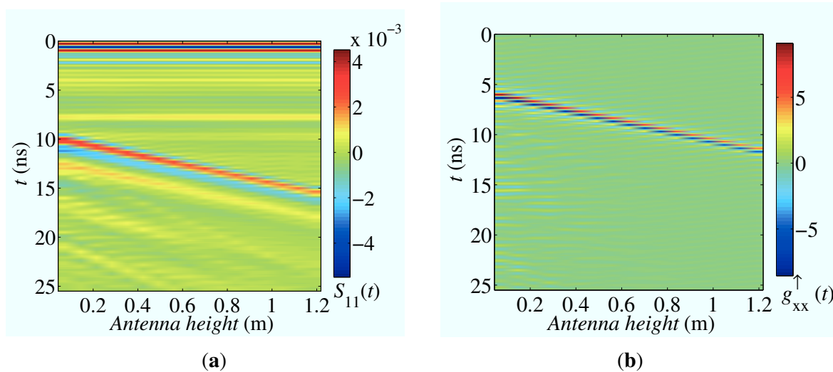
Figure 4. Time domain representation (b-scan) of radar measurement performed with the horn antenna at different heights above a perfect electrical conductor (copper sheet). (a) Measured raw GPR signal S_{11}(t) and (b) the filtered signal g_{xx}^{\uparrow}(t) using the antenna model.
