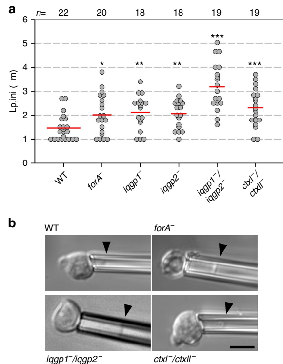
Figure 5 | ForA is required for cortical integrity. (a) Initial projection length L p,ini of wild-type and mutant cells determined by MPA using a constant suction pressure of 500 Pa. Red lines, mean values. n , number of analysed cells. *** P ≤ 0.001; ** P ≤ 0.01; * P ≤ 0.05 (Mann-Whitney U -test). Statistical differences refer to wild type. (b) Development of projections (black arrowheads mark menisci) after 145 s in representative samples. Scale bar, 10 \mu m.
