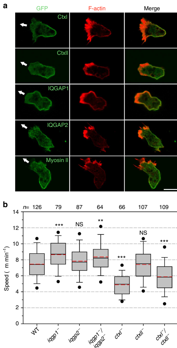
Figure 4 | Ctx and the IQGAPs localize like myosin II to the rear and affect cell migration. (a) The proteins indicated were expressed as GFP fusions in the respective knockout mutants, fixed and labelled with Atto488-conjugated nanobodies (green) to enhance the GFP signal. Filamentous actin was stained with rhodamine phalloidin (red). The white arrow marks the direction of cell movement. Scale bar, 10 \mu m. (b) Quantitative analysis of random cell motility of iqgp - and ctx - mutants in unconfined environments. n , number of tracked cells. *** P ≤ 0.001; ** P ≤ 0.01; NS, not significant (Mann-Whitney U -test). Statistical differences refer to wild type.
