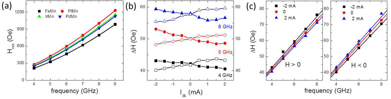
FIG. 3. (Color online) (a) Resonance field versus frequency and the corresponding Kittel fit for different antiferromagnetic sample stacks. (b) and (c) Resonance linewidth ( \Delta H ) versus dc-bias current ( I_{dc} ) at different frequencies, f = 4, 5 , and 6 GHz [dc current polarity: solid (+), empty (-)], and resonance linewidth versus frequency at different dc-bias currents, I_{dc} = -2, 0 , and 2 mA, for PtMn(10)/Py(5).
