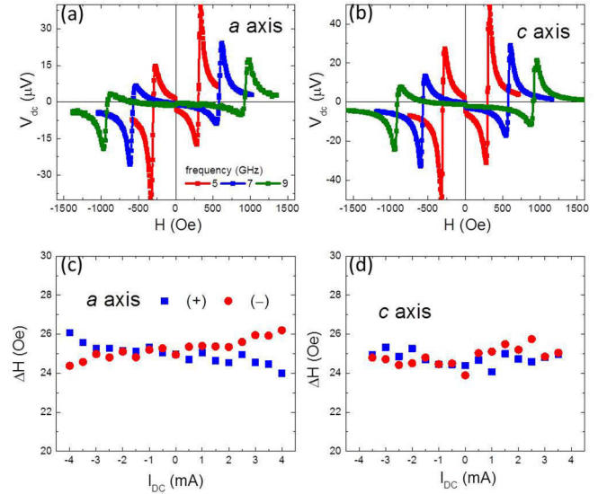
FIG. 6. (Color online) Measured spin-torque ferromagnetic resonance signals from (a) a - and (b) c -axis PtMn(10)/Cu(1)/Py(5), and (c,d) the corresponding resonance linewidth versus dc-bias current at 5 GHz.
