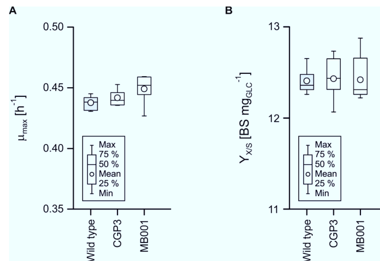
Figure 3.9: Phenotyping of the first generation of genome-reduced C. glutamicum strains in the BioLector on CGXII medium with 20 g l -1 D-glucose. (A) Maximum growth rate of CGP3 and MB001 compared to the wild type (n=7). (B) Biomass yield of CGP3 and MB001 compared to the wild type (n=7).
