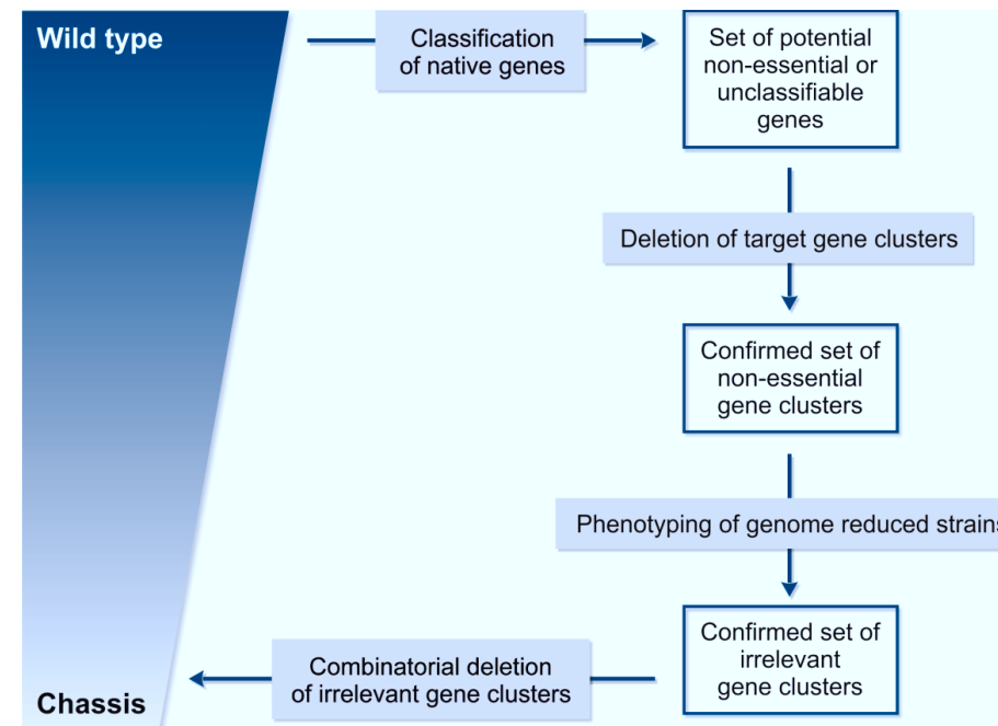
Figure 1.2: Outline of the targeted top-down approach followed in this work to construct a chassis organism based on the C. glutamicum wild type ATCC 13032 - modified from Unthan et al. 2014 [4].
