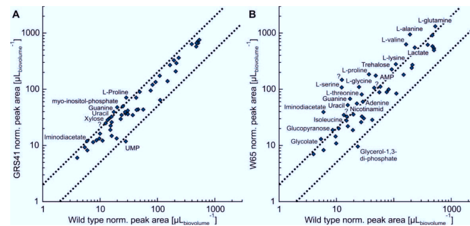
Figure 3.15: Intracellular GC-ToF-MS fingerprint of GRS41 (A) and W65 (B) compared to the C. glutamicum wild type. Strains were grown in 1 l bioreactors on defined CGXII medium and sampling was performed during exponential growth phase. The resulting peak areas for all detectable metabolites were normalized by the total biovolume in each sample. Dashed lines represent levels of 2-fold increased or decreased values compared to the wild type. Metabolites which could not be identified using the JuPOD database are labeled with a question mark.
