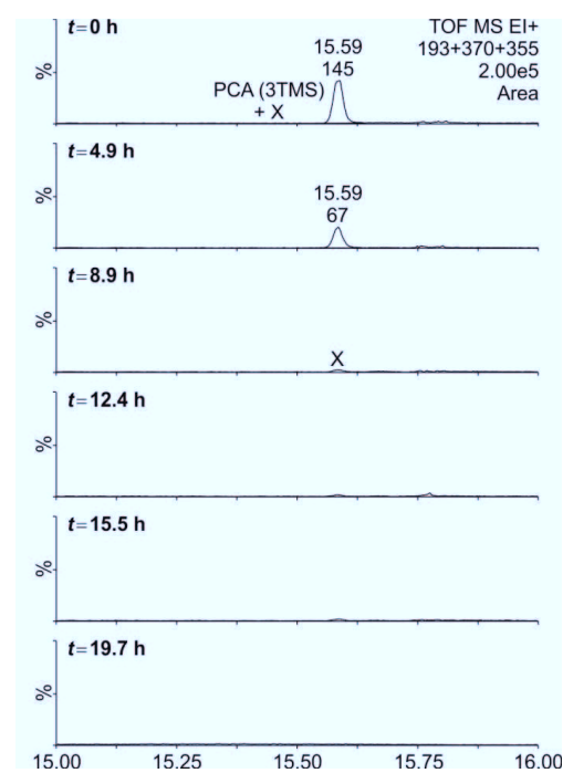
Figure S-2: Selected chromatograms from untargeted metabolome screening of culture supernatant samples from batch cultivations of C. glutamicum on CGXII glucose medium. The iron-chelator PCA decreased during the first growth phase and was already absent at the switch to the second phase - modified from Unthan et al. 2014 [2].
