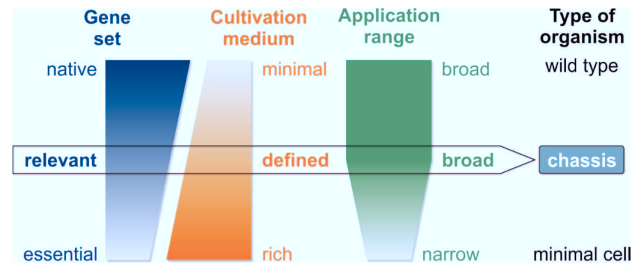
Figure 1.1: Definitions referred to in this work considering types of organisms and the underlying interplay of their gene set, cultivation medium and application range - modified from Unthan et al. 2014 [4].
