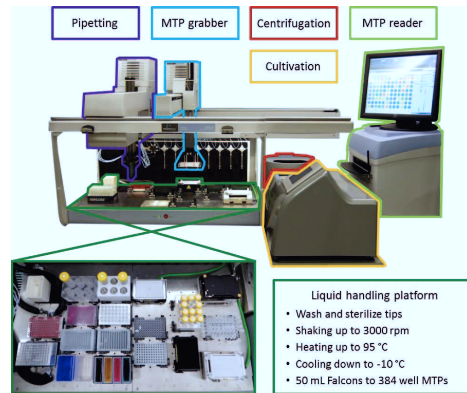
Figure 1.3: Setup of the mini pilot plant (MPP) used in this work. The Janus workstation liquid handling platform was extended by devices for shaking, incubation, microtiter scale cultivation, centrifugation and photometric analysis.
