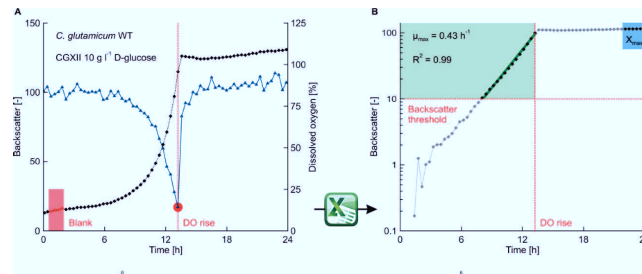
Figure 3.6: Standardized processing of BioLector data in an Excel routine for analysis of large strain libraries. (A) Exemplary raw data of backscatter (gain 20) and dissolved oxygen measurement during a 24 hour cultivation of the C. glutamicum wild-type. (B) During automated data analysis, each backscatter curve was first blanked by its initial values (red box). Then a backscatter threshold and the rise in the DO signal were used to trim the data and estimate the maximum specific growth rate from the exponential growth phase (green box). X_{max} was determined from the blanked backscatter values of the last two hours (blue box) and normalized by the applied substrate mass to estimate biomass yields.
