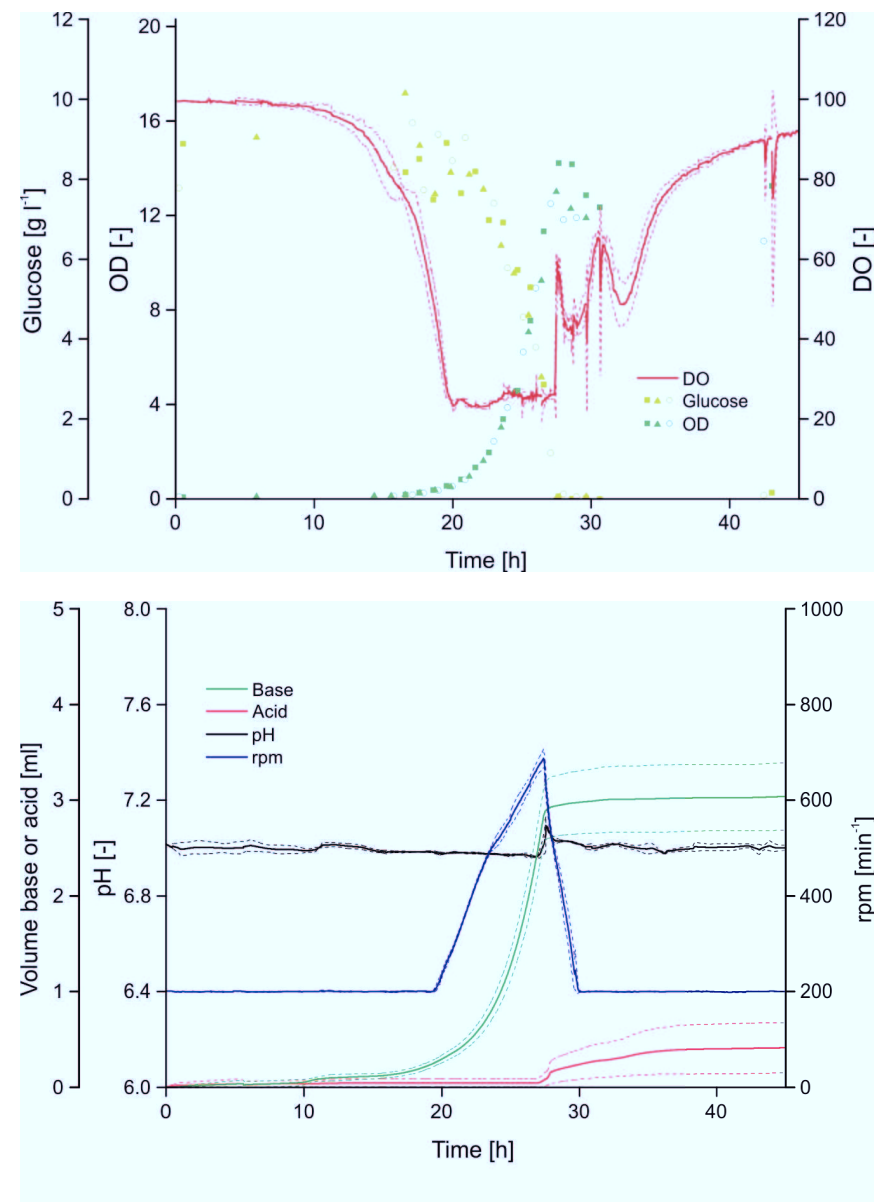
Figure S-7: Cultivation of pre-chassis W121 in lab-scale bioreactors (1 l) on CGXII medium with 10 g L -1 glucose regulated at 30 °C, 30 % DO and pH 7. All graphs of online measured values are mean of three replicates with standard deviation drawn in dashed lines. Offline values derived from samples are displayed in different symbols for each run.
