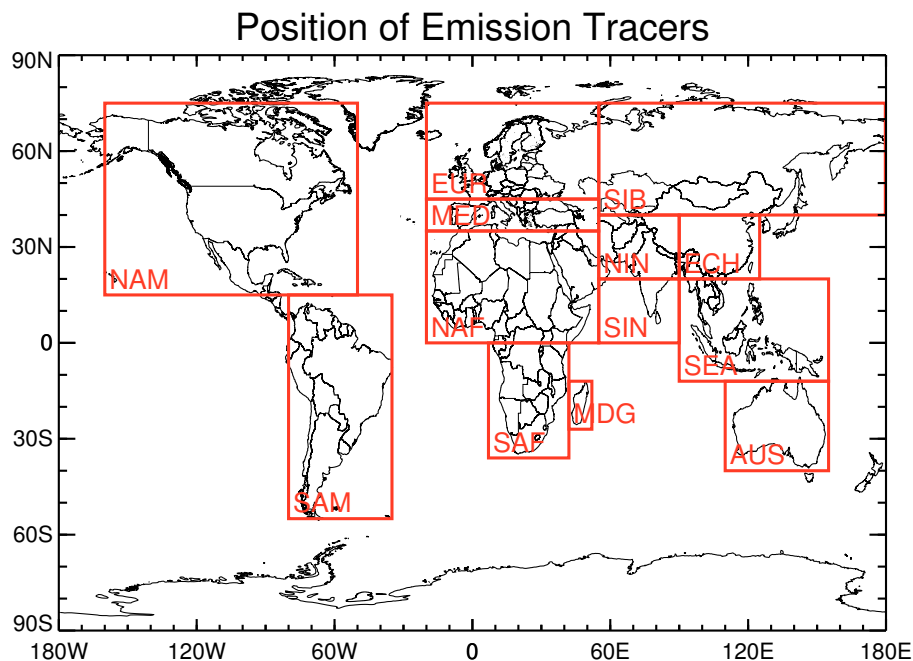
Figure 1. Global geographic position of artificial boundary layer source regions in the CLaMS model, also referred to as “emission tracers”. The latitude and longitude range for each emission tracer is listed in Table 1.
