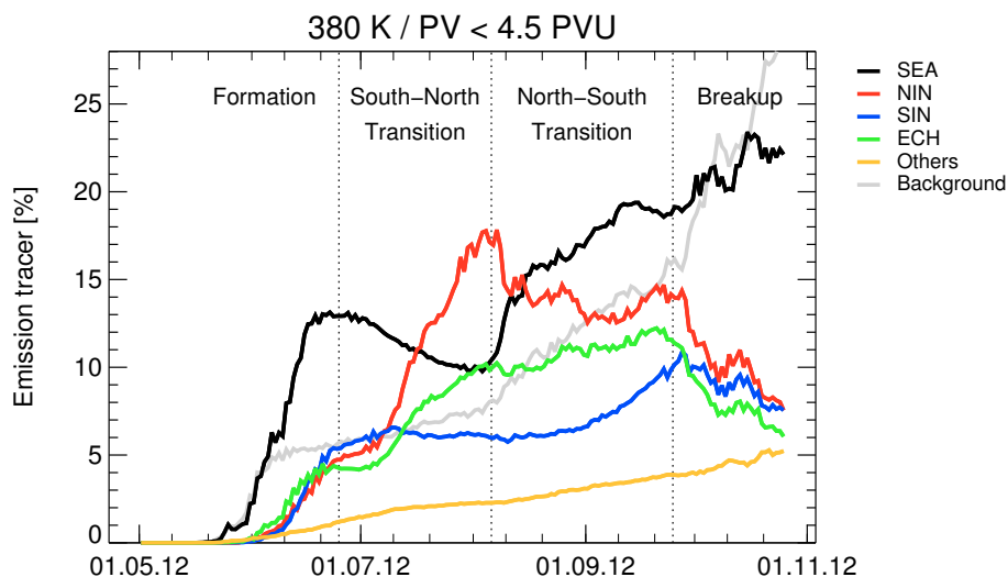
Figure 8. Temporal evolution of different emissions tracers from Southeast Asia (SEA, black), North India (NIN, red), South India (SIN, blue), East China (ECH, green), and from all other land masses (others, yellow) within the Asian monsoon anticyclone at 380 K from May 2012 until end of October 2012. Contributions of boundary sources not considered in the defined emissions tracers listed in Table 1 are summarised as background (grey). The shown percentages are mean values calculated for air masses in Asia in the region between 15 and 50° N and 0 and 140° E at 380 \pm 0.5 K (see black box in Fig. 7) with PV values lower than 4.5 PVU that marks the edge of the anticyclone.
