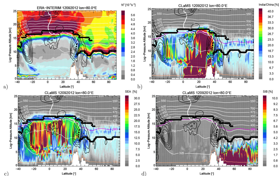
Figure 11. Latitude-height cross-section of the Northern Hemisphere including the Asian Monsoon area ( \approx 15\text{--}35^\circ\text{N} ) at 80^\circ\text{E} longitude of (a) static stability ( N^2 ), (b) the fraction of air originating in India/China (here the sum of North India (NIN), South India (SIN), and East China (ECH)), the fraction of air originating in (c) Southeast Asia (SEA) and in (d) Siberia (SIB). The corresponding levels of potential temperature are marked by thin white lines. The 380 K surface is highlighted in purple to illustrate the position of the horizontal cross-sections shown in Figs. 3 and 7. Further, the thermal tropopause (black dots) and the 4.5 PVU surface (thick white lines) are shown. The wind velocities are shown as black lines. The different emission tracers are initialised 2–3 km above surface following orography indicated by the orange line (corresponding to \zeta lower than 120 K).
