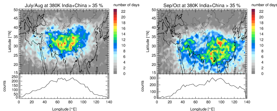
Figure 6. The number of days ( N(\lambda, \phi) ) (top panel) calculated in latitude-longitude bins (of 2.5^\circ longitude \times 1.0^\circ latitude) at 380 K ( \pm 1 K) with mean values of the contributions of emission tracers for India/China larger than 35 % for July/August (left) and September/October (right) 2012. The longitudinal dependence (bottom panel) of the occurrence of days with contributions of emission tracers for India/China larger than 35 % (here “counts” is the number of days summarised over all latitude bins for one longitude bin: \text{counts}(\phi) = \sum_{\lambda=15^\circ}^{\lambda=50^\circ} N(\lambda, \phi) ).
