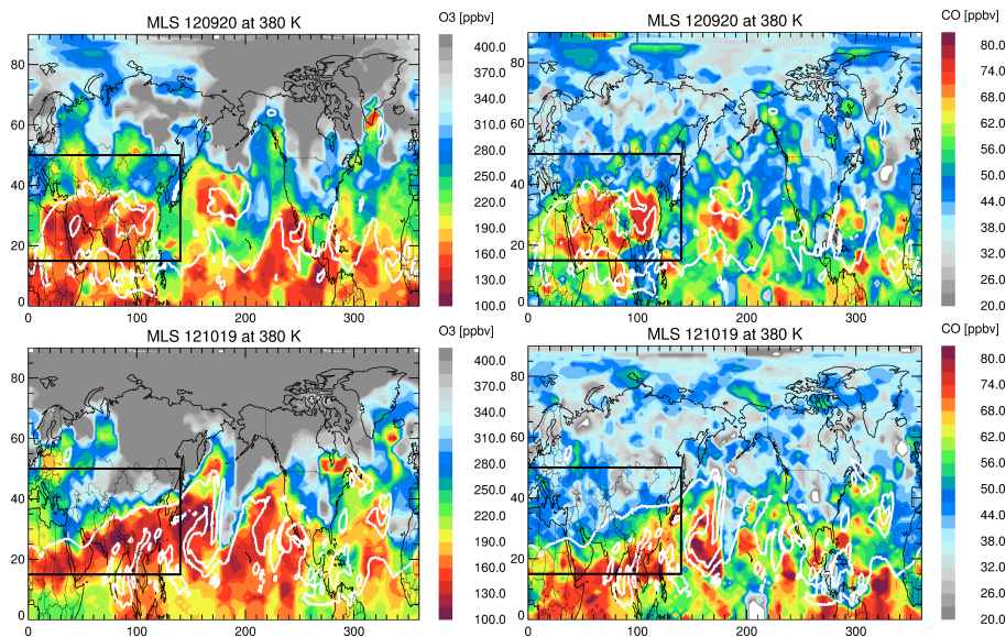
Figure 5. The same as Fig. 4, but on 20 September 2012 (top) and on 19 October 2012 (bottom). Here for simplification, the abscissa is for the longitude range from 0 to 360° to highlight the distribution of O 3 and CO during the eddy shedding event on 20 September 2012 (top) and after the breakup of the anticyclone on 19 October 2012 (bottom).
