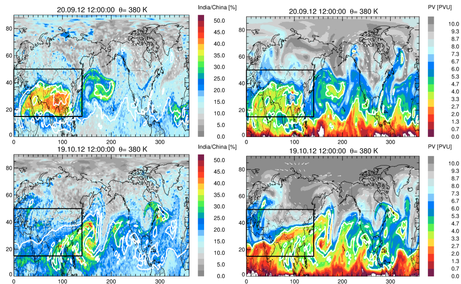
Figure 3. The same as Fig. 2, but on 20 September 2012 (top) and on 19 October 2012 (bottom). Here for simplification, the abscissa is for the longitude range from 0 to 360° to highlight the eddy shedding event on 20 September 2012 (top) and the distribution of emission tracers for India/China after the breakup of the anticyclone on 19 October 2012 (bottom).
