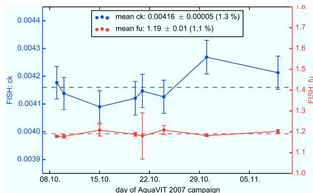
Figure 7. Time series for the calibration constants c_k and f_u during the AquaVIT-1 campaign evaluated with the enhanced calibration scheme.
