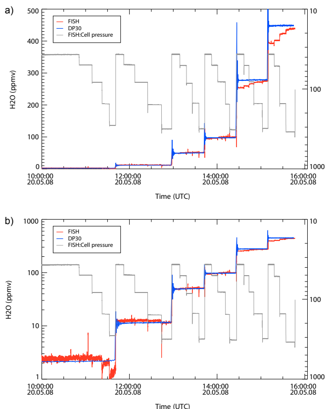
Figure 4. FISH and DP30 WVMR time series measured with the Jülich calibration bench with a flow rate of 5 standard L min -1 : (a) linear scale; (b) logarithmic scale.
