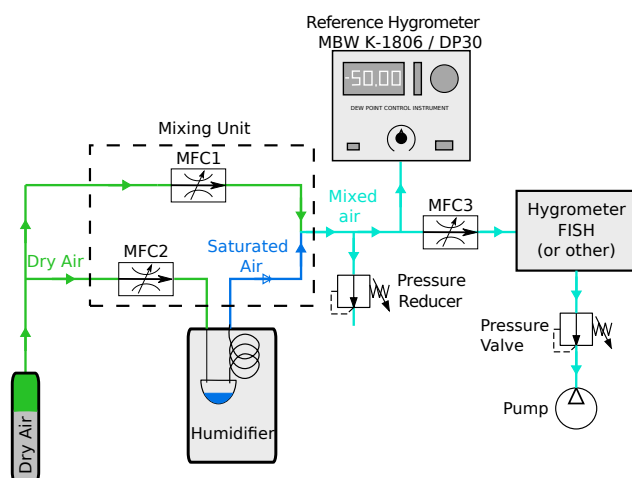
Figure 3. This diagram illustrates the principal setup of the Jülich calibration bench. The colored paths (green, dark and light blue) indicate the air flow through the system. Green and dark blue represent the flow of dry and water saturated air, respectively. The user-defined, stable humidity level generated by mixing the dry and saturated air is colored in light blue.
