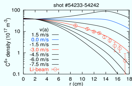
Fig.2) High ion temperatures: IONEQ calculations with convection velocity v(a) as parameter and data from Li-beam CX.
