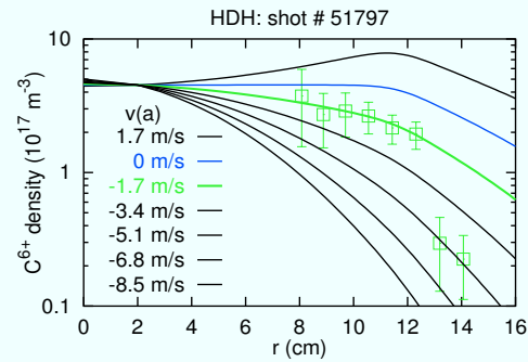
Fig.6) HDH-mode: IONEQ calculations with v(a) as parameter and measured data from Li-beam CX.
