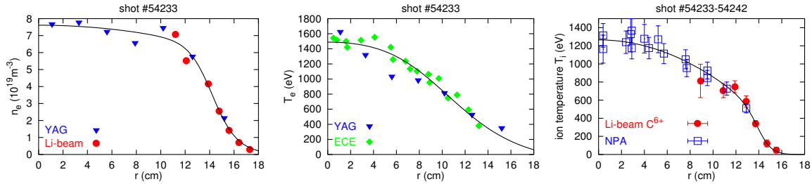
Fig.2) High ion temperatures: IONEQ calculations with convection velocity v(a) as parameter and data from Li-beam CX.
