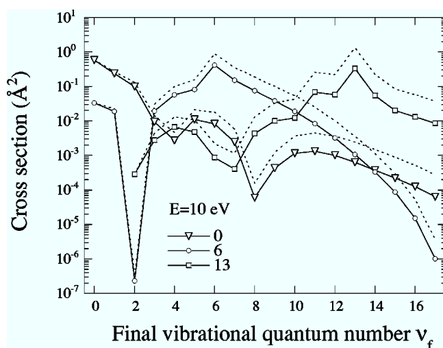
FIG. 10. State-to-state cross sections for process \text{H}_2(c^3\Pi_u, \nu_i) + e \rightarrow \text{H}_2(g^3\Sigma_g^+, \nu_f) + e (solid lines) as a function of final vibrational quantum number, at the incident energy E=10 eV, for \nu_i=0, 6 , and 13 , compared with corresponding structural factors [Eq. (2)] (dashed lines) normalized to the first \nu_f cross-section value.
