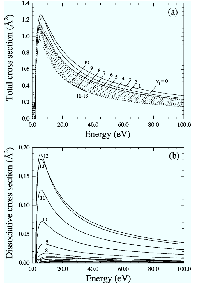
FIG. 5. Cross sections as a function of energy for the processes (a) \text{H}_2(c^3\Pi_u, \nu_i = 0-13) + e \rightarrow \text{H}_2(g^3\Sigma_g^+) + e ; (b) \text{H}_2(c^3\Pi_u, \nu_i = 0-13) + e \rightarrow \text{H}_2(g^3\Sigma_g^+) + e \rightarrow \text{H} + \text{H} + e .
