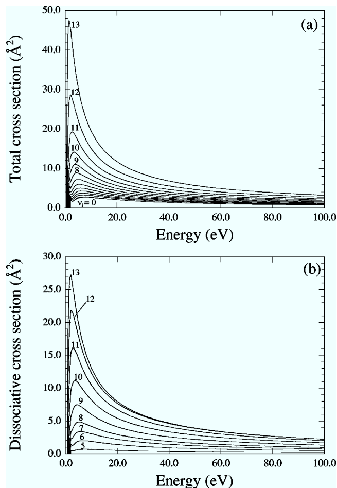
FIG. 7. Cross sections as a function of energy for the processes (a) \text{H}_2(c^3\Pi_u, \nu_i = 0 - 13) + e \rightarrow \text{H}_2(h^3\Sigma_g^+) + e ; (b) \text{H}_2(c^3\Pi_u, \nu_i = 0 - 13) + e \rightarrow \text{H}_2(h^3\Sigma_g^+) + e \rightarrow \text{H} + \text{H} + e .
