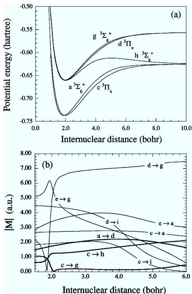
FIG. 1. (a) Schematic energy diagram for triplet states of H_2 molecule; (b) transition dipole moment as a function of internuclear distance for some triplet-triplet transitions (thick lines indicate the transitions considered in this paper).
