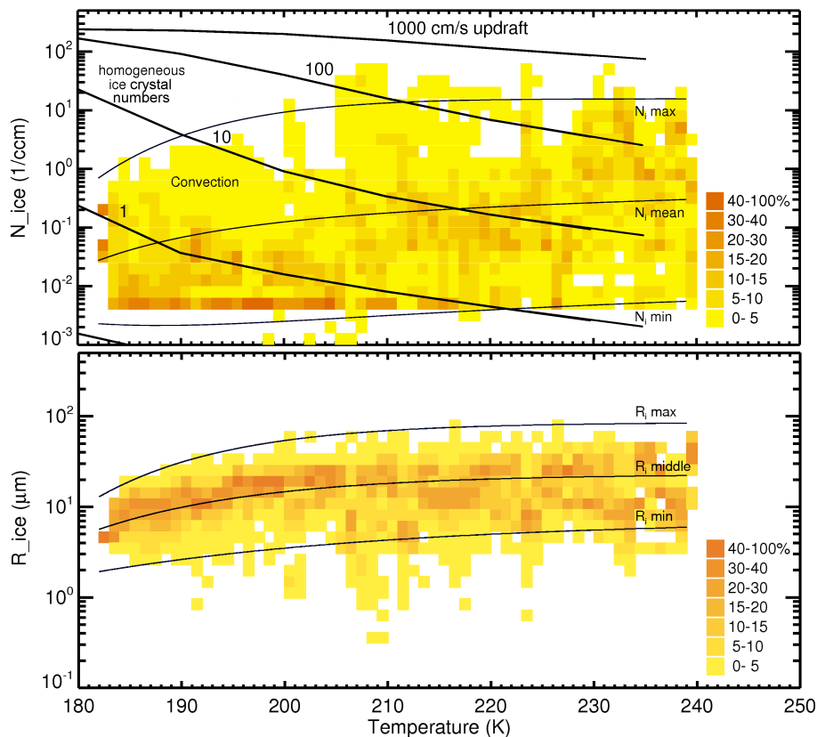
Fig. 9. Frequencies of occurrence of ice crystal numbers N_{\text{ice}} (top panel) and sizes R_{\text{ice}} (bottom panel) vs. temperature (same dataset as Fig. 5; thin solid lines: minimum, middle and maximum N_{\text{ice}} and R_{\text{ice}} ; thick solid lines in top panel: ice crystal numbers arising for homogeneous freezing at different updraft velocities after Koop et al. (2000) for an aerosol particle number of 300 \text{ cm}^{-3} and mean pressure; data are sorted in 1 K temperature bins).
