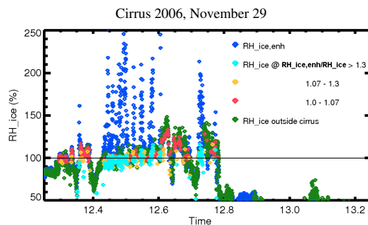
Fig. 2. \text{RH}_{\text{ice}} and \text{RH}_{\text{ice,enh}} in the course of the flight Cirrus 2006, November 29, colour coded for “cirrus-parameter” \text{RH}_{\text{ice,enh}}/\text{RH}_{\text{ice}} to define in/out cirrus (inside cirrus: confident , less confident , uncertain ; outside cirrus ).
