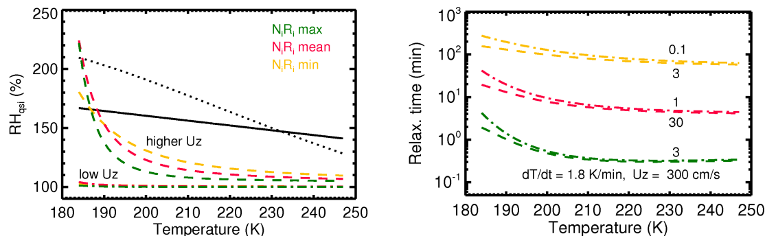
Fig. 6. Quasi steady state RH_{\text{ansi}} (left) and relaxation times \tau (right) vs. temperature for minimum (yellow), middle (red) and maximum (green) N_i R_i and a high (dashed)/low (dashed-dotted) vertical velocity u_z , respectively ( N_i R_i = N_{\text{ice}} \cdot \overline{R_{\text{ice}}} , calculated from the lines in Fig. 5 with p = p_{\text{mean}}(T) taken from Schiller et al. (2008), electronic supplement; the black dotted line represents water saturation, the black solid line the homogeneous freezing threshold after Koop et al. (2000); note that the calculations are not for evaporating cirrus, where u_z is negative and RH_{\text{ice}} is below saturation); for more information see text.
