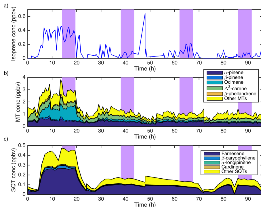
Figure 3. Isoprene (a), monoterpene (b), and sesquiterpene (c) concentrations measured from the outlet air of the JPAC plant chamber. In (b) and (c) we left out those terpenes that had a negligible contribution to the total terpene concentration. Purple bars indicate UV on periods during the measurements.
