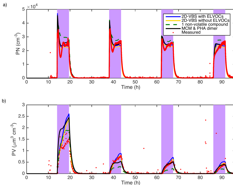
Figure 8. Modelled and measured (a) total particle number concentration and (b) total particle volume concentration. The model results are from simulations with the 2-D VBS and with or without ELVOC formation via ozonolysis and OH-oxidation of monoterpenes and sesquiterpenes (Reactions R1 and R2), from a simulation when the MCM compounds were used as the condensable organic compounds and considering PHA dimer formation with Eq. (7), and from a simulation with only one condensable non-volatile compound. The mass yield of the non-volatile compound formed from O_3 and OH oxidation of all monoterpenes and sesquiterpenes was 60 %.
