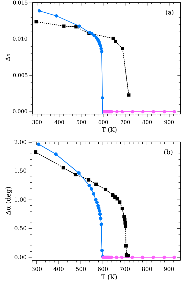
FIG. 4. (Color online) Temperature variations of (a) distortion parameter \Delta x and (b) deviation \Delta \alpha of the distortion angle from 90^\circ . The present NPD data (circles) are compared to the neutron-diffraction experiments performed on single crystals (squares) by Chattopadhyay et al. [8]. The continuous lines are just guides to the eye.
