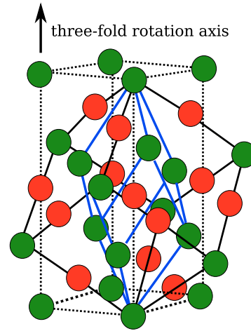
FIG. 1. (Color online) Structure of the low-temperature phase of GeTe (space group R\bar{3}m ) shown in the pseudocubic (thick black lines), hexagonal (dotted lines), and rhombohedral (thick blue/gray lines) representations.
