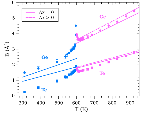
FIG. 8. (Color online) Experimental (symbols) and theoretical (lines) isotropic temperature factors B determined for Ge (circles) and Te (squares) atoms in the rhombohedral and cubic phases of GeTe. The solid lines denote calculated B factors for the rhombohedral and ideal cubic GeTe structures. Dashed lines correspond to calculated B factors for the cubic GeTe structure with static distortion \Delta x = 14.56 \times 10^{-3} ( s = 2.84 \text{ \AA} , l = 3.19 \text{ \AA} ). Calculations are performed within the harmonic approximation. Theoretical isotropic temperature factors are evaluated as B = 8\pi^2 \langle U \rangle , where \langle U \rangle is the trace of the U_{ij} tensor [20].
