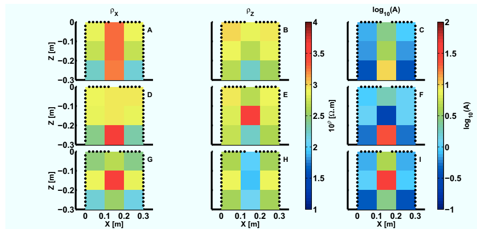
Figure 4.4: ERT inversion results for \rho_X (panel A, D, and G), \rho_Z (panel B, E, and H), and \log_{10}(A) (panel C, F, and I) for Stage I (panel A, B, and C), Stage II (panel D, E, and F), and Stage III (panel G, H, and I) for mesh9.
