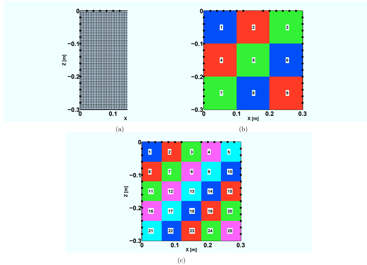
Figure 4.2: (a) Discretization used for ERT forward modelling, and discretization used for ERT inversion: mesh9 (b) and mesh25 (c). All elements have been numbered for proper identification. The position of all electrodes is indicated with solid black circles.
