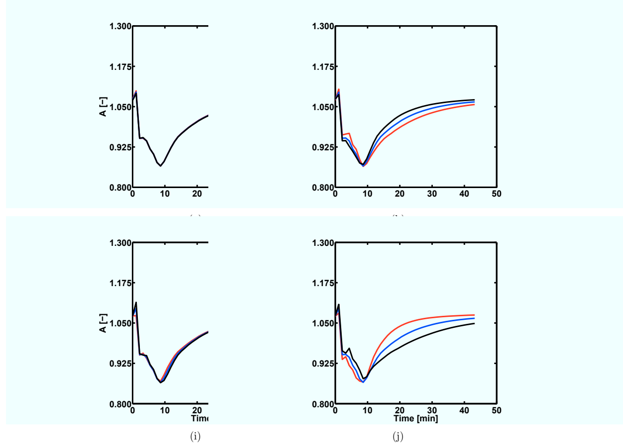
Figure 3.7: Sensitivity analysis of the anisotropy to changes in the hydraulic properties by increasing (black) and decreasing (red) 10 % of the following parameters: (a) \alpha , (c) K_s , (e) n , (g) \theta_r , and (i) \theta_s of the macropore domain and (b) \alpha , (d) K_s , (f) n , (h) \theta_r , and (j) \theta_s of the matrix domain. Blue lines correspond with the original hydraulic parameters provided in Table 3.1. The n parameter of the macropore domain (e) could not be increased by 10 % because of numerical issues with the HYDRUS model.
