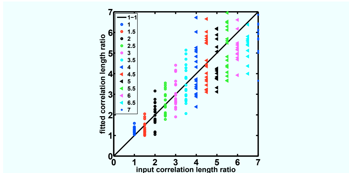
Figure 2.10: Scatter plot of the prescribed and fitted correlation length ratio obtained by inversion of the effective complex electrical resistivity in two directions by minimizing Equation 2.14 for 247 distributions with varying Cole-Cole parameters, volume fraction, and the correlation length ratio for material A and B.
