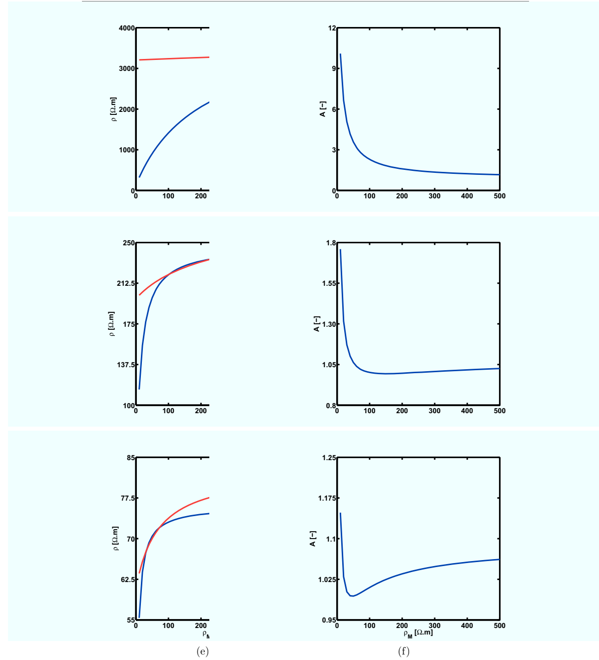
Figure 3.4: Simulated horizontal (red) and vertical (blue) resistivity (a, c, and e) and the associated anisotropy (b, d, and f) from (a and b) dry ( \rho = 3800 \Omega.m ), (c and d) moist ( \rho = 250 \Omega.m ), and (e and f) fully saturated ( \rho = 72 \Omega.m ) matrix domain as a function of the macropore resistivity for a macropore volume fraction of 0.05 \text{ cm}^3 \text{ cm}^{-3} . \rho_M indicates the resistivity of the macropore domain.
