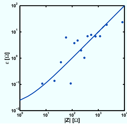
Figure 4.3: Binning of the symmetrical measurement configurations into 15 equally sized bins (dots) in logarithmic scale and the fitted error model (line).
