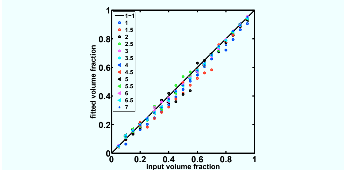
Figure 2.11: Scatter plot of the prescribed and fitted volume fraction obtained by inversion of the effective complex electrical resistivity in two directions by minimizing Equation 2.14 for 247 distributions with varying Cole-Cole parameters, volume fraction, and the correlation length ratio for material A and B.
