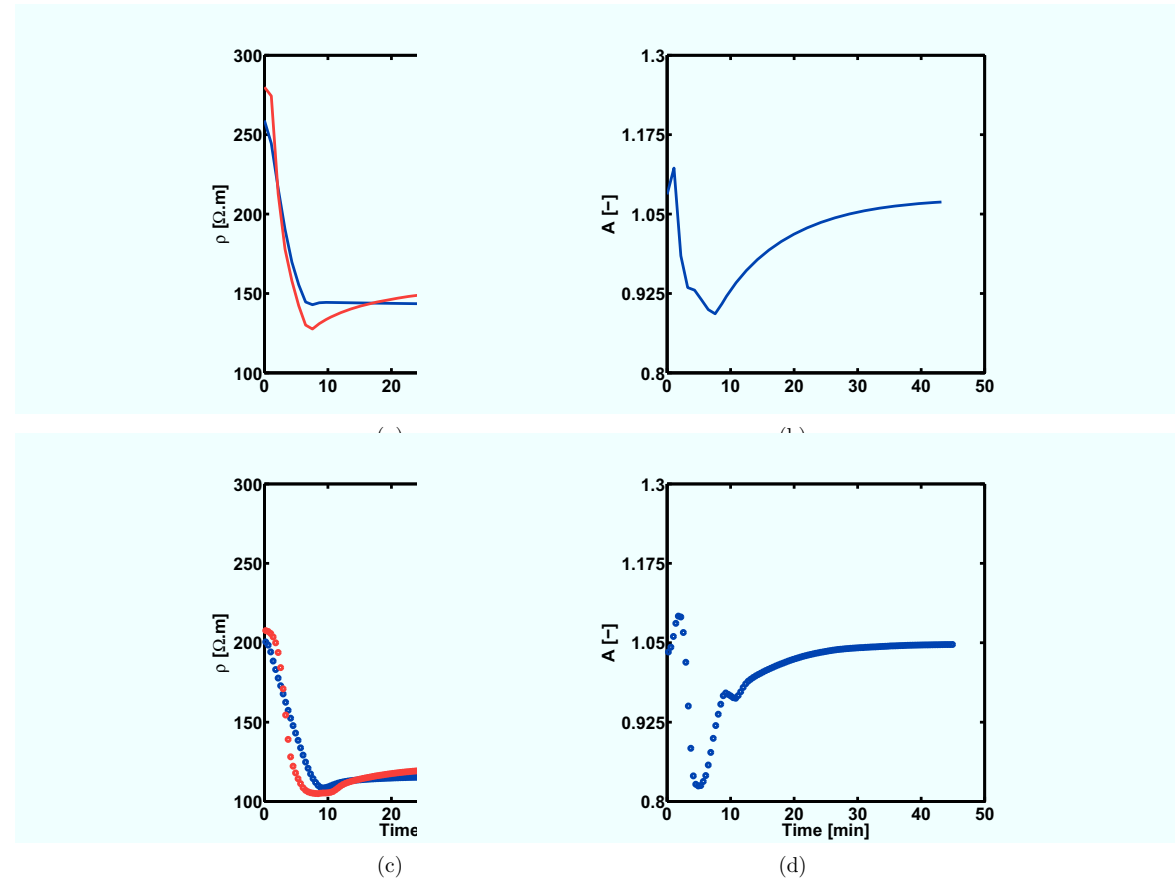
Figure 3.6: Horizontal (red) and vertical (blue) electrical resistivity (a and c) and the associated anisotropy (b and d) from (a and b) simulations and (c and d) measurements of water infiltration in an artificial macropore.
