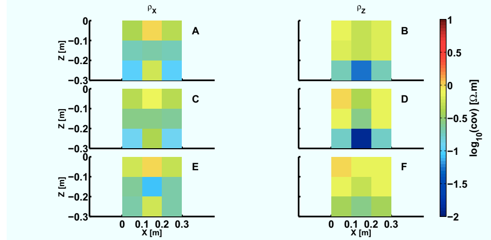
Figure 4.5: Cumulative sensitivity coverage for Stage I (panel A and B), Stage II (panel C and D), and Stage III (panel E and F) for \rho_X (left) and \rho_Z (right) for mesh9.
