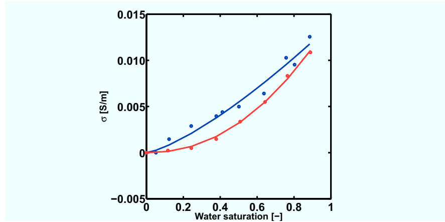
Figure 3.2: Electrical conductivity measurements made with TDR (dots) on soil sample cores and the fitted Archie's model (lines) for sand-clay (blue) mixture and sand (red) material.
