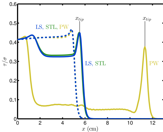
Figure 5 | The frictional stress is prior to the first event (dashed lines) and is after (solid lines). The color code is as in Fig. 1. It is seen that the stress left at the tail of the rupture fronts, \tau_r , is roughly homogeneous in space, and that it is much lower in the PW model than in the LS and STL models. The location of the fronts after the event is marked by x_{tip} . The deeper penetration of the PW model, also shown in Fig. 4, is clearly visible.
