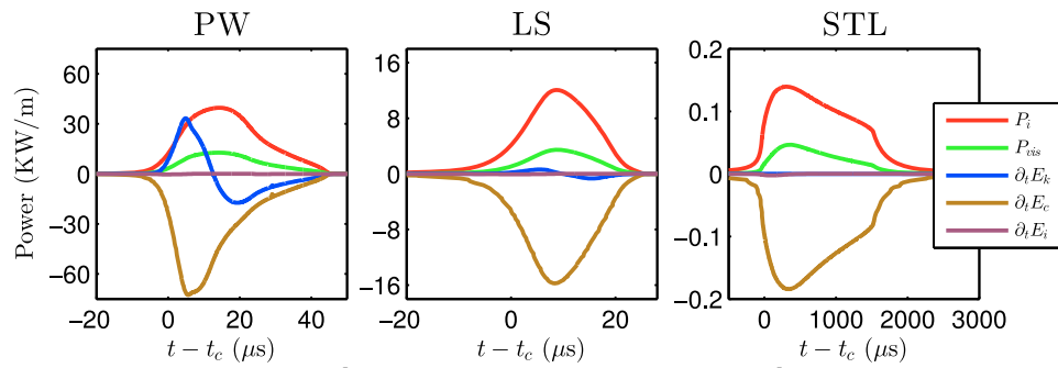
Figure 6 | The rate of change of energies \partial_t E_\gamma(t) = \partial_t \int_0^L \varepsilon_\gamma(x, t) dx and dissipation rates P_\gamma(t) = \int_0^L p_\gamma(x, t) dx ( \varepsilon_\gamma(x, t) and p_\gamma(x, t) are defined in Eqs. (21)) during the first event for the three models.
