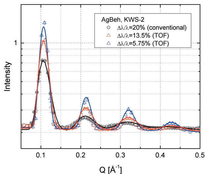
Figure 10 SANS data of the AgBeh reference sample measured at KWS-2 in conventional (black) and TOF (red and blue) modes for different \Delta \lambda/\lambda_{\text{aim}} . Only data recorded in the central TOF channel are shown.
