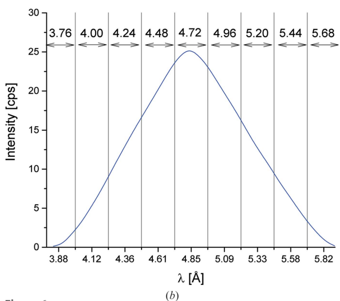
Figure 6 Measured direct beam intensity on the detector ( L_D = 1.3 m) for \lambda = 4.72 Å as a function of TOF ( a ) and of recalculated wavelength ( b ) according to the measured TOF and experimental settings corresponding to \Delta\lambda/\lambda_{\text{aim}} = 5\% ; the real \Delta\lambda/\lambda calculated from the measured t and \Delta t corresponding to each time slot is indicated in ( a ); the mean wavelength of each slot is indicated in ( b ), as defined by the left flank of the slot, according to the scheme shown in Fig. 5( b ).
