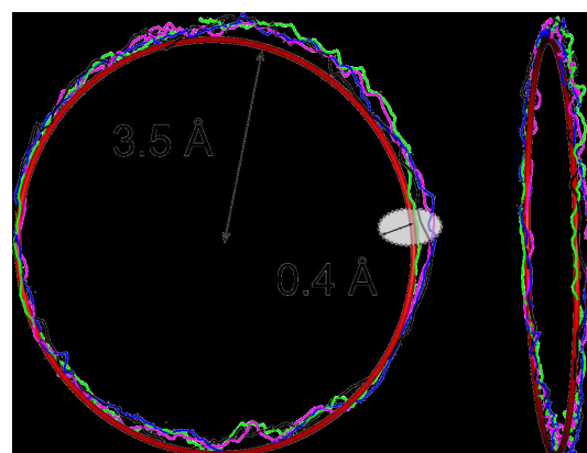
Figure 3: Precision of an arbitrary trajectory tracking in HCM with the visual feedback. The operator followed a circle with HCM for four times. Each attempt took one minute and the maximum deviation from the cycle was approx. 0.4 \text{ \AA} . Further details in text.
