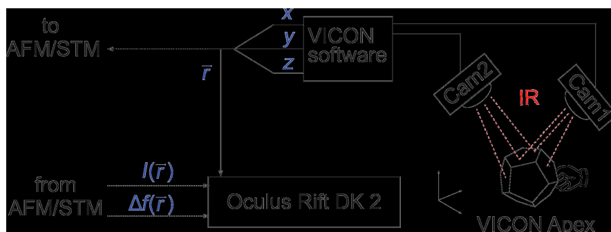
Figure 2: Scheme of the set-up used for HCM with a visual feedback using Oculus Rift virtual reality goggles (ORT). VICON 3D tracking system with two IR cameras follows the position of the VICON Apex device. VICON Apex has a dodecahedral shape, on the surface of which multiple sources of IR light are installed. The emitted IR light is registered by the cameras that compose an image from which the VICON software reconstructs the position and the orientation (not used in the experiment) of the Apex device in 3D space. The obtained coordinates x, y, z are used to set the position of the AFM/STM tip. The same coordinates are used to plot 3D trajectories in the virtual space of (ORT).
