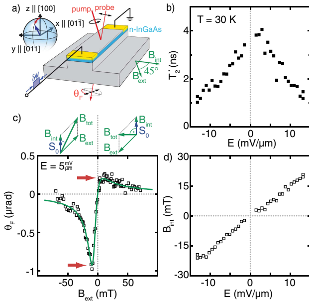
FIG. 1 (color online). (a) Schematic setup. dc or pulsed E fields are applied along the [01\bar{1}] direction of an n -InGaAs transport channel. Electrically or optically generated spins are probed by static and TRFR in polar geometry. (b) T_2^* vs dc E field. (c) (upper panel) Schematics of total effective magnetic field \mathbf{B}_{\text{tot}} for positive and negative B_{\text{ext}} . (lower panel) Asymmetric Hanle curve taken at E = +5 \frac{\text{mV}}{\mu\text{m}} and T = 30 \text{ K} . The green line is a fit to Eq. (1). (d) B_{\text{int}} determined from asymmetric Hanle signal vs dc E field.
