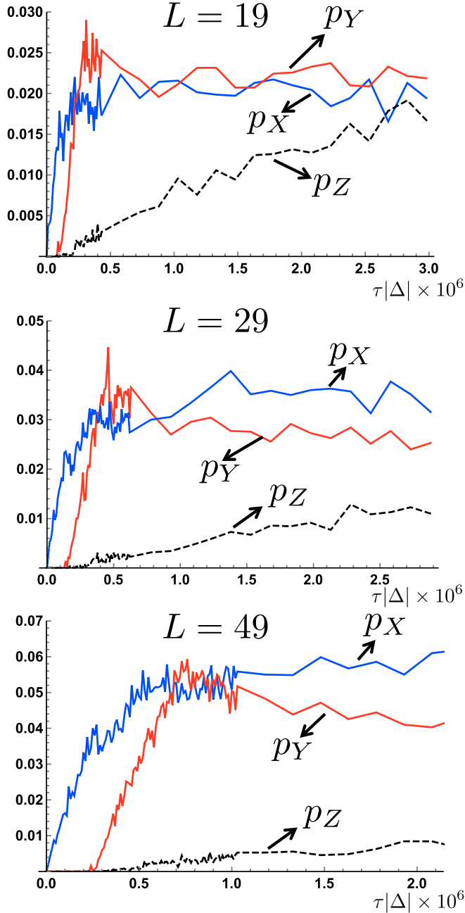
FIG. 16. (Color online) Plots of p_X , p_Y , and p_Z as function of time. MBSs 1 and 3 are exchanged while MBSs 2 and 4 remain immobile [see Fig. 7(b)]. The time to braid is proportional to the size of the trijunction and we have \tau_{\text{braid}} = (2L + 2)10^4/|\Delta| . For \tau < \tau_{\text{braid}} , i.e., when the exchange is not finished, we exchange the MBSs until time \tau with the coupling to the thermal bath being on. Then, we unitarily (no coupling to the thermal bath) finish the braid and perform error correction at the end. Here, we use \kappa = 2 \times 10^{-4}|\Delta| and \beta = 4/|\Delta| .
