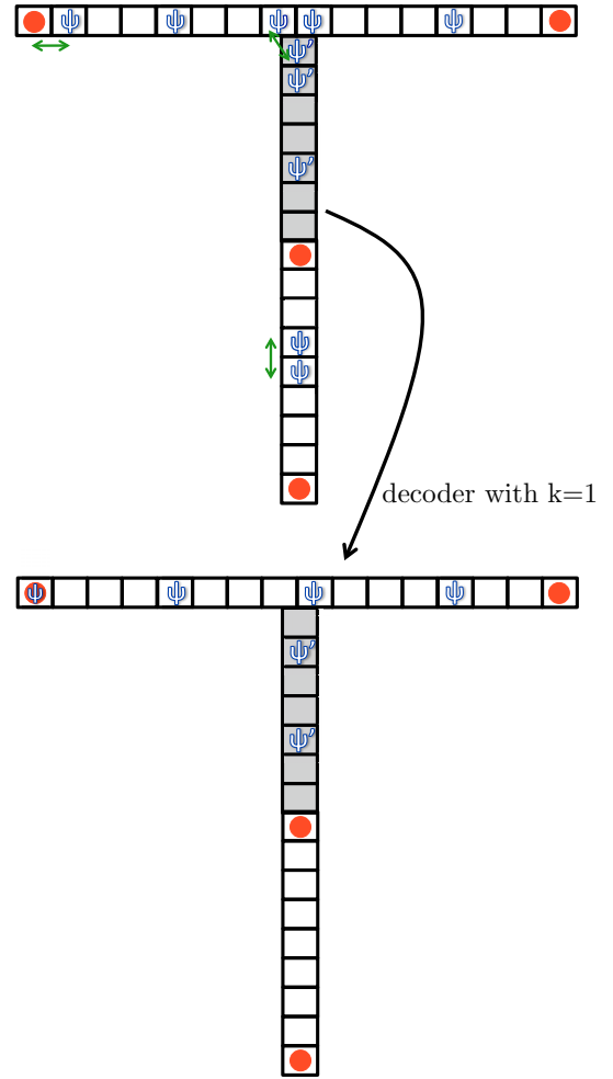
FIG. 14. (Color online) First iteration ( k = 1 ) of the greedy decoder used in our trijunction simulations. After having identified the pairs of excitations at distance k , we annihilate them according to the protocol described in Sec. VI. Our algorithm is a straightforward adaptation of the one presented in Ref. [50].
