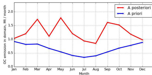
Figure 10. Monthly emissions of OC in Asia, total 2008, unit = \text{Mt PM month}^{-1} . Annual average OC mass: a priori: 7.8 \times 10^9 kg; a posteriori: 1.5 \times 10^{10} kg.
