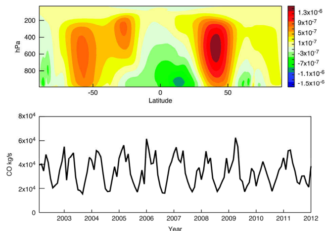
Figure 2. Cross section at 180^\circ \text{E} of the average zonal CO flux ( \text{kg m}^{-2} \text{s}^{-1} ) in the 2003–2012 period calculated from the CO, U and density fields of the MACC re-analysis (top). Time series of monthly mean CO ( \text{kg s}^{-1} ) transported over the northern Pacific through a pane at 180^\circ \text{E} ( 30\text{--}70^\circ \text{N} , up to 300 hPa) (bottom).
